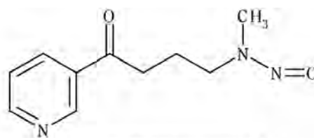
4-(methylnitrosamino)-1-(3-pyridyl)-1-butanone
