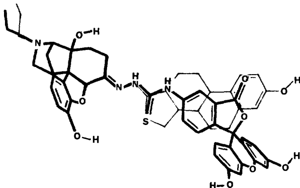
FIGURE 4. NAL-F (dark) and NAL-E superimposed at the naloxone fragment. The polar thiosemicarbazone of the former spatially matches the nonpolar steroid of the latter.
