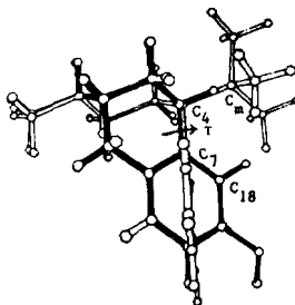
Fig. 1b: Overlap of the optimized phenyl axial conformer of 4- t -butyl-4-( m -OH)-phenyl piperidine with the benzmorphinan ring of morphine.
