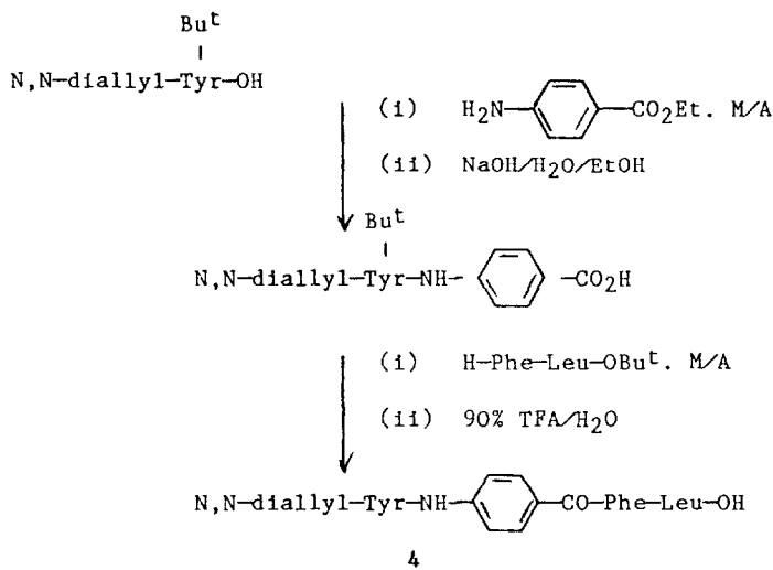
FIGURE 1. Synthetic route
