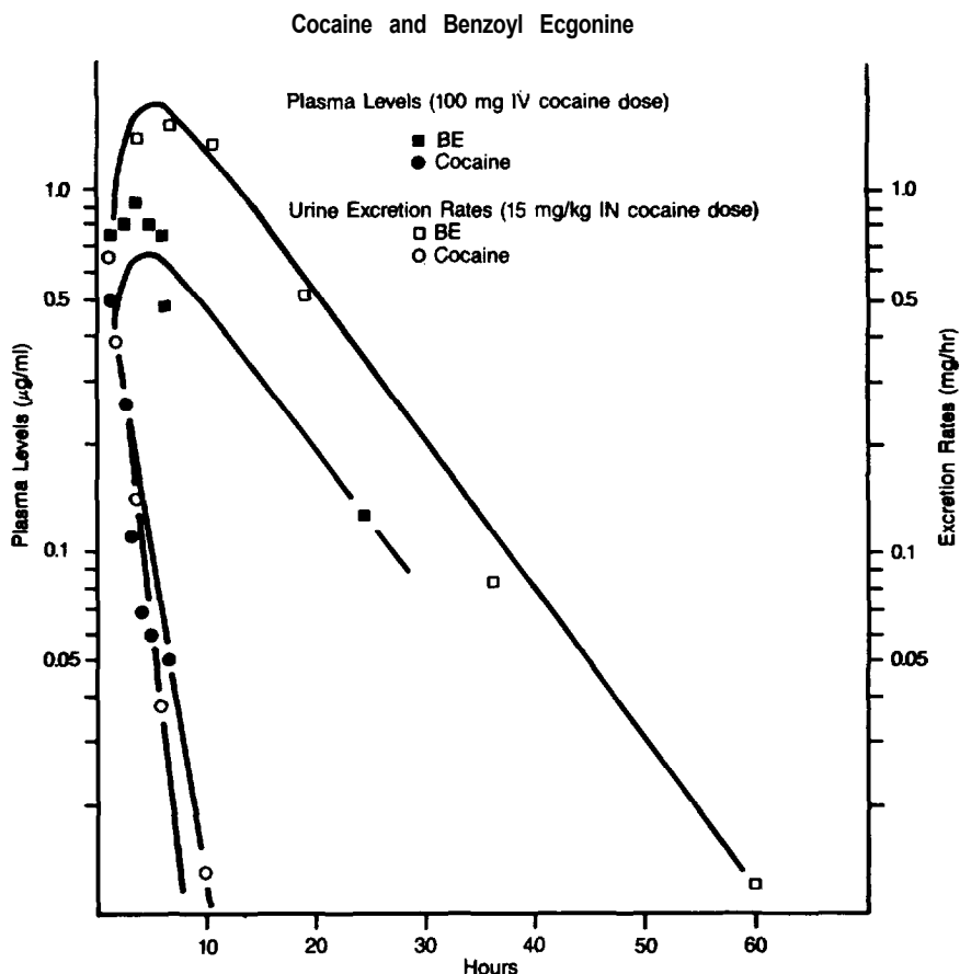
Figure 5. A similar plot of plasma levels and urinary excretion rates of cocaine and benzoylecgonine (From Ambre 1985. Copyright 1985, Preston Publications, Inc.).
