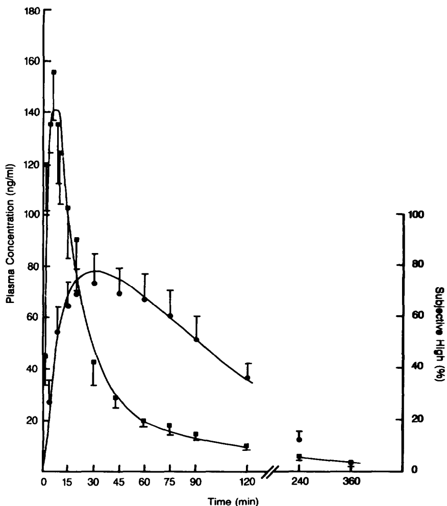
Figure 3. Plasma THC concentration-time (■) and subjective high-time (●) after smoking one 2.5 percent THC cigarette (mean \pm SE; n=6). Solid curves are computer fits to the data (From Chiang and Barnett 1984. Copyright 1984, The C.V. Mosby Co.)
