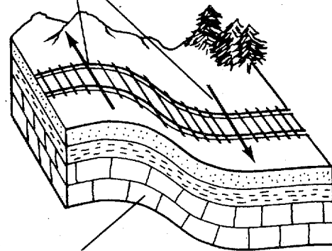
Deformed Rocks
