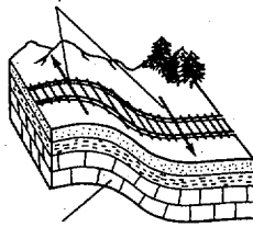
Deformed Rocks
