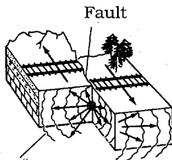
Earthquake Waves
