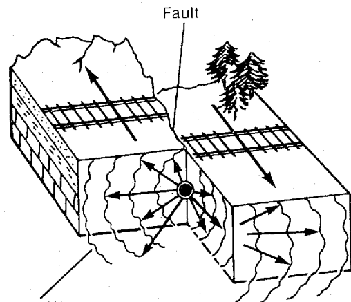
Earthquake Waves
