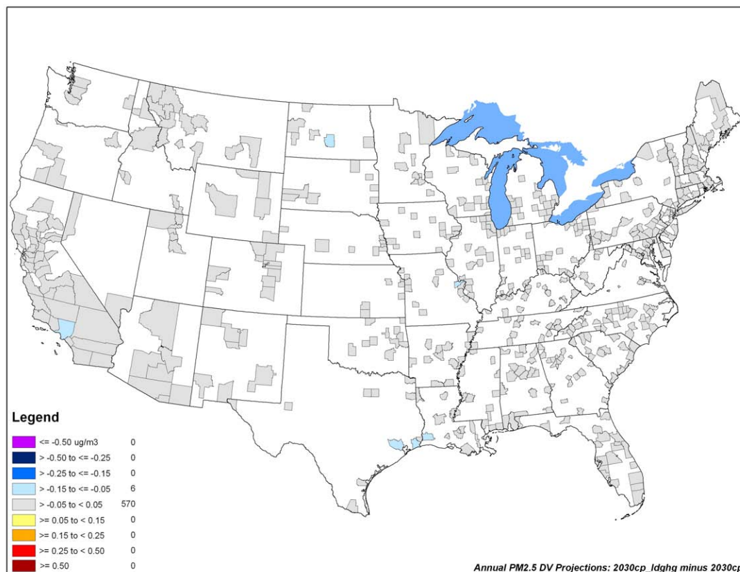
Figure 7-9 Projected Change in 2030 Annual PM 2.5 Design Values Between the Reference Case and Control Case
