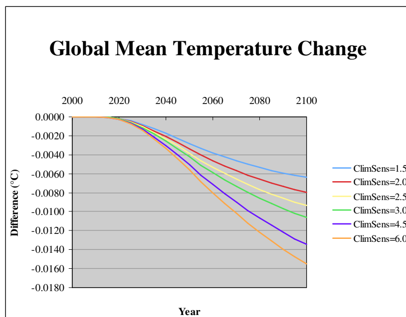
Figure 7-26 Estimated Projected Reductions in Global Mean Surface Temperatures from Baseline for the Final Vehicles Rulemaking (for climate sensitivities ranging from 1.5-6°C)
