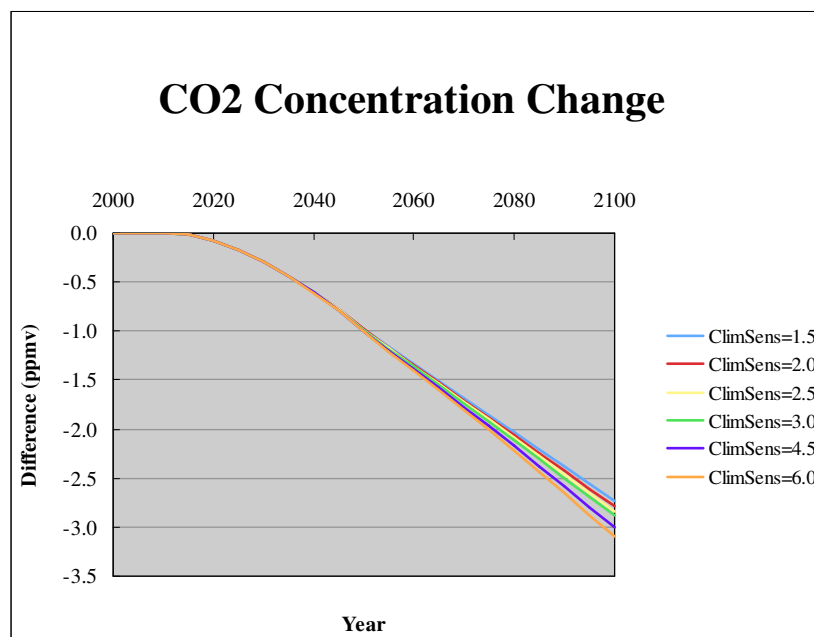
Figure 7-25 Estimated Projected Reductions in Atmospheric CO2 Concentrations (parts per million by volume) from Baseline for the Final Vehicles Rulemaking (for climate sensitivities ranging from 1.5-6°C)
