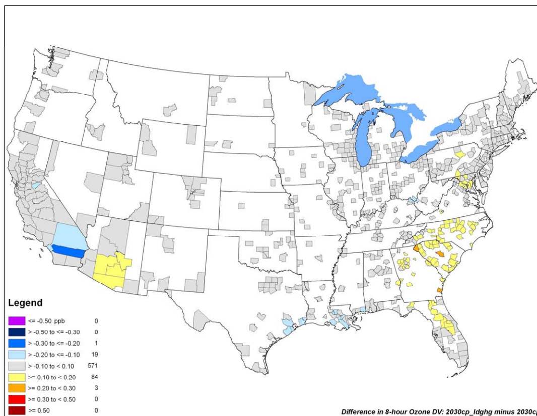
Figure 7-13 Projected Change in 2030 8-hour Ozone Design Values Between the Reference Case and Control Case
