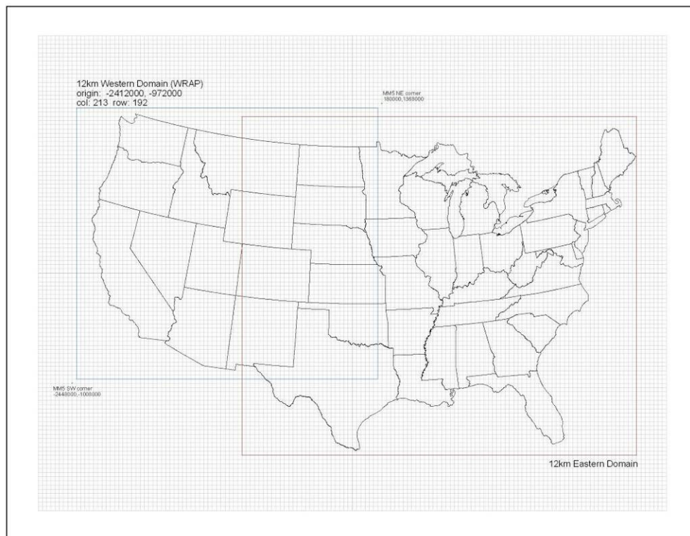
Figure 7-3 Map of the CMAQ Modeling Domain
