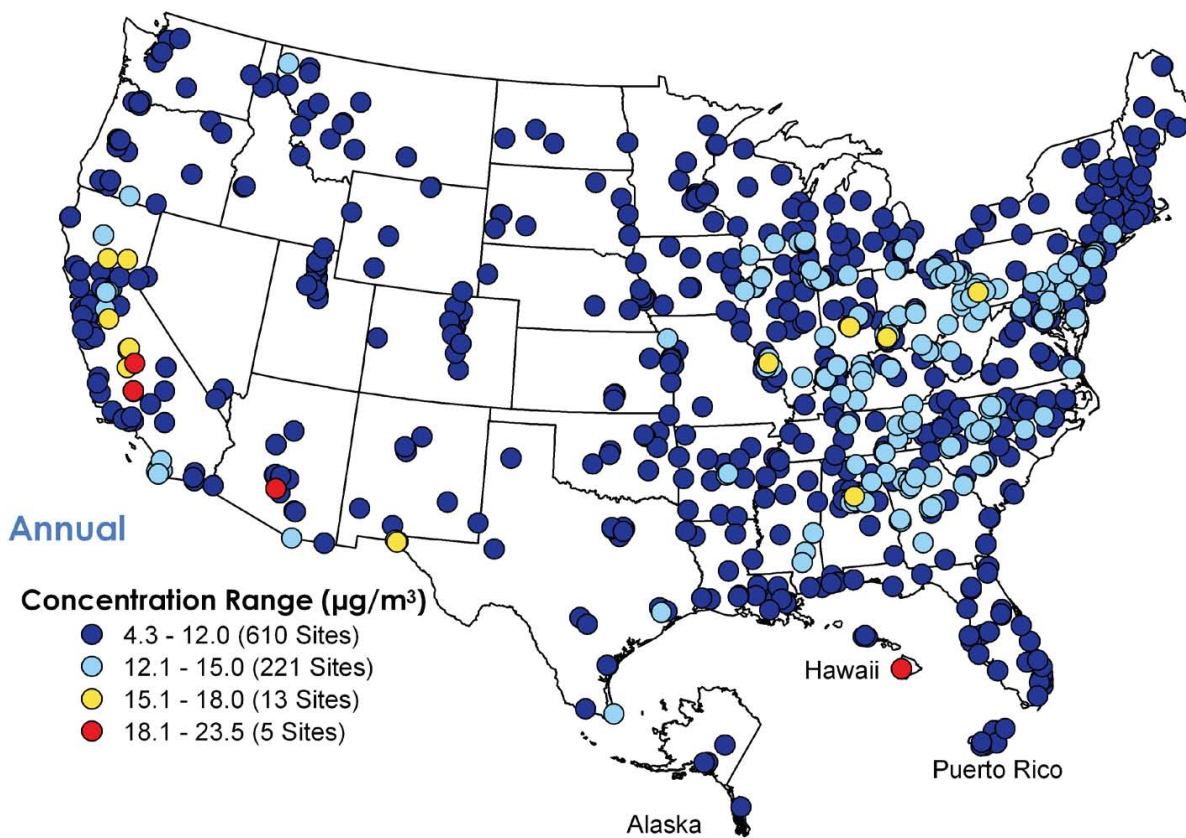
Figure 7-4 Annual Average \text{PM}_{2.5} Concentrations in \mu\text{g}/\text{m}^3 for 2008 x
