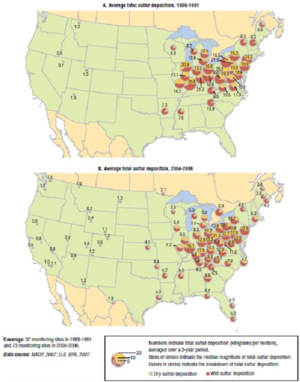
Figure 7-22 Total Sulfur Deposition in the Contiguous U.S., 1989-1991 and 2004 -2006
