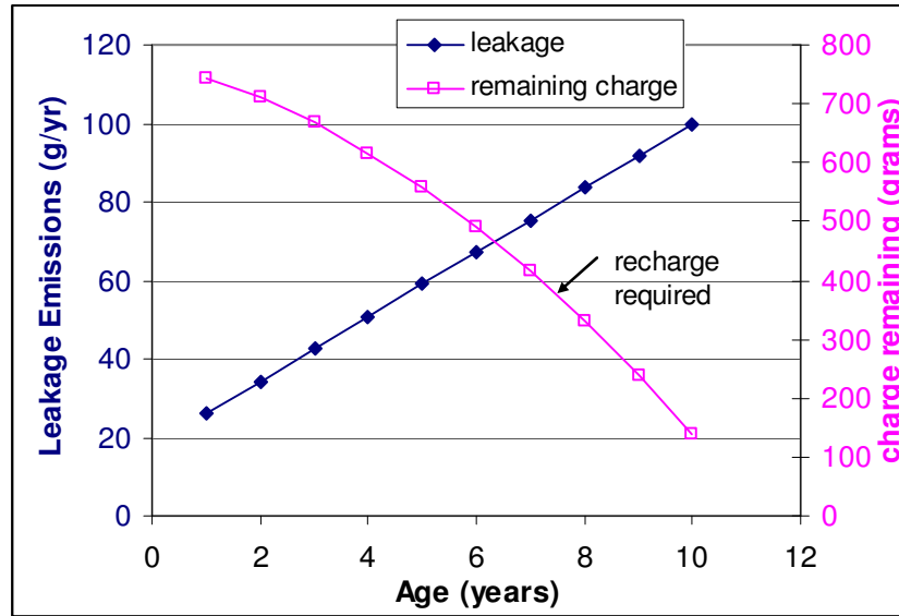
Figure 2-1 Deterioration Rate of Refrigerant Leakage
