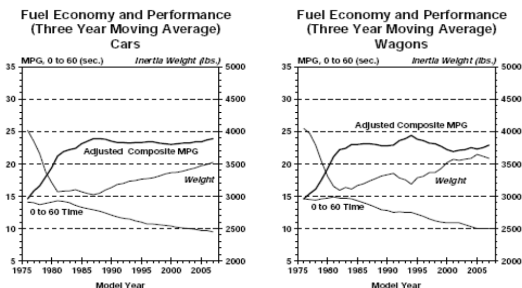
Figure 7-28 Weight, 0-to-60 MPH acceleration time and adjusted fuel economy for light-duty vehicles
