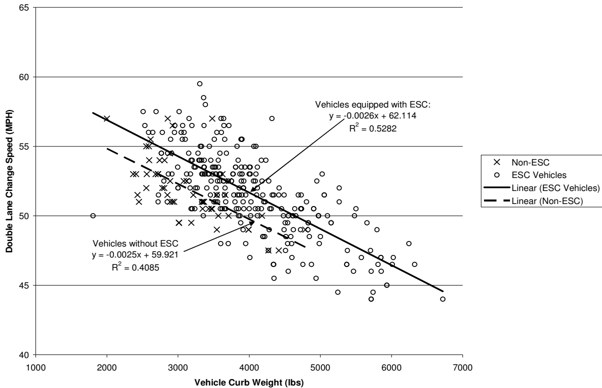
Figure 7-29 Double Lane Change Speed vs. Vehicle Curb Weight
