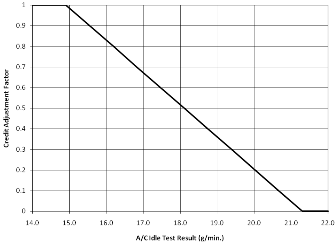
Figure 2-5 A/C Credit Adjustment Factor.
