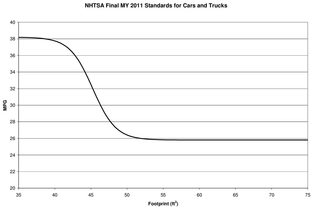
Figure 3-1 NHTSA Reformed CAFE Curve for MY 2011 Cars
