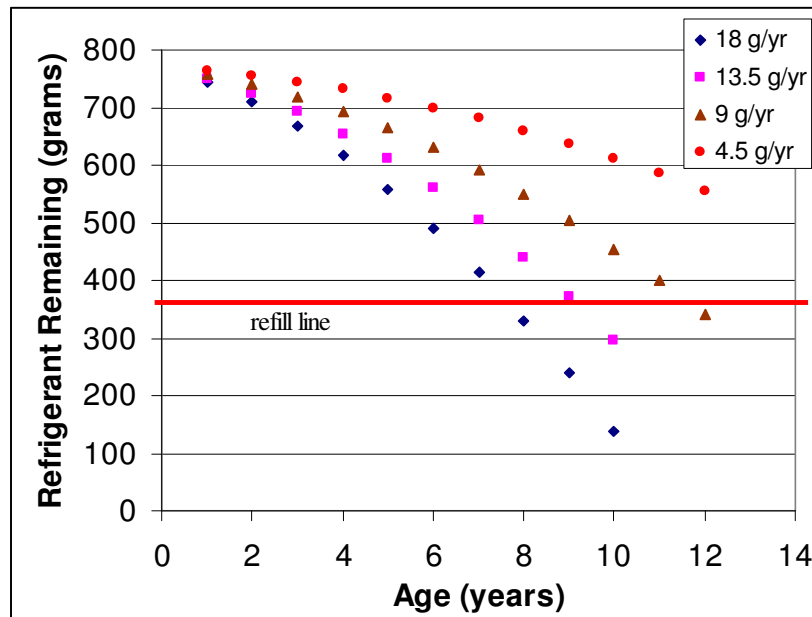
Figure 2-3 A/C Refrigerant Remaining in a Typical System as Vehicles Age and Deteriorate
