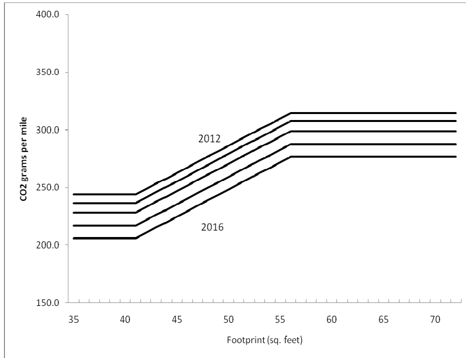
Figure 3-12 CO 2 (g/mi) Car standard curves
