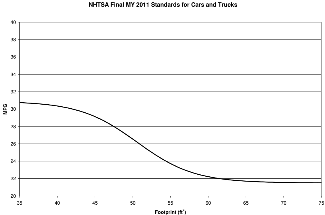
Figure 3-2 NHTSA Reformed CAFE Curve for MY 2011 Trucks
