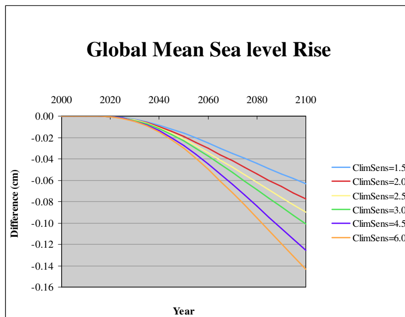
Figure 7-27 Estimated Projected Reductions in Global Mean Sea Level Rise from Baseline for the Final Vehicles Rulemaking (for climate sensitivities ranging from 1.5-6°C)
