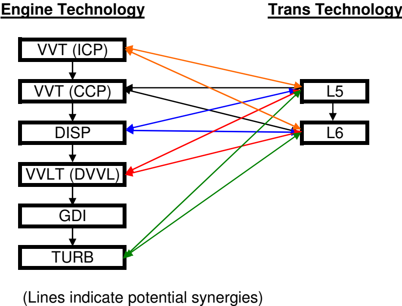
Figure 1-3 Illustration of technology pairings for a specific technology application path
