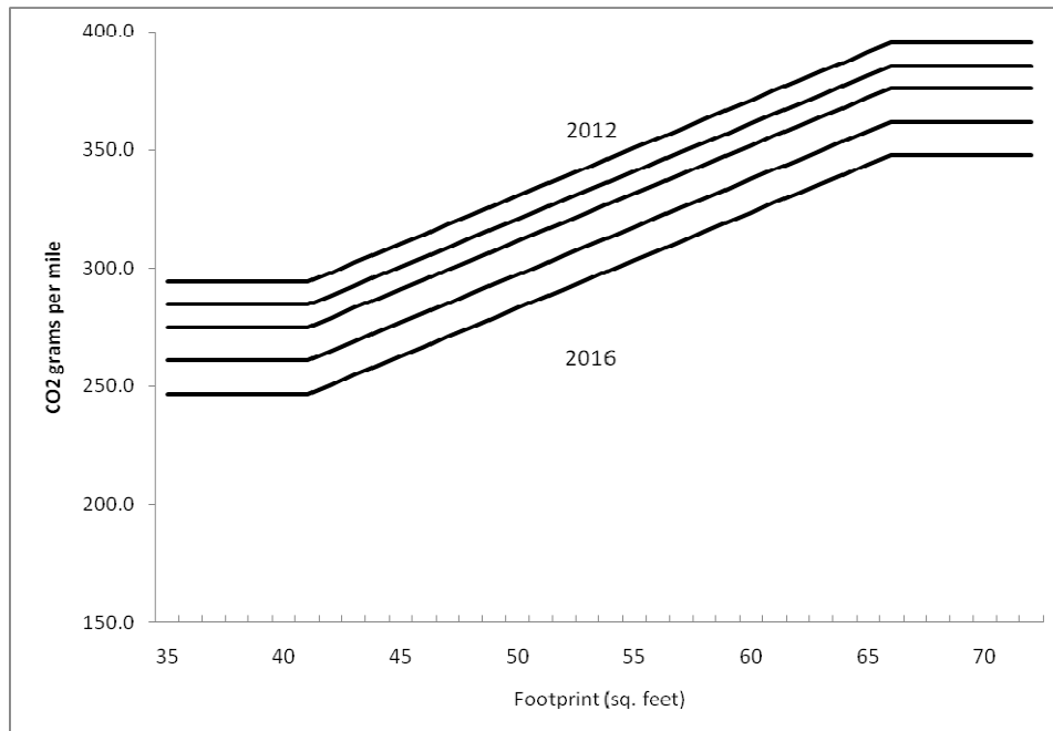
Figure 3-13 CO 2 (g/mi) Truck standard curves
