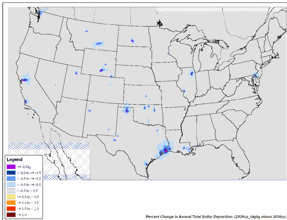
Figure 7-24 Percent Change in Annual Total Sulfur over the U.S. Modeling Domain as a Result of the Required Vehicle Standards
