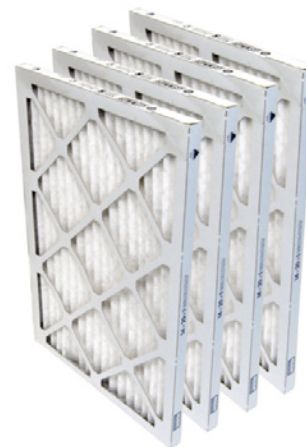
Building America recommends a MERV 8 or higher filter on the HVAC return. MERV (Minimum Efficiency Reporting Value) is a measure of an air filter's efficiency at removing particles. [This exceeds the ASHRAE 62.2-2010 6.7 recommended MERV 6 or better.]
