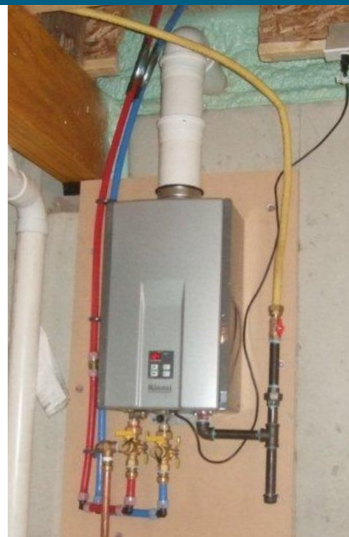
The tankless gas-fired water heaters installed by Nelson Construction in Farmington, Connecticut, save energy by eliminating the stand-by losses inherent with storage tank water heaters.
