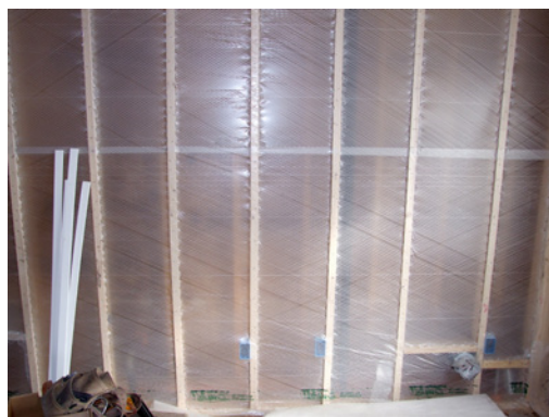
(top) The double-stud wall consists of two 2x4 16-inch-on-center framed walls set 5 inches apart.
