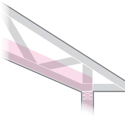
Some builders use cantilevered trusses to get full height insulation over the exterior wall.
