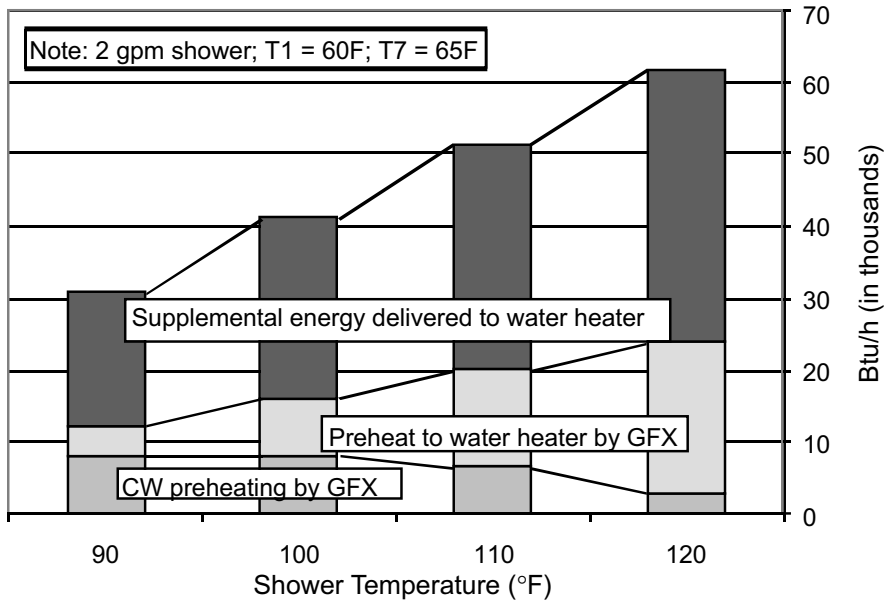
Figure 2. Heat exchange from GFX.
