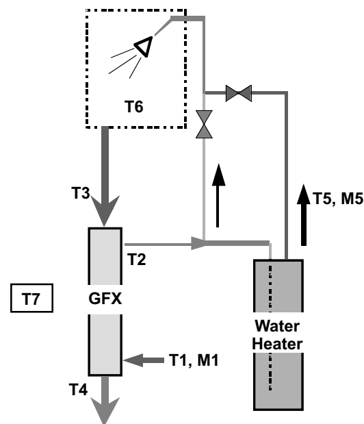
Figure 1. Layout of GFX system in residential application.
