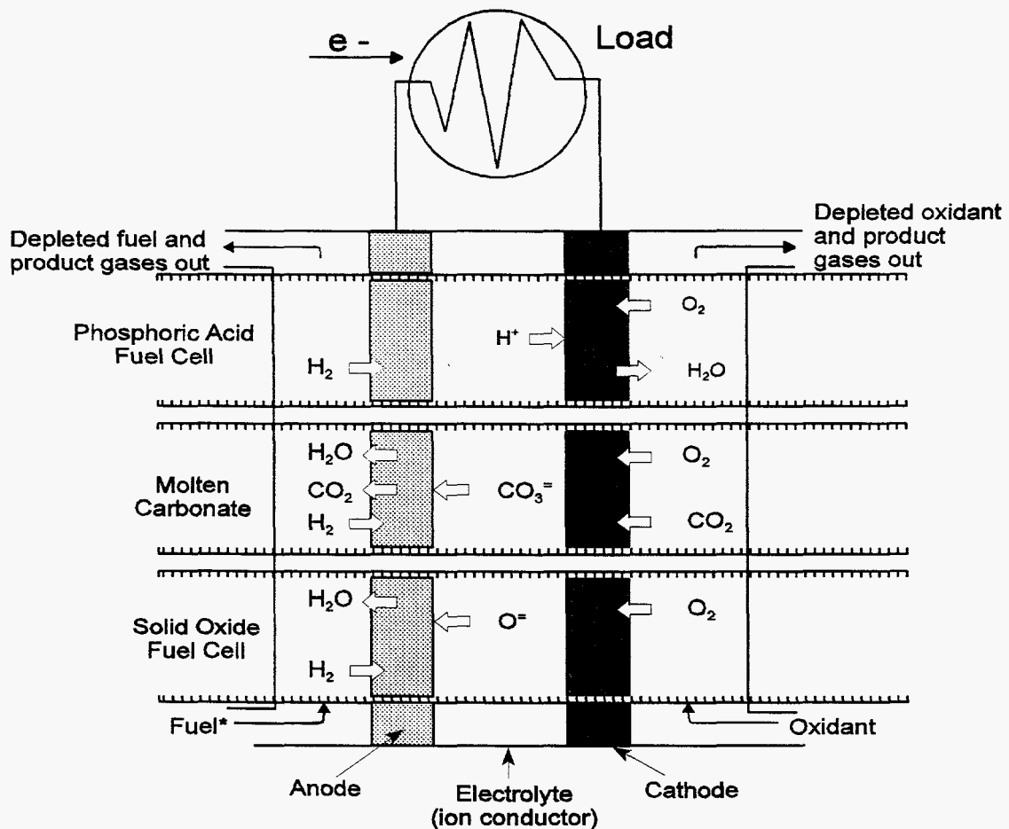
EXHIBIT 4 REPRESENTATIONS OF THREE TYPES OF FUEL CELLS
