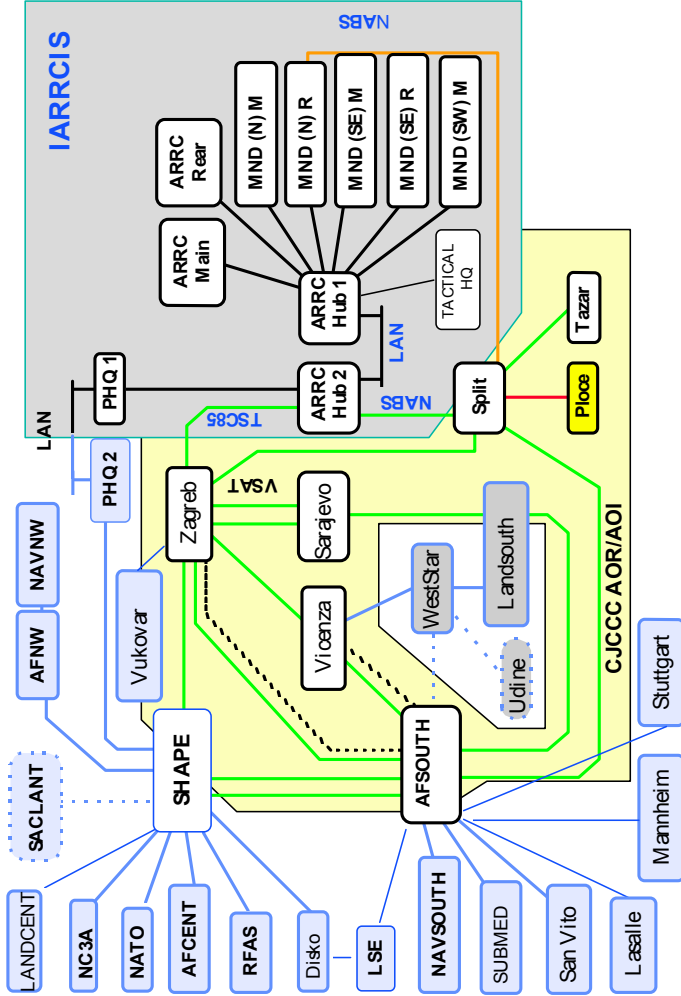
Figure 11-9. CRONOS/IARRCIS Network
