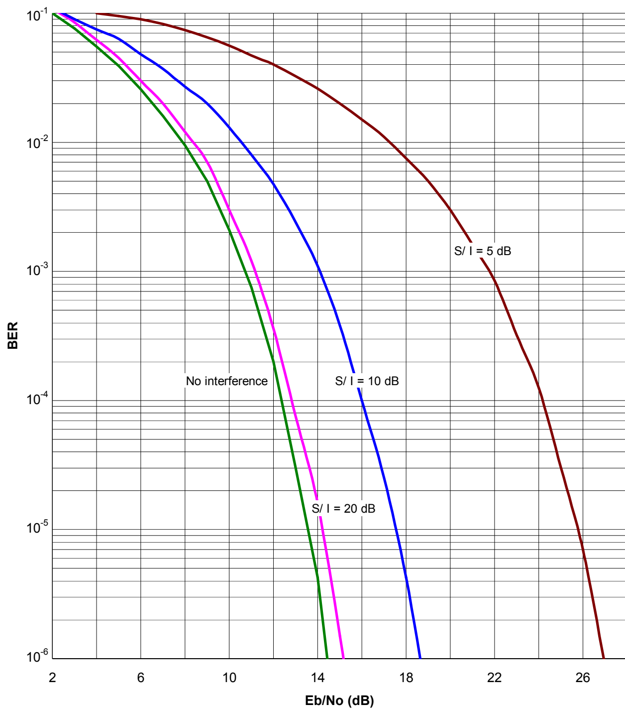
Figure 6-20. BER vs. E_b/N_0 Curves for QAM Receiver ( M = 16 ) with CW Interference
