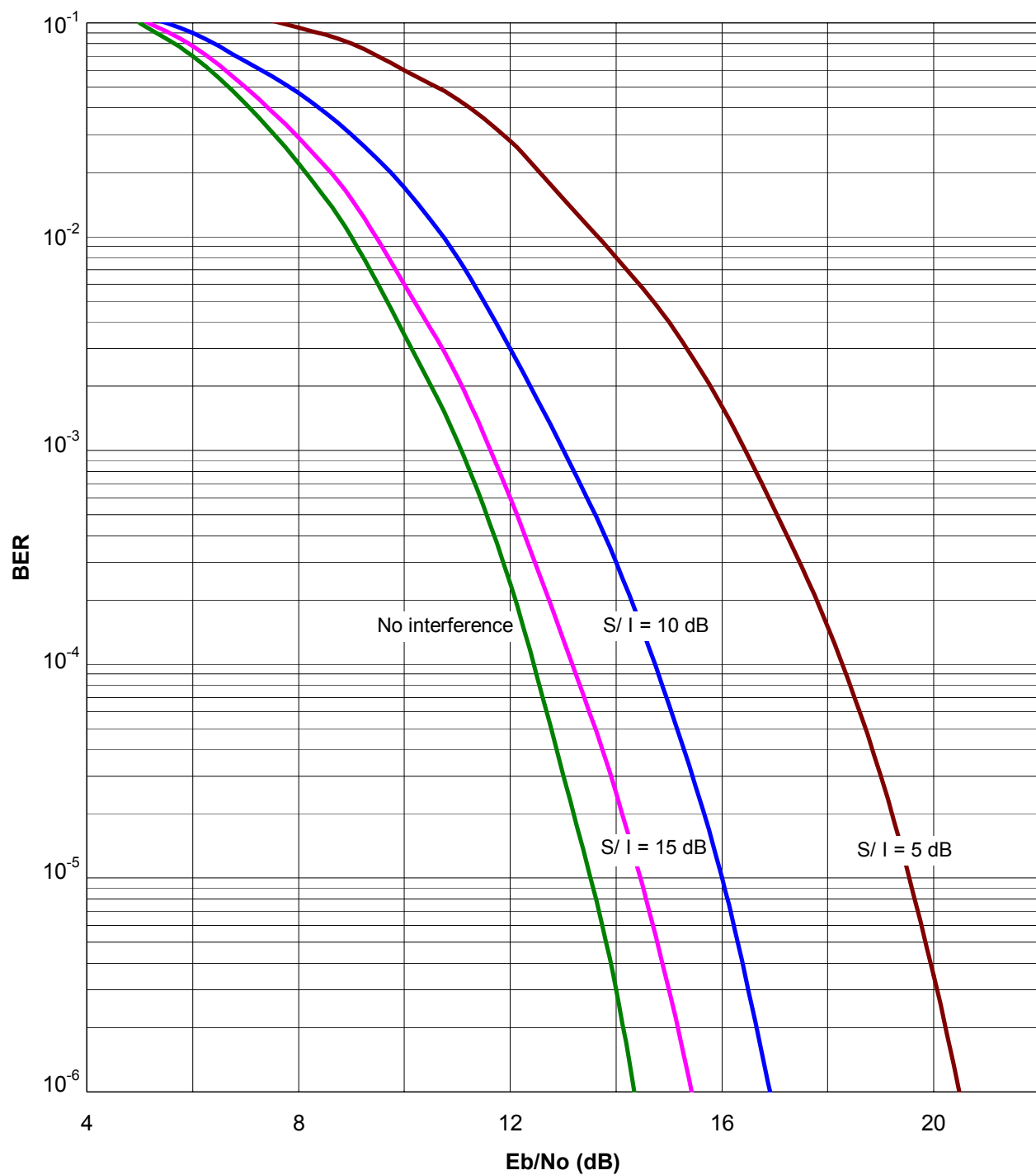
Figure 6-10. BER vs. E_b/N_0 Curves for Noncoherent FSK Receiver ( M = 2 ) with CW Interference
