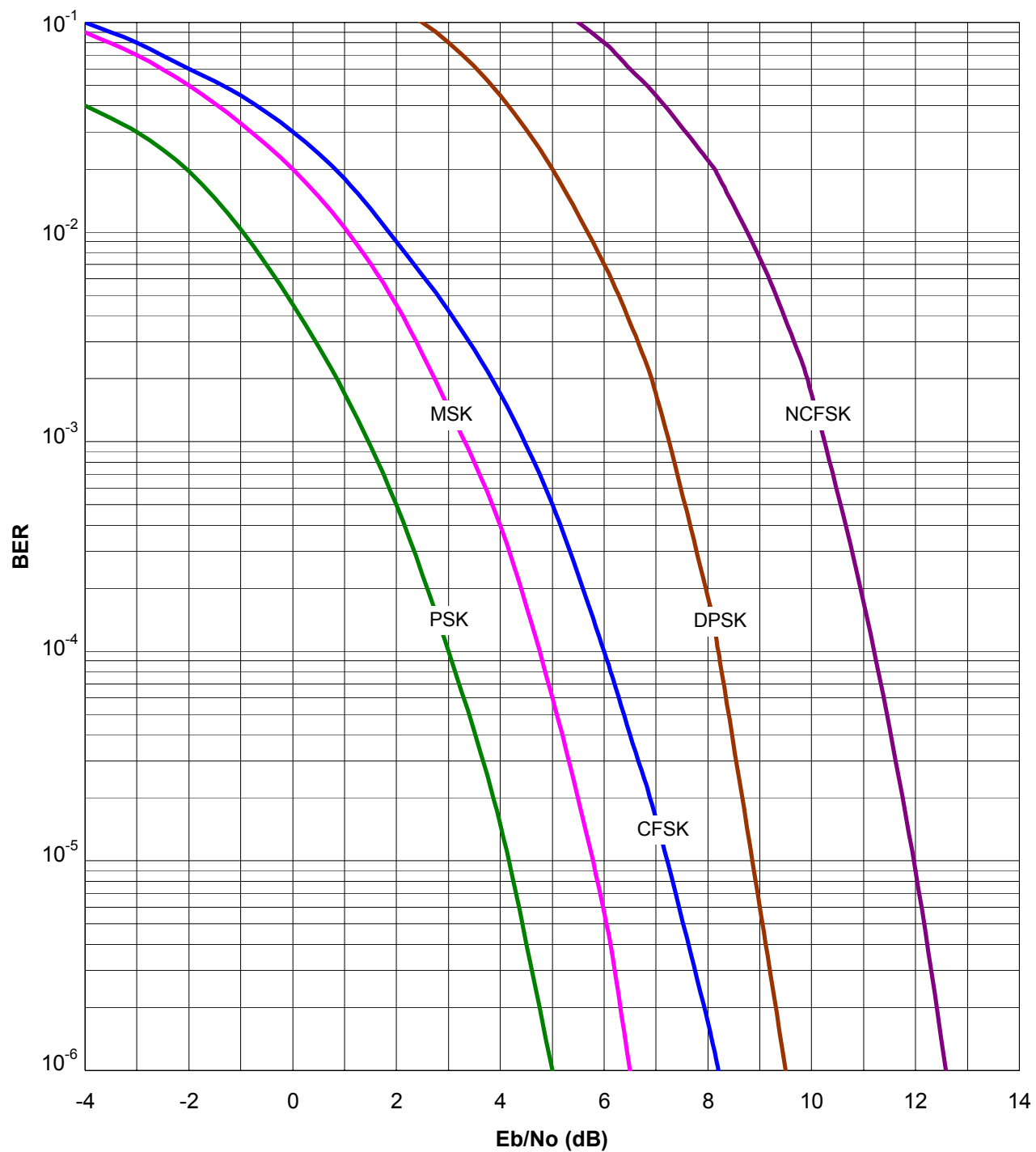
Figure 7-5. BER vs. E_b/N_0 Curves for Soft-decision (64, 6) Hadamard Decoder
