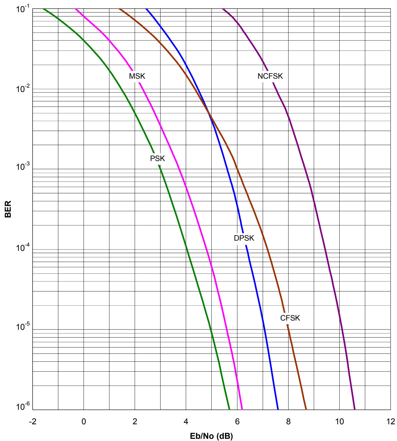
Figure 7-7. BER vs. E_b/N_0 Curves for Soft-decision (24, 12) Golay Decoder
