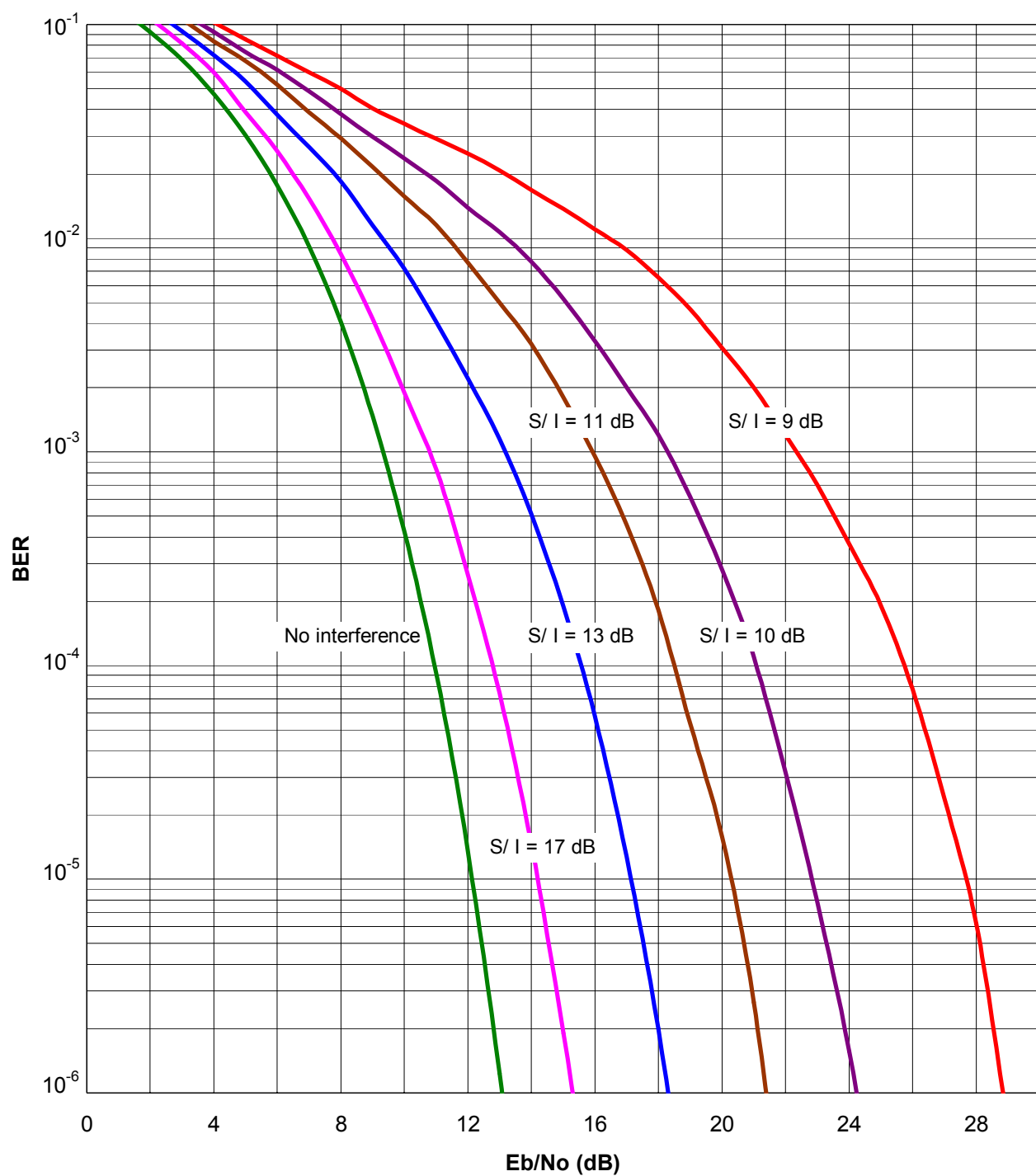
Figure 6-7. BER vs. E_b/N_0 Curves for DPSK Receiver ( M = 4 ) with CW Interference
