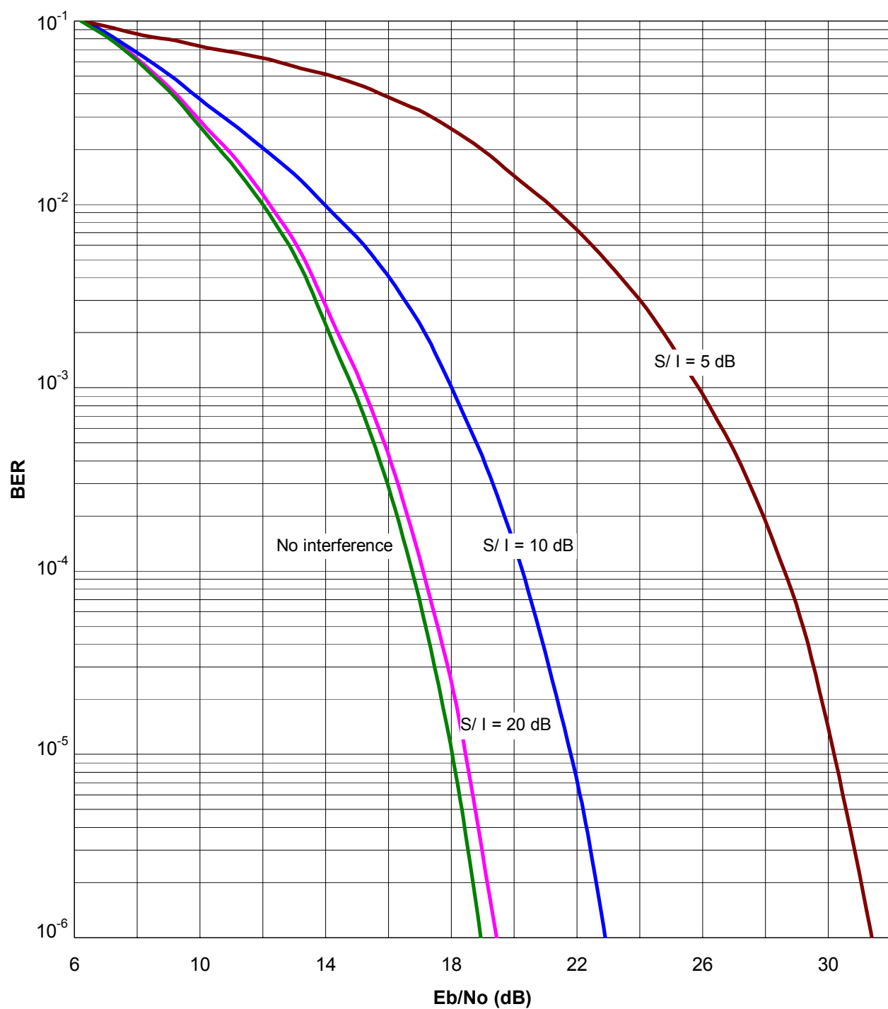
Figure 6-21. BER vs. E_b/N_0 Curves for QAM Receiver ( M = 64 ) with CW Interference
