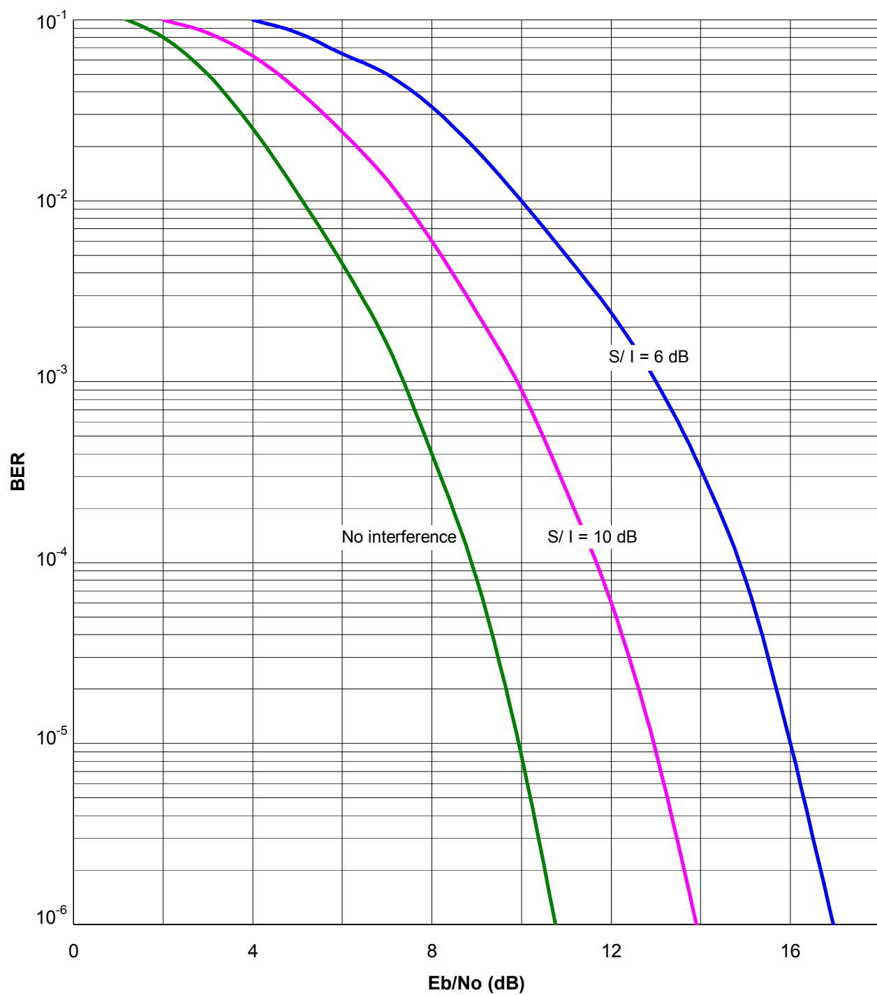
Figure 7-13. BER vs. E_b/N_0 Curves for Binary CPM Decoder (Modulation Index 1/2)
