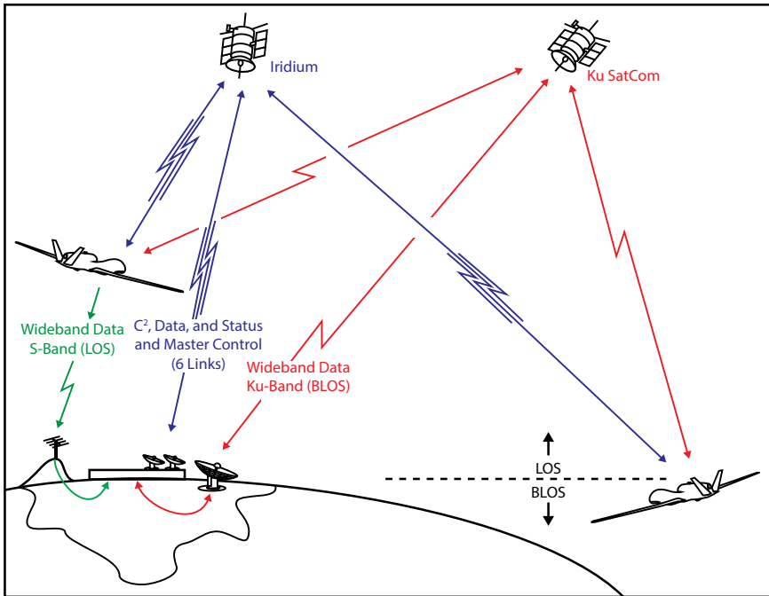
Figure 6. RQ-4 Global Hawk system architecture
