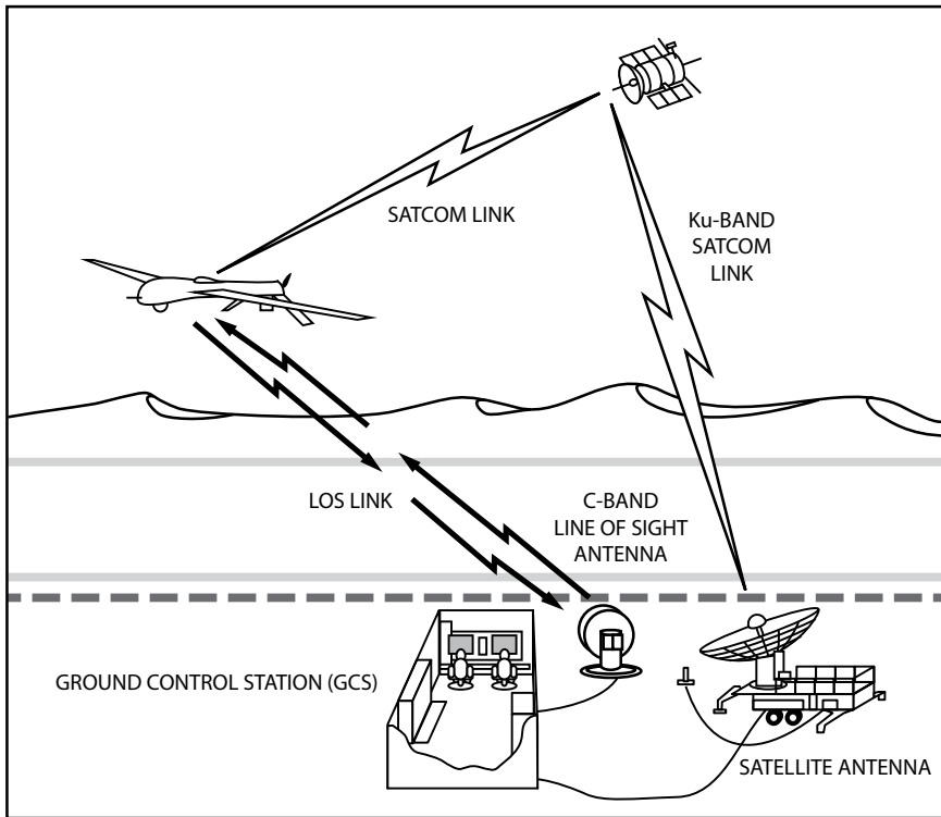
Figure 5. MQ-1 and MQ-9 LOS and BLOS configuration
