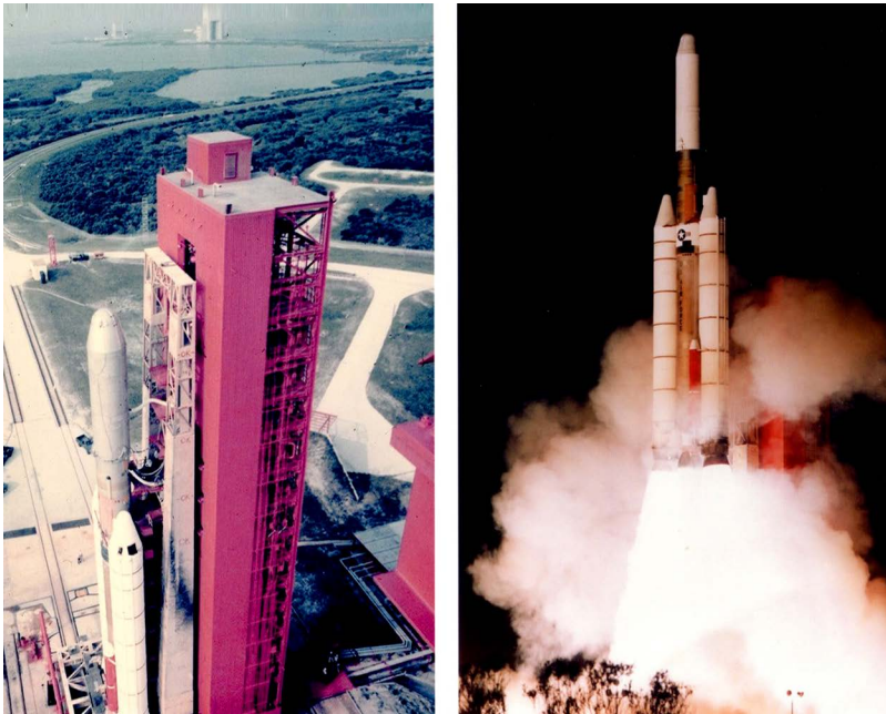
Fig. 14. The Titan 34D launch vehicle at LC-40, launching 30 October 1982. (Photo courtesy of John Hilliard)
