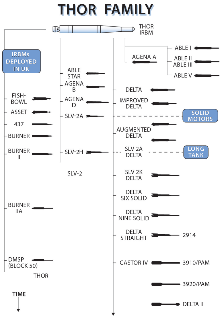
Fig. B.2. Evolution of the Thor space booster. (Adapted from ANSER, A Historical Look at United States Launch Vehicles, 1967–Present , ANSER Space Analysis Division, SADN 97-2 [Arlington, VA: ANSER Space Analysis Division, 1997], A-4.)
