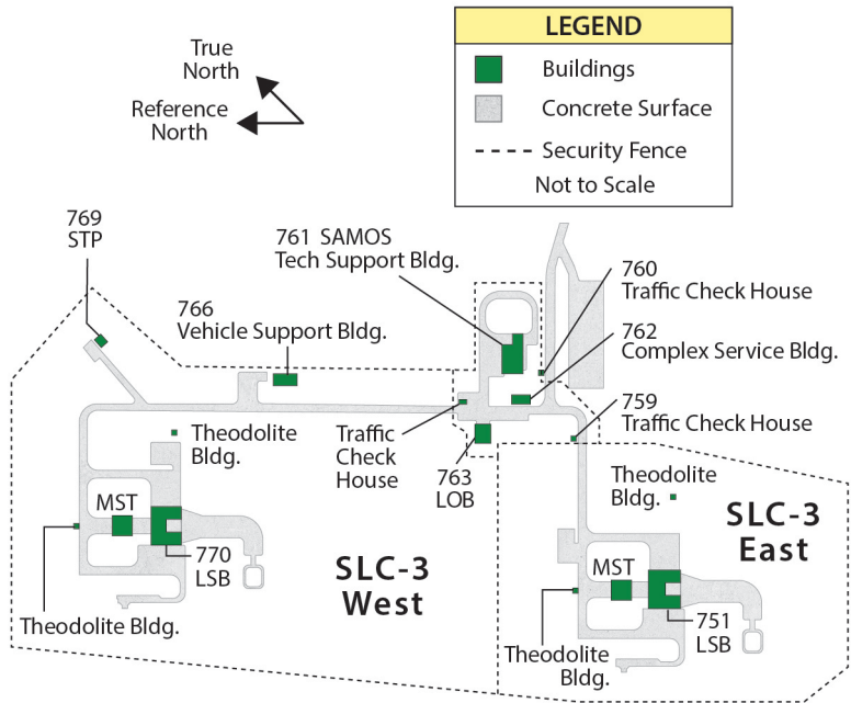
Fig. B.5. Space Launch Complex (SLC)-3, shown in a 1959 configuration. (Adapted from Historic American Engineering Record, National Park Service, Vandenberg Air Force Base, Space Launch Complex 3 [SLC-3], HAER No. CA-133-1 [San Francisco, CA: Historic American Engineering Record, National Park Service, Western Region, March 1993], 64.)
