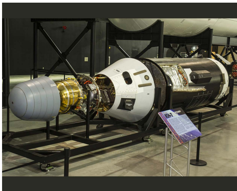
Fig. 5. The Gambit KH-7 camera system, as seen in a static museum display. (Photograph courtesy of the National Museum of the Air Force)
