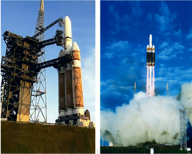
Fig. 22. The Delta IV Heavy on pad 37, left, and lifting off for its test flight, 21 December 2004. (Photo courtesy of John Hilliard)
