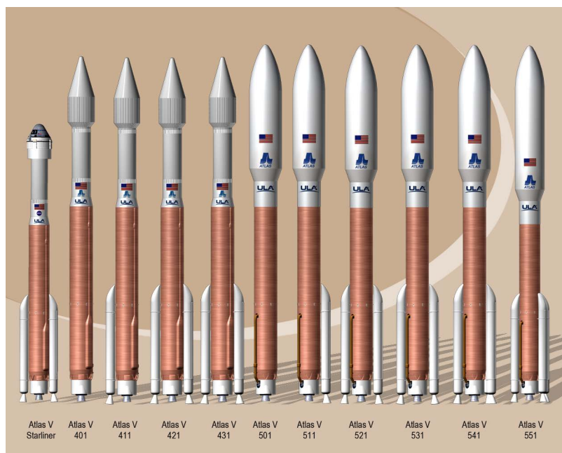
Fig. 21. The Atlas V vehicle family. (Photo courtesy of United Launch Alliance)
