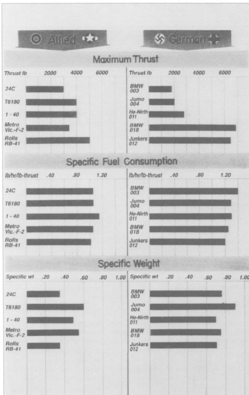
Figure 13—Characteristics of Turbojets
