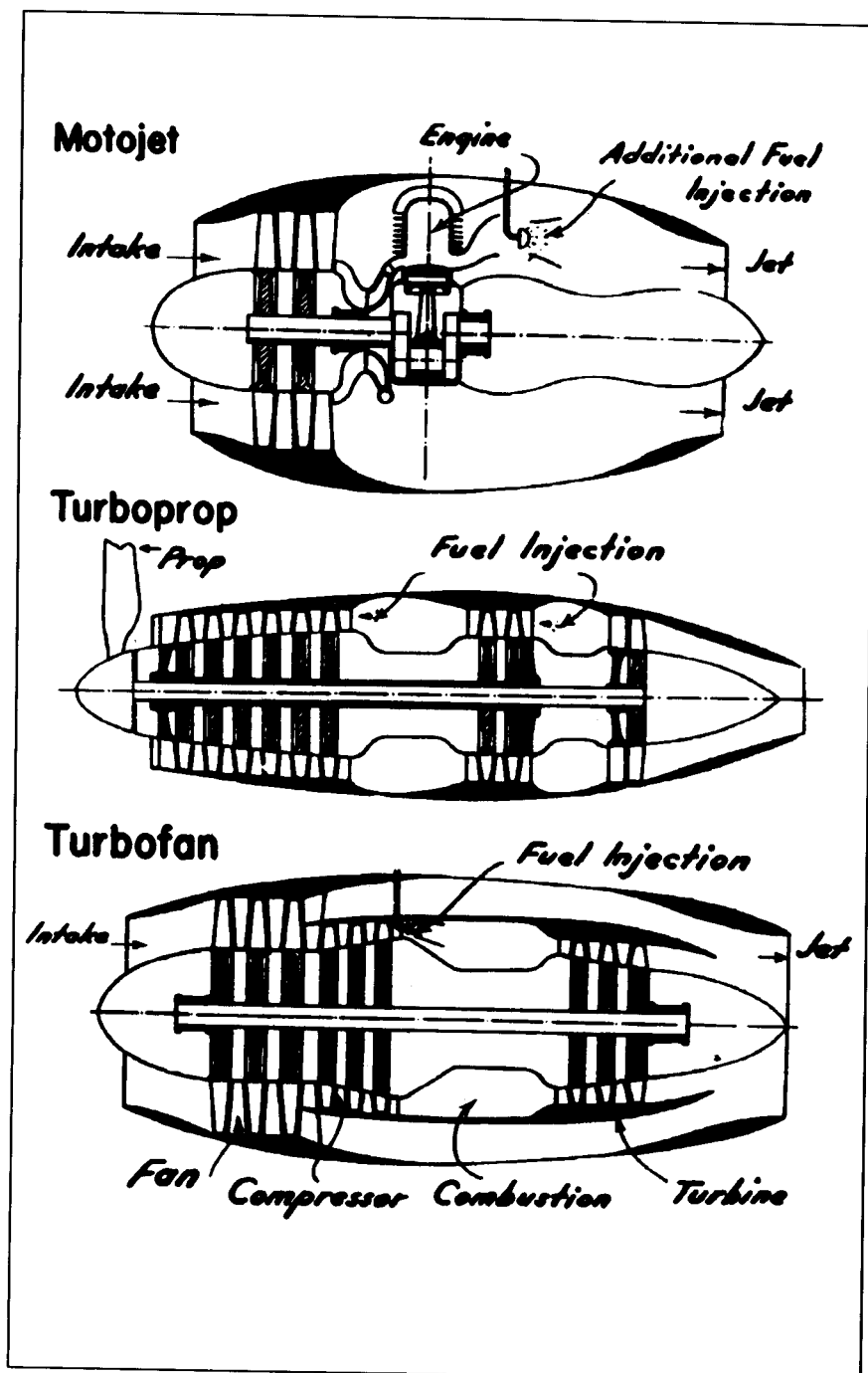
Figure 10-A—Various Propulsion Systems
