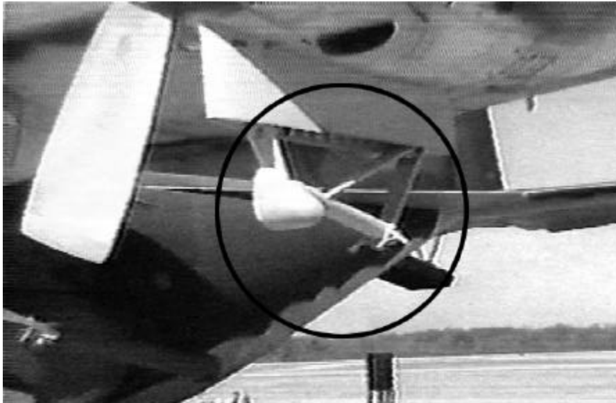
Two sets of Shrike rockets were mounted on an external pylon to stabilize the aircraft during takeoff.
