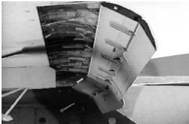
Double-slotted flap configuration used on Credible Sport.
