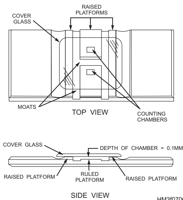
Figure 7-6.—Top and side views of a hemacytometer.
