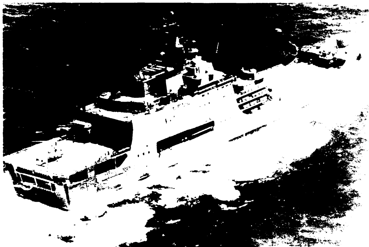
The IVAN ROGOV class LPD provides the Soviet Navy with a significant amphibious capability. The ship can carry air-cushion vehicles or conventional landing craft in its floodable well deck and, using its bow door and ramp, can offload its cargo over the beach. It also has a hanger and two helo landing decks.
