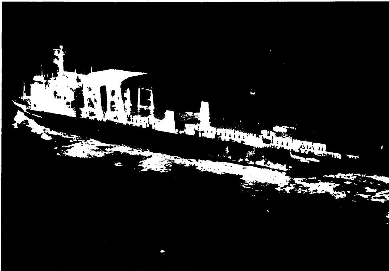
STAKHANOVETS YERMOLENKO is one of three Finnish-built heavy-lift load carriers of the STAKHANOVETS KOTOV class. These ships can be loaded and unloaded using roll-on/roll-off, lift-on/lift-off and/or float-on/float-off methods. Besides the 700-ton lift capacity gantry cranes, these ships have a floodable well deck with a stern gate.
