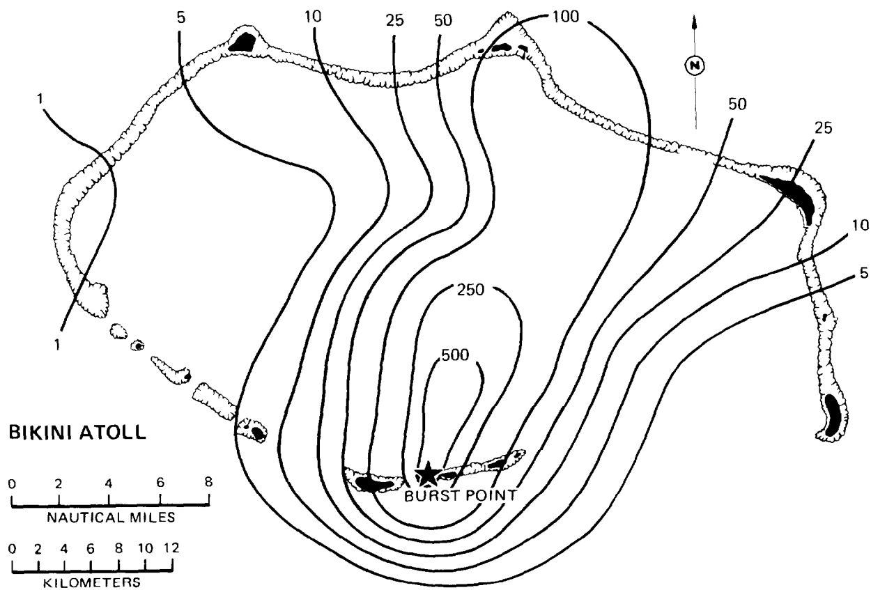
Figure 79. CASTLE, K00N close-in gamma fallout pattern (R/hr) at H+1 (source: Reference 53, p. 78).
