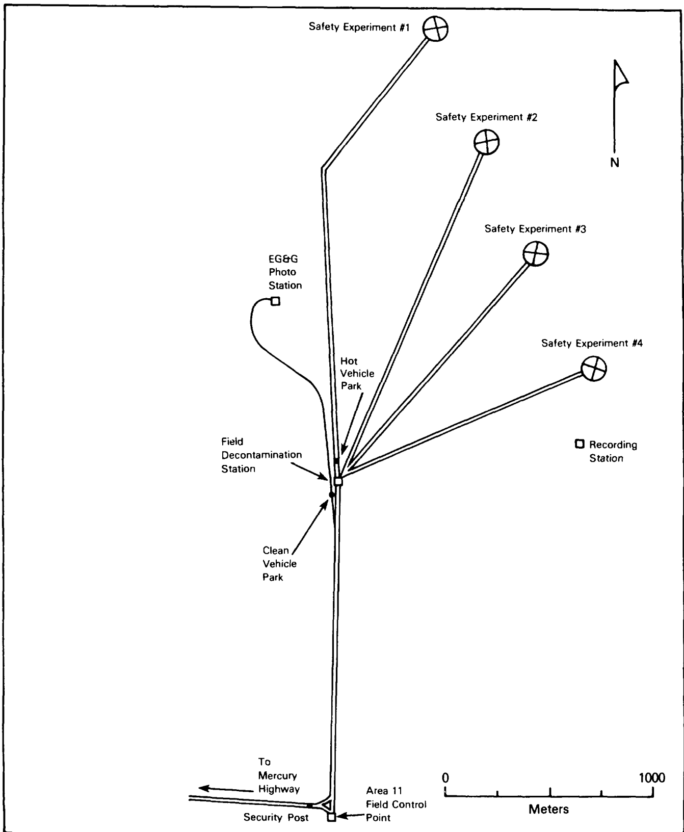
Figure 2-1: LOCATIONS OF PROJECT 56 GROUND ZEROS AND FIELD INSTALLATIONS
