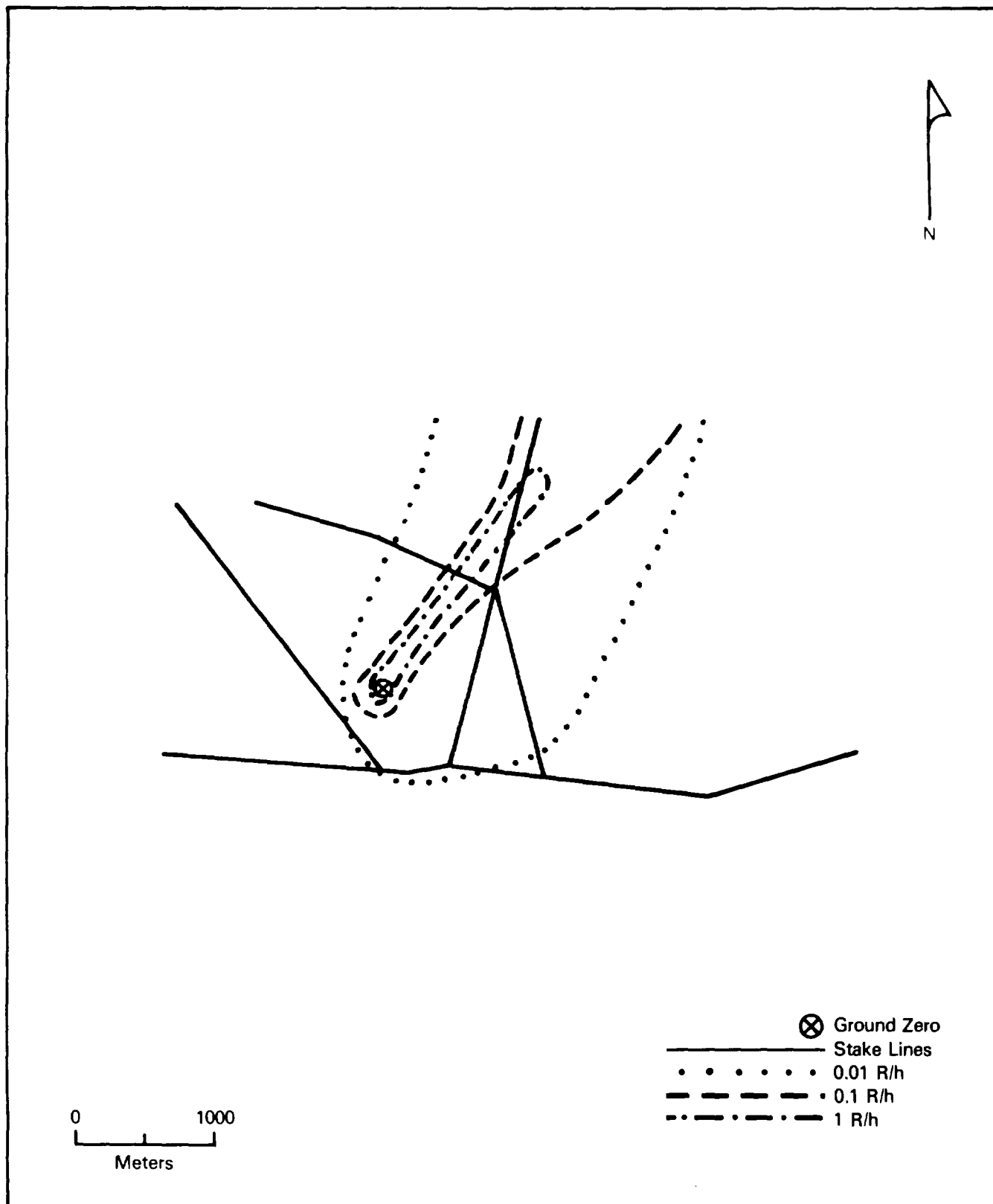
Figure 3-2: SURVEY FOR PASCAL A, 26 JULY 1957, MID-TIME 0929
