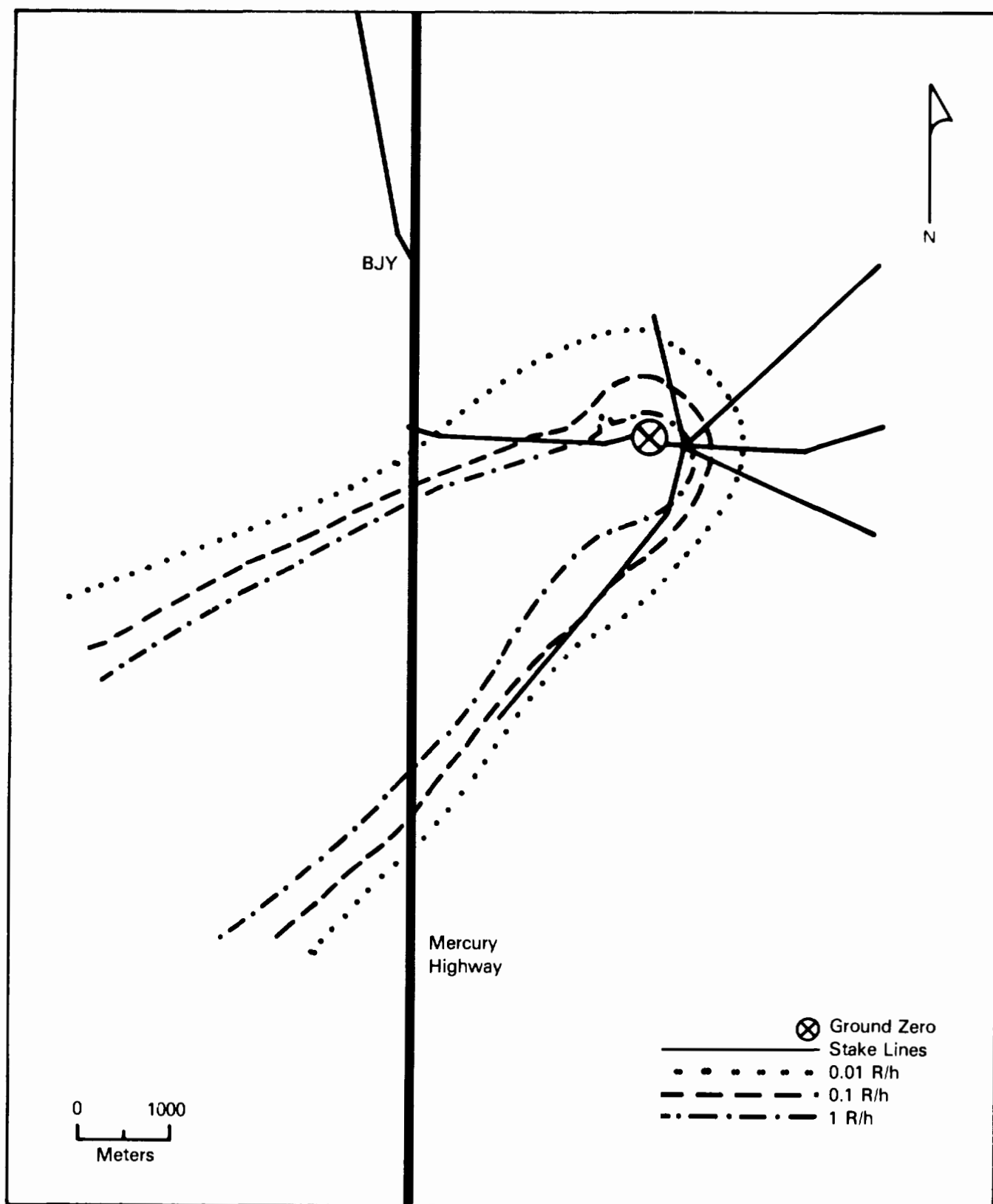
Figure 4-2: INITIAL SURVEY FOR COULOMB C, 9 DECEMBER 1957, MID-TIME 1341
