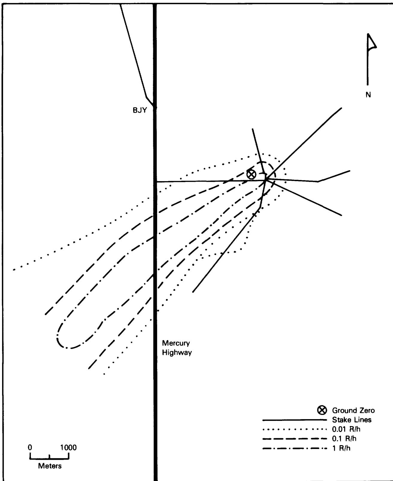
Figure 4-3: RESURVEY FOR COULOMB C, 10 DECEMBER 1957, MID-TIME 0945
