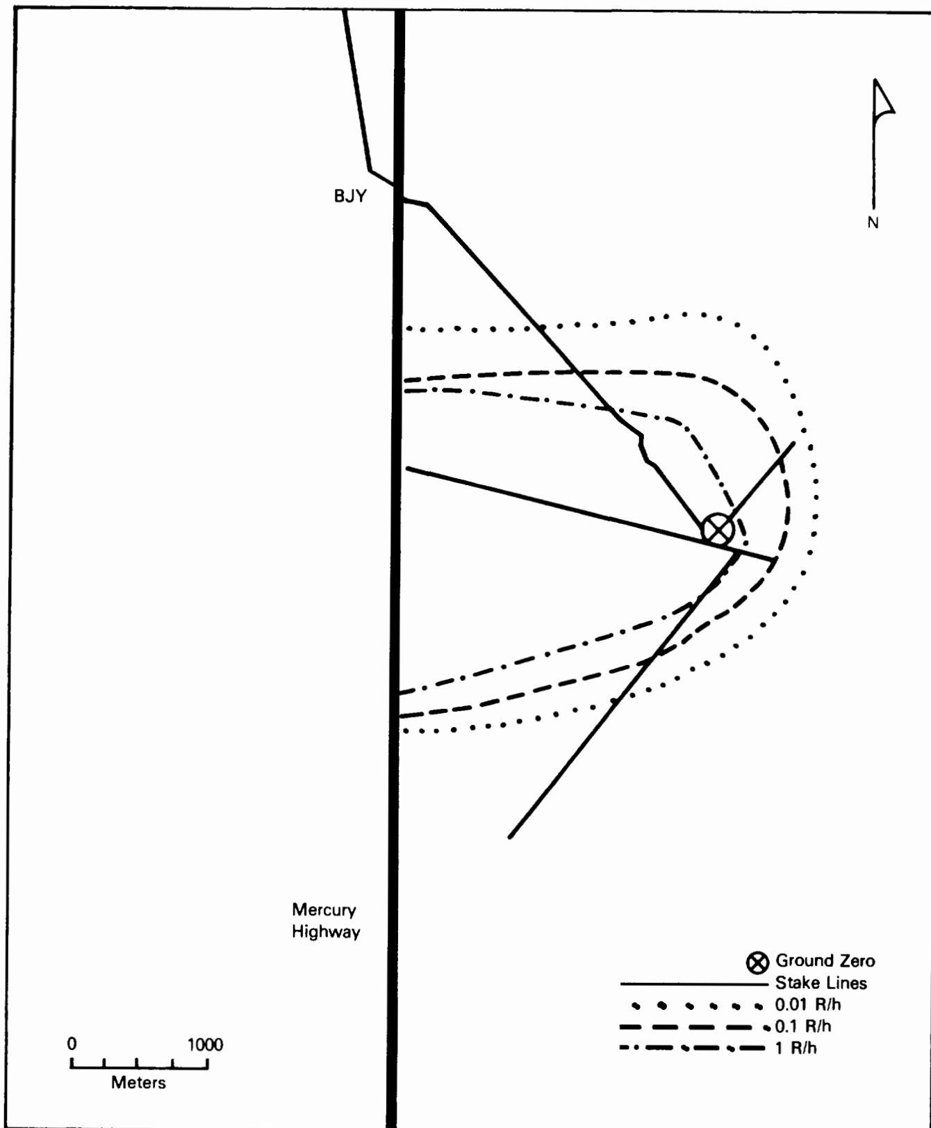
Figure 3-3: INITIAL SURVEY FOR COULOMB B, 6 SEPTEMBER 1957, MID-TIME 1344
