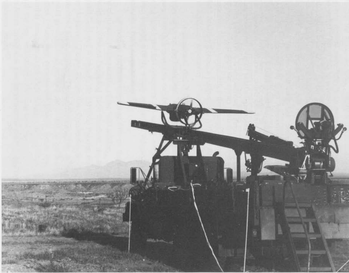
An Aquila Remotely Piloted Vehicle in launch position
