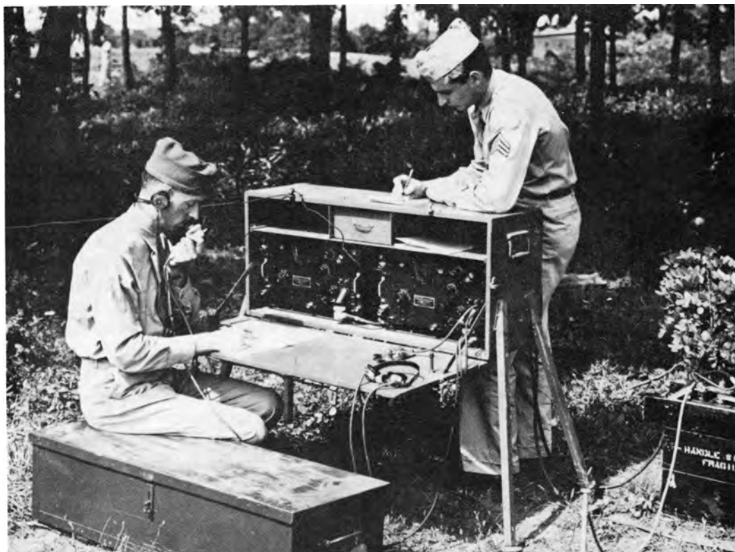
THE SCR-177. Receiving position showing the BC 314-C and BC 312-C receivers.
