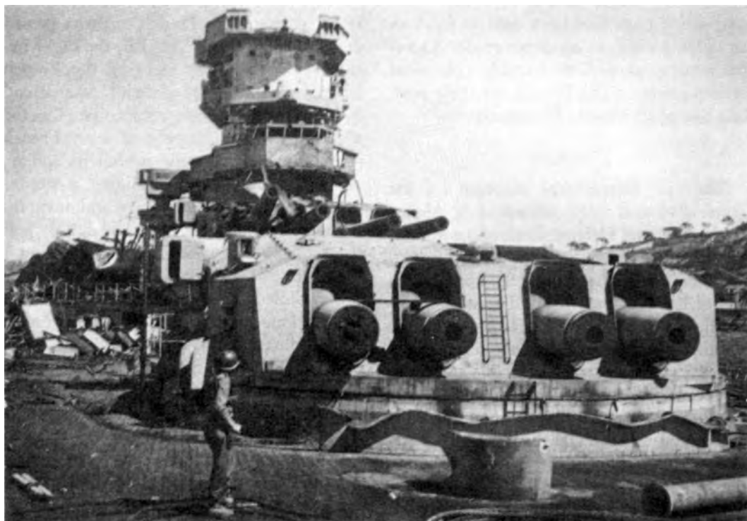
BATTLESHIP STRASBOURG , Toulon Harbor, September 1944. Note four lower turret guns, the ends of which were cut off when the French scuttled the ship in November 1942.
