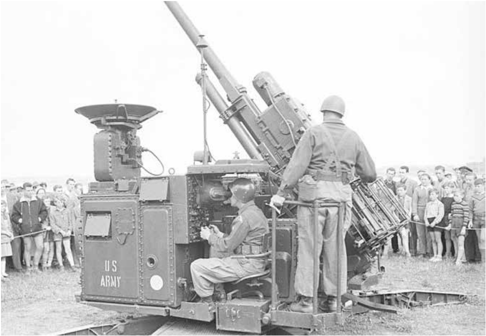
A radar-guided 75-mm. anti-aircraft gun, the U.S. Army's Skysweeper ( Stadtarchiv Kiel, Schleswig-Holstein, Germany )
