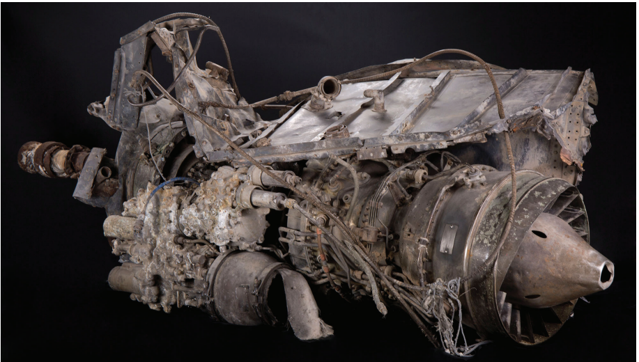
A UH–60 Black Hawk engine from the wreckage of the first helicopter shot down during the Battle of Mogadishu, Somalia
