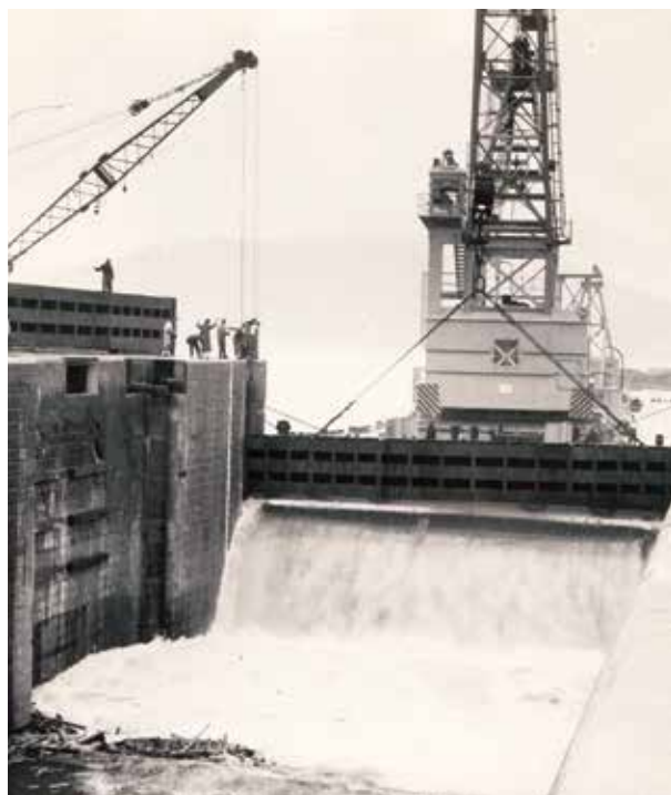
Removal of the stop-log from the canal lock at Incheon Tidal Basin, September 1960. Credit: Photo by PFC D. Heyde, FED, FED-PAO Historical Files.
