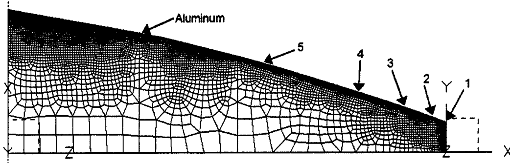
Figure 18. Axisymmetrical Finite Element Model of the Yawsonde.
