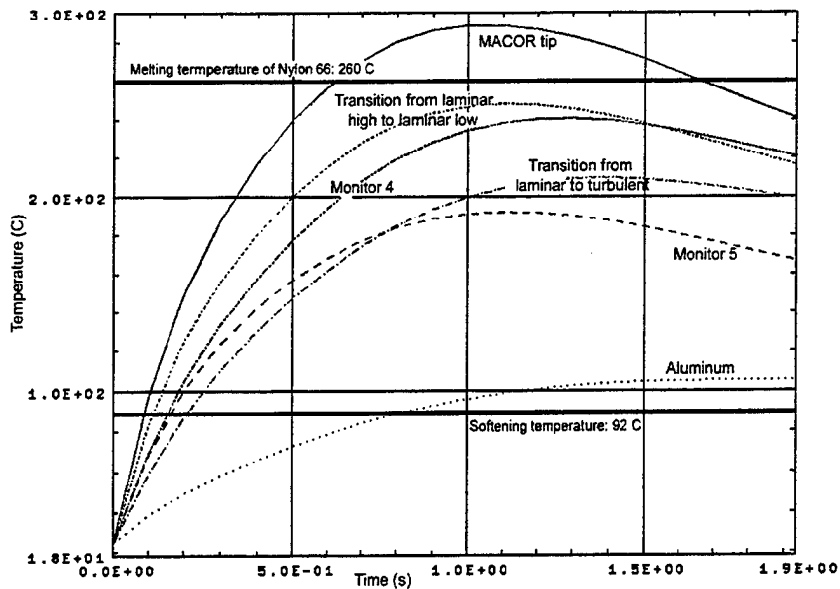
Figure 19. Computed Temperature Response of a Yawsonde With a Mach 3 Launch and a Laminar to Turbulent Transition Boundary Layer Scheme.
