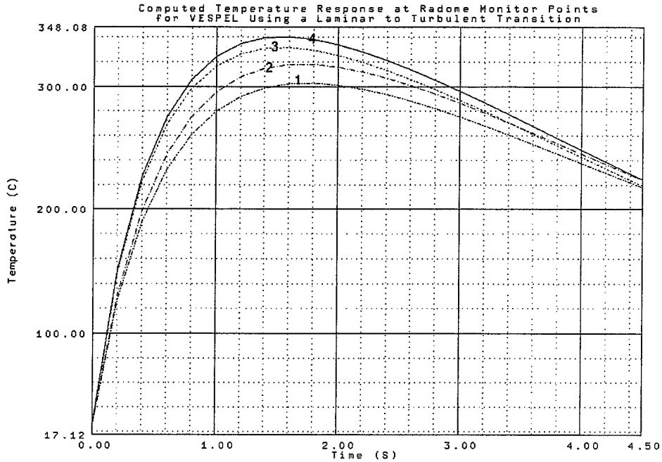
Figure 12. Computed Temperature Response at Radome Monitor Points for Vespel® With a Laminar to Turbulent Transition.
