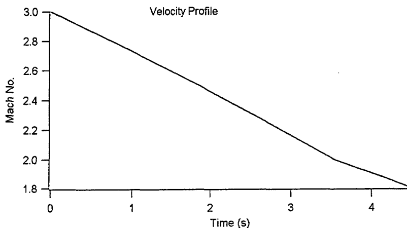
Figure 2. Experimental Velocity Profile.
