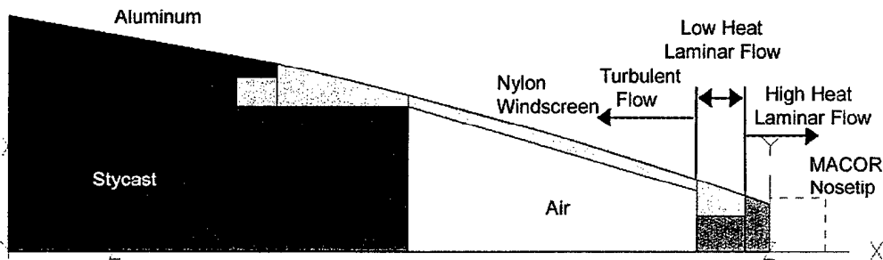
Figure 17. Axisymmetrical Layout of the Yawsonde Model.
