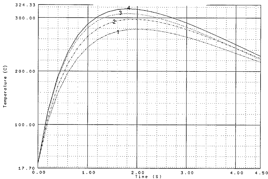
Figure 11. Computed Temperature Response at Radome Monitor Points for Celazole ® With a Laminar to Turbulent Transition.
