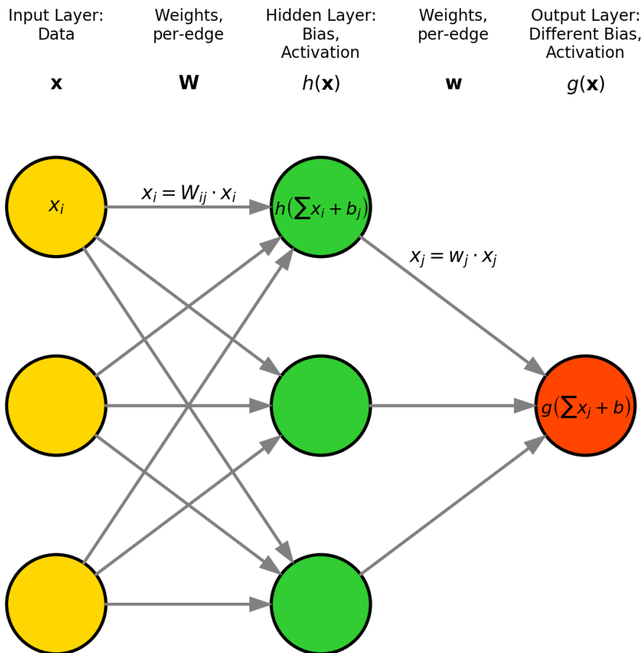
Fig. 1 Information flow of a small feed-forward neural network (also known as multilayer perceptron), drawn with nodes (circles) and edges (arrows). Input nodes are drawn in yellow, hidden nodes in green, and the output node in orange. Math operations are shown for a subset of the network.
