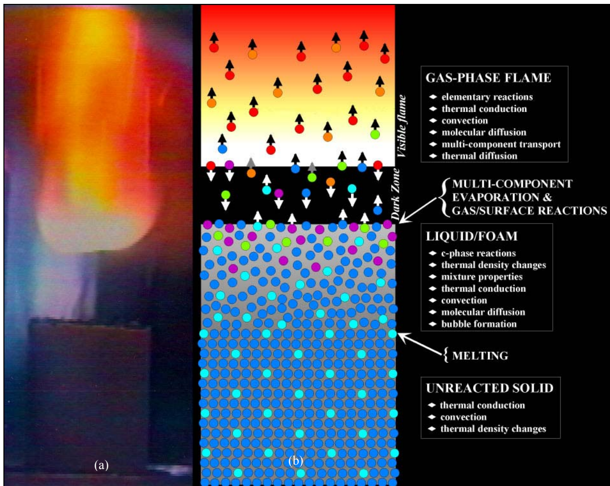
Figure 1. Photograph of an (a) RDX-composite propellant (M43) deflagrating at 1.6 MPa and (b) a caricature of the 3-phase molecular processes involved.
