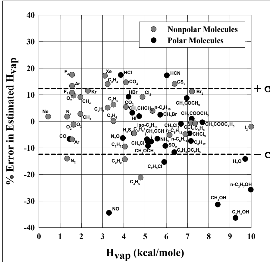
Figure 21. Accuracy of the simple heat-of-vaporization theory using 61 L-J parameter sets for both polar and nonpolar molecules.
