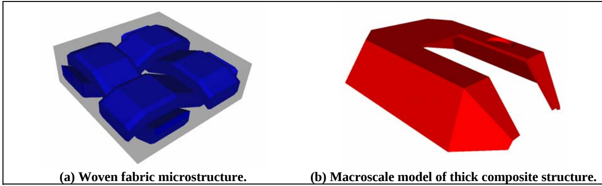
Figure 10. Visual example of micro and macroscale MSStress models.
