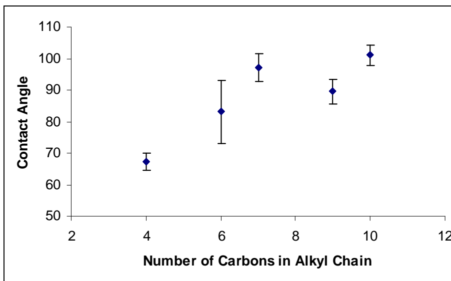
Figure 3. Contact angle of PVP grafted films.
