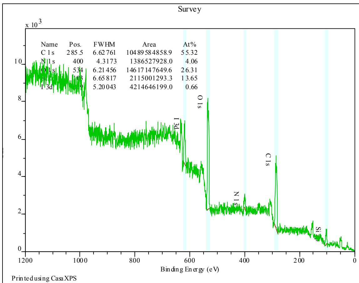
Figure 6. Survey spectrum of quaternary ammonium salt surface.
