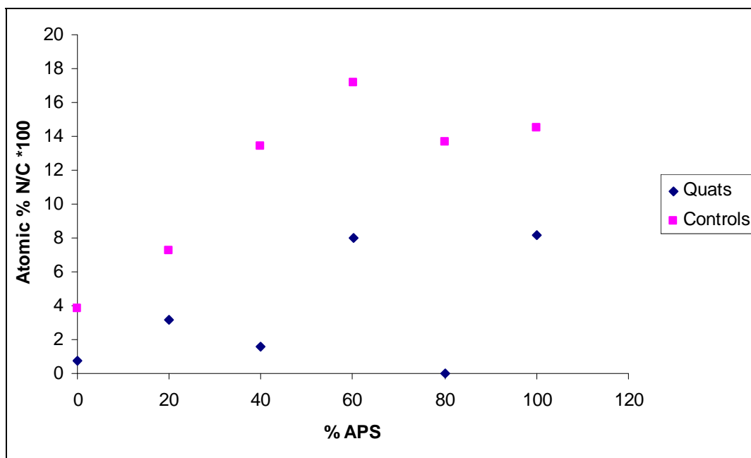
Figure 5. XPS N/C ratios of method B controls and quaternary nitrogen samples.
