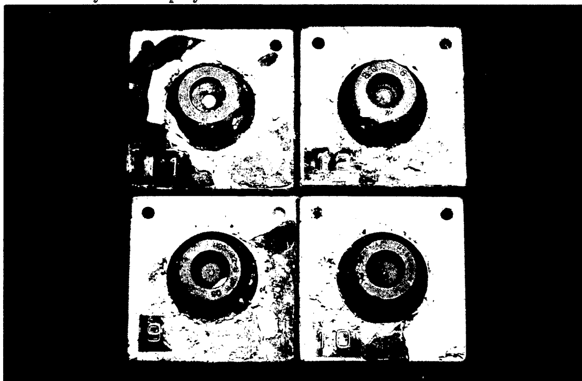
Figure 74. Inconel 718 Nickel-Based Superalloy Bolt Heads With Antiseize Solid Film Lubricant ( \text{MoS}_2 ) After 62 Days of Salt Spray. Reduced 25%.
