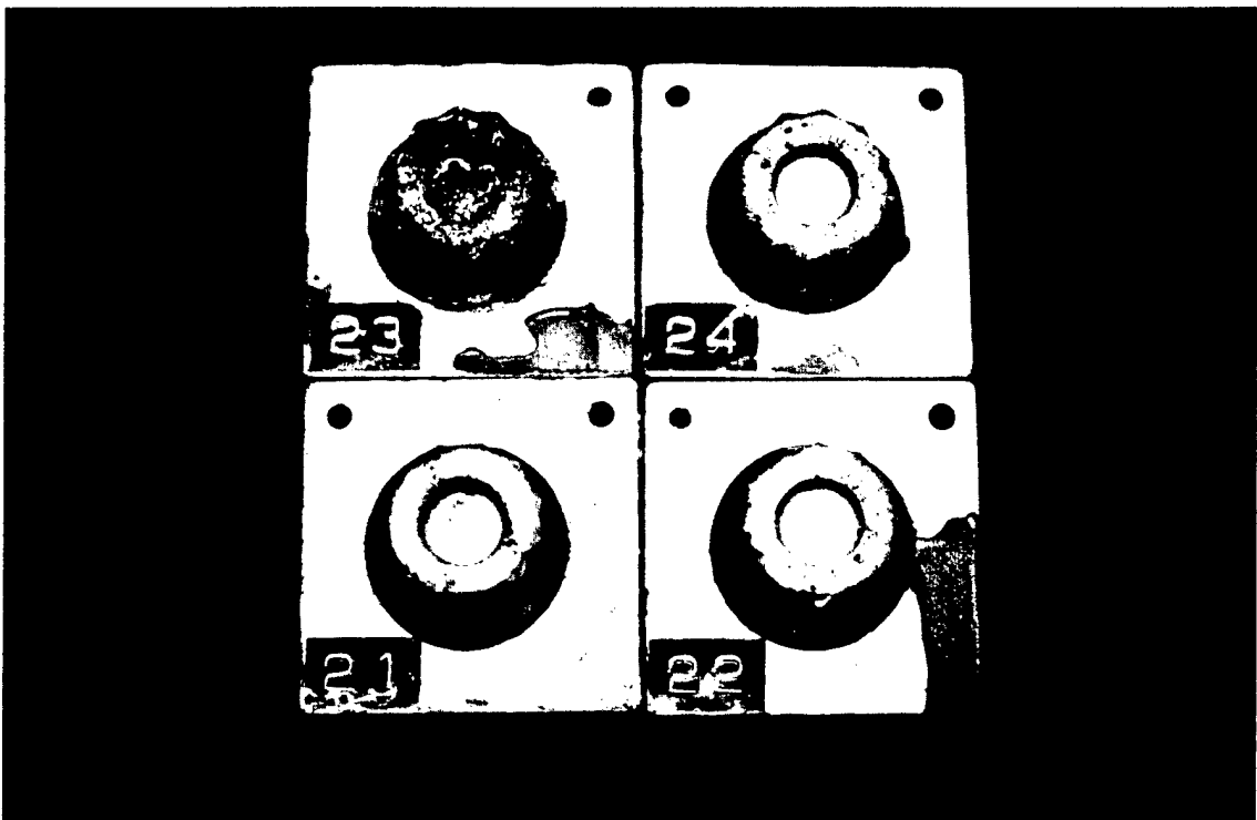
Figure 80. H11 Chromium Hot Work Tool Steel Bolt Heads With Cadmium Electroplate After 62 Days of Salt Spray. Reduced 25%.
