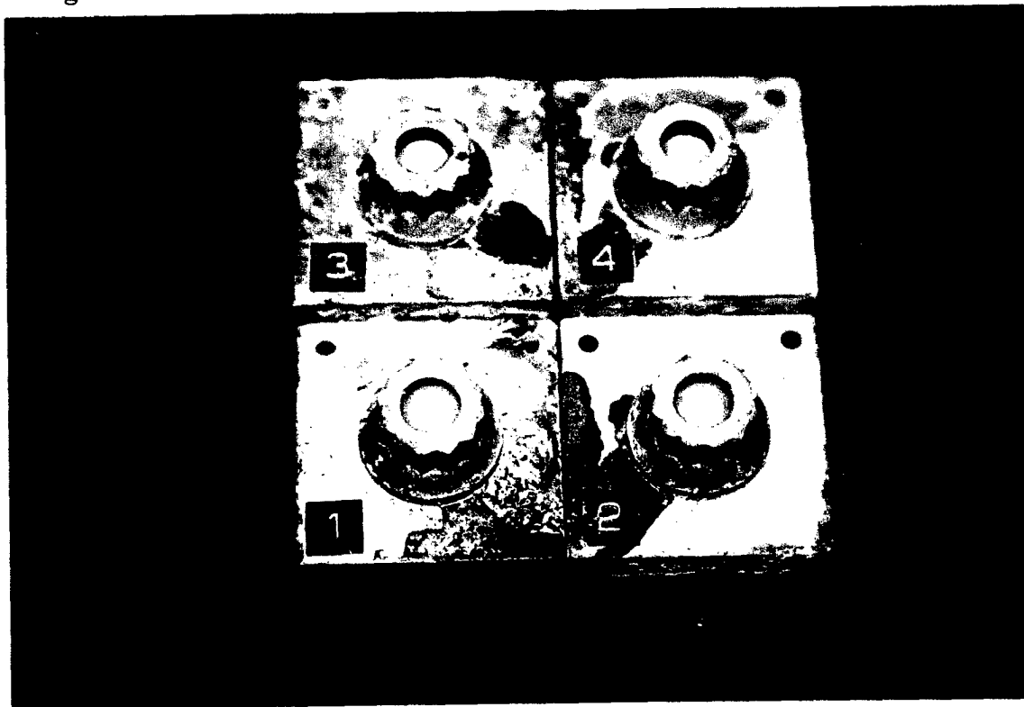
Figure 70. Inconel 718 Nickel-Based Superalloy Bolt Heads With IVD Al Coating After 62 Days of Salt Spray. Reduced 25%.
