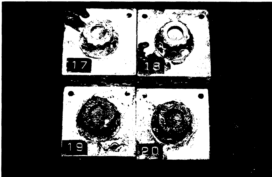
Figure 78. H11 Chromium Hot Work Tool Steel Bolt Heads With IVD Al Coating After 62 Days of Salt Spray. Reduced 25%.
