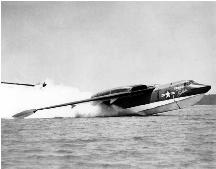
With tail obscured by water spray, Martin XP6M-1 SeaMaster accelerates for takeoff, 1956.
