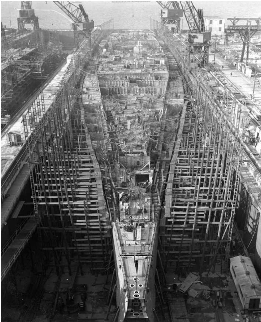
With hull surrounded by scaffolding, USS Forrestal (CVA-59) is under construction at Newport News Shipbuilding and Dry Dock Co., Newport News, Virginia, January 1954.
