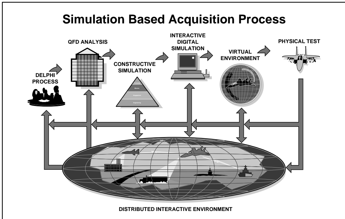
Figure 4-2. SBA Process
