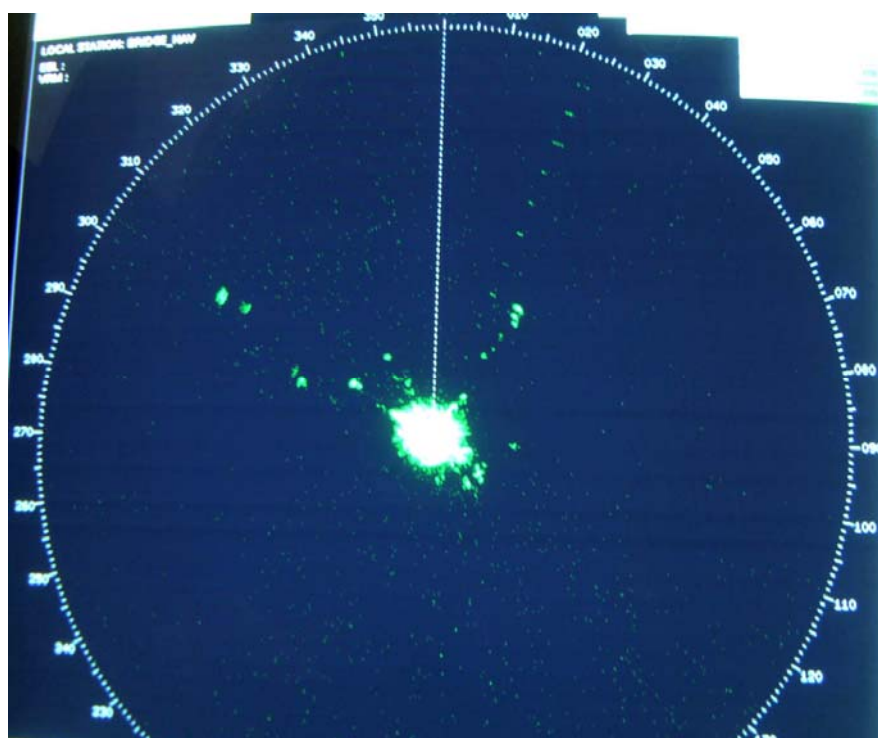
Figure A-4. +50 dB I/N , ungated, 10 \mu s pw, 1% duty cycle, IR on.
