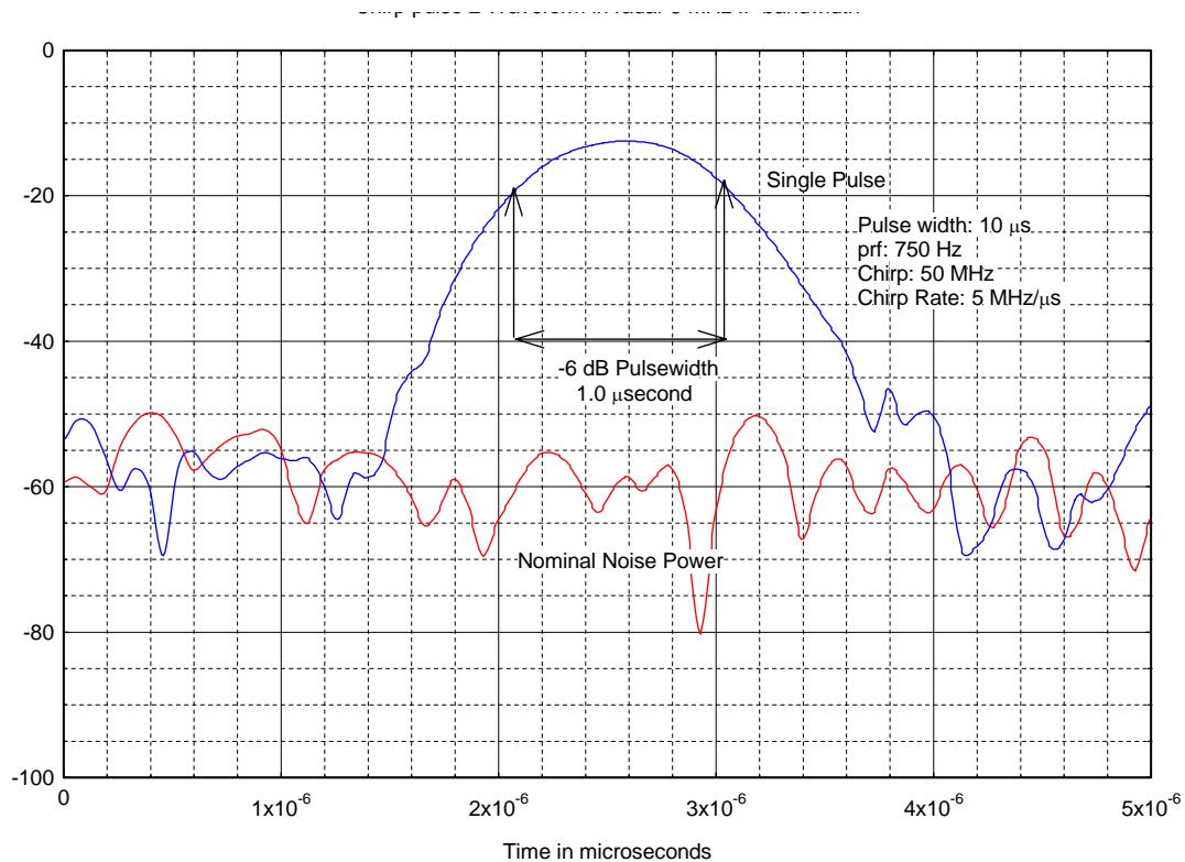
Figure D-4. Chirped waveform 2 in marine Radar F receiver.
