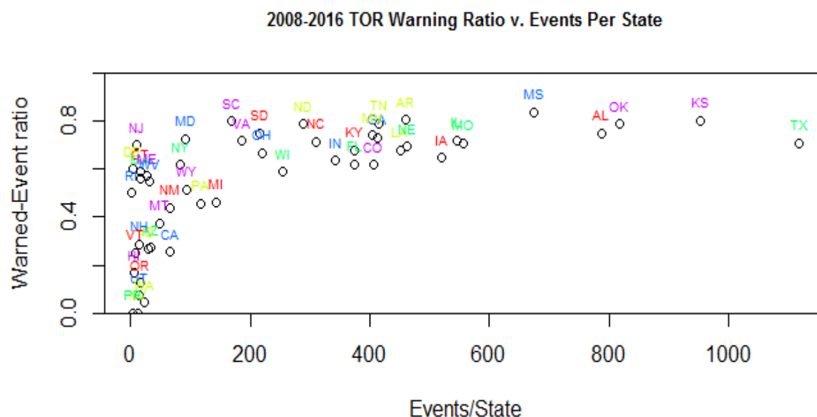
Figure 3. Warned tornado event fraction (from all events) as a function of tornado events per state for 2008-2016. There are very few tornado events in western states. The percent of events warned increases rapidly as the event rate grows and stays uniformly high past 200 events/state.
