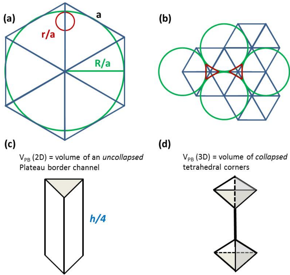
Figure 7. Determination of the volume fraction using Princen's model
