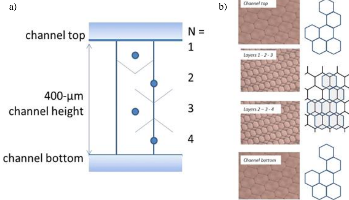
Figure 6. Interpretation of optical microscope images of the emulsion droplet tessellation.
