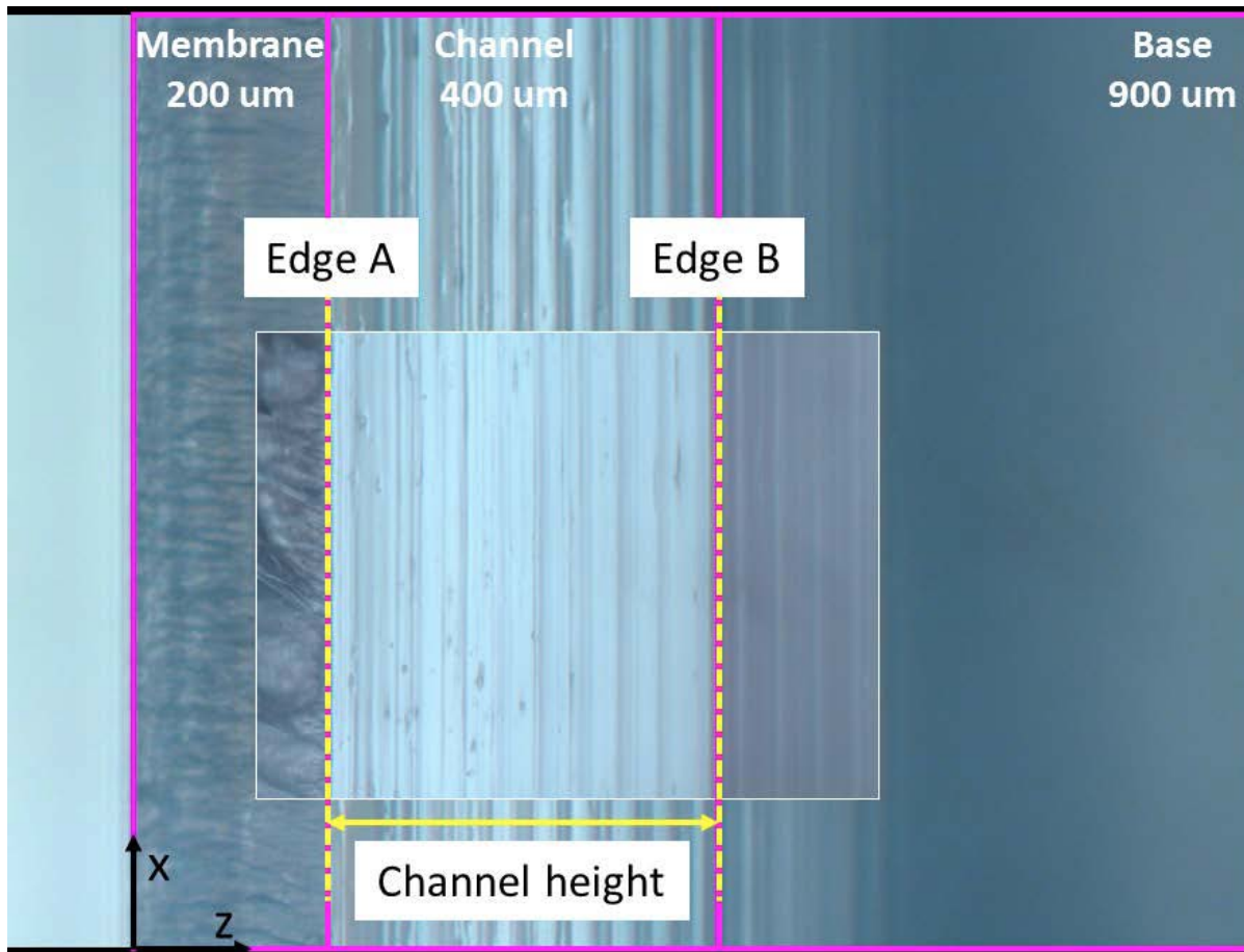
Figure 3: Cross sectional image of the microfluidic channel of nominally 400 \mu\text{m} channel height.
