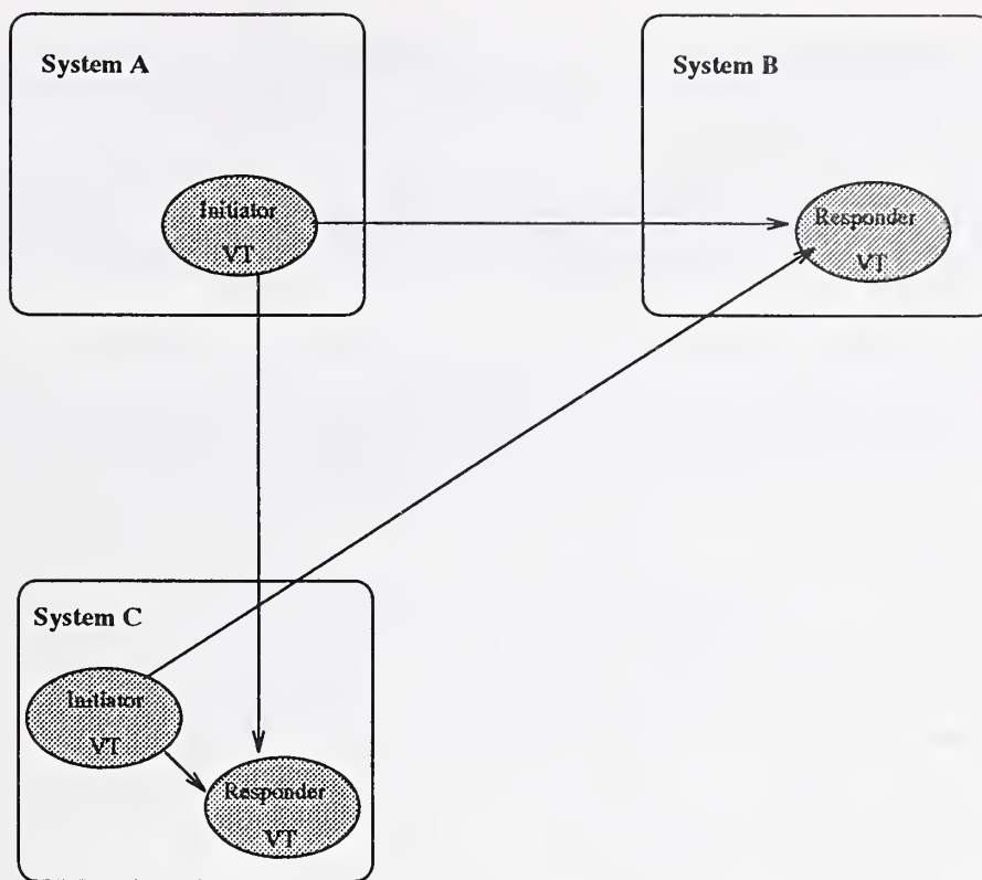
Figure 6.1: Initiator/Responder Relationship
