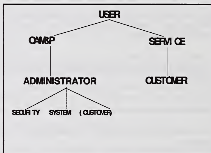
Figure 1 - User Roles.
