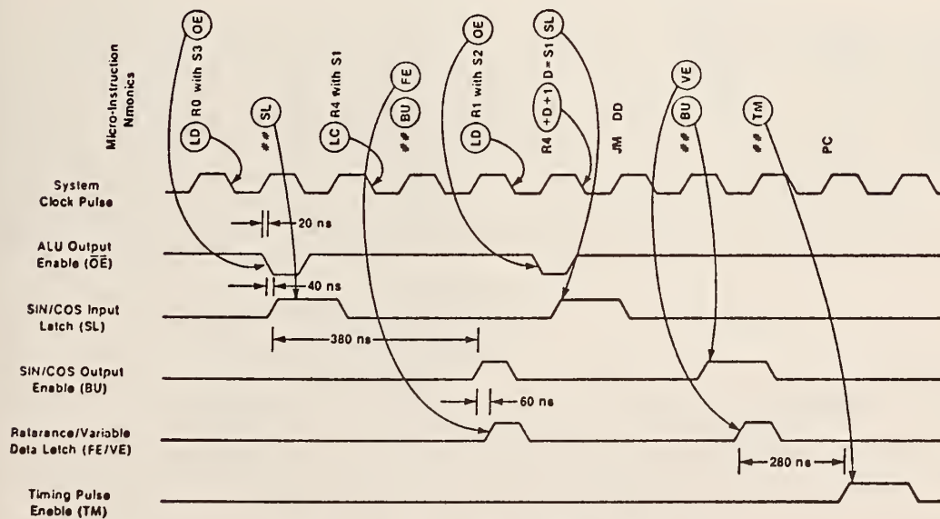
Timing Diagram of High-Speed Processor (Initial Cycle)
