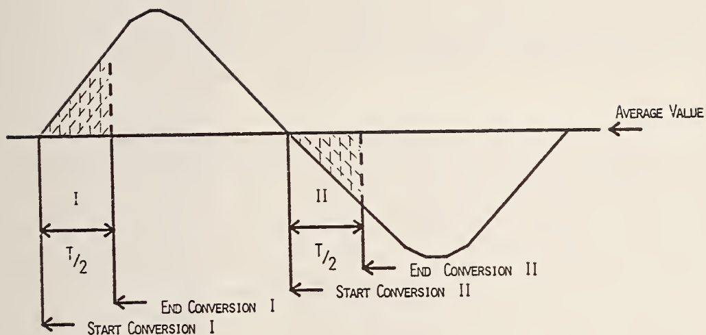
Figure 7.31 Digital Input Ripple
