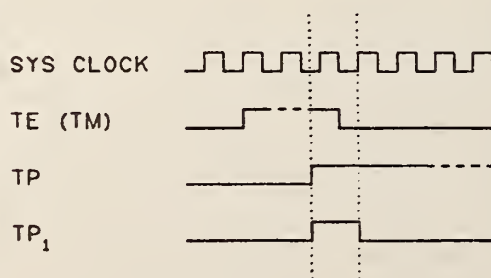
TIMING PULSE DIAGRAM
