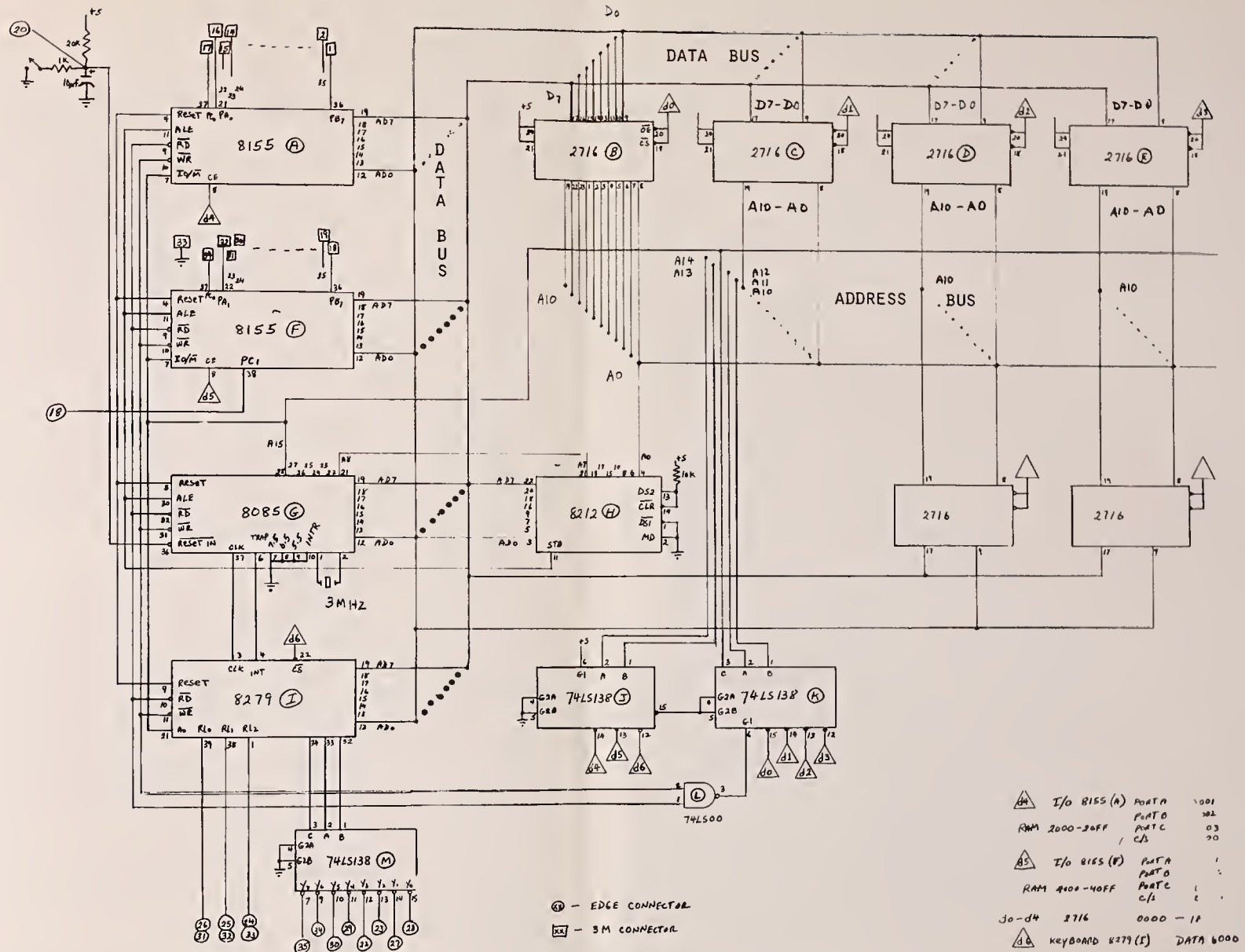
Fig. 7.33 8085 Microcomputer Circuit Dia. D-11
