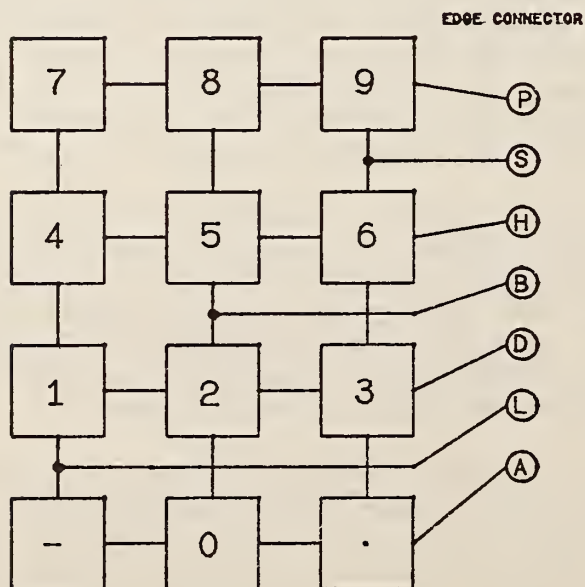
Figure 7.36 Number Keyboard
