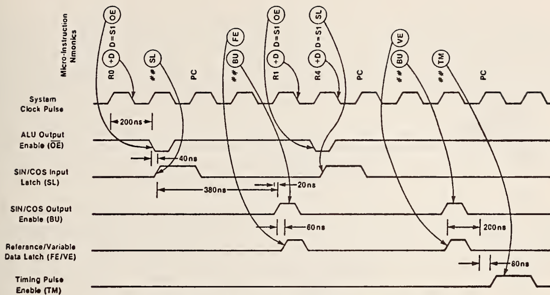
Timing Diagram of High-Speed Processor (Normal Cycle)
