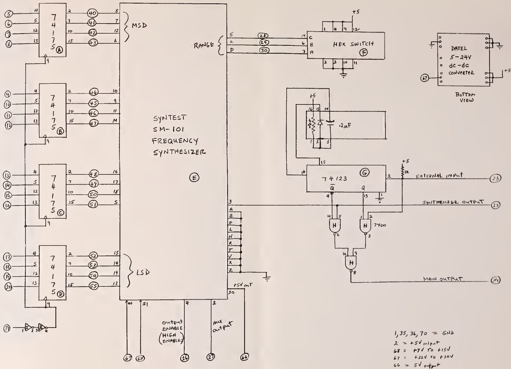
7.21 Freq. Synthesizer Circuit Dia. D3
