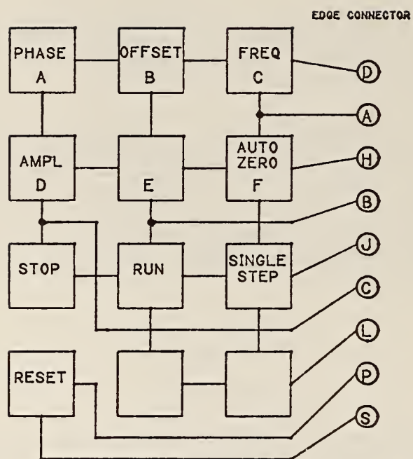
Figure 7.35 Function Keyboard
