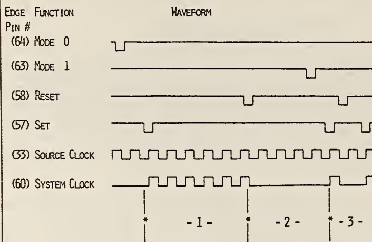
Figure 7.16 System Clock Control
