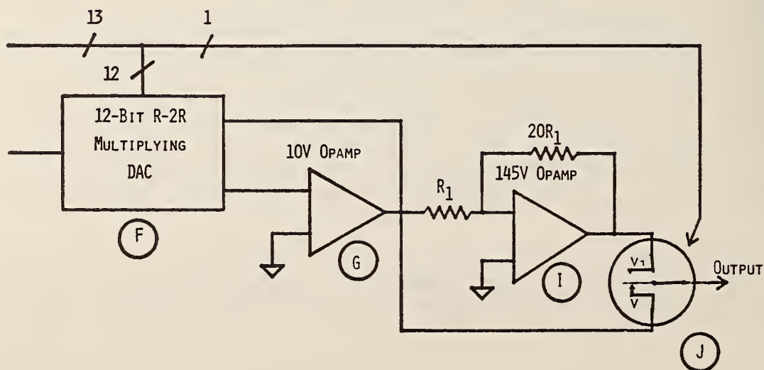
Figure 7.23 Block Diagram of Programmable Output Voltage Circuitry
