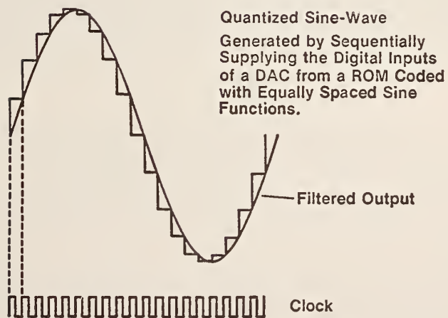
Figure 4.3 Stepped Sincwave
