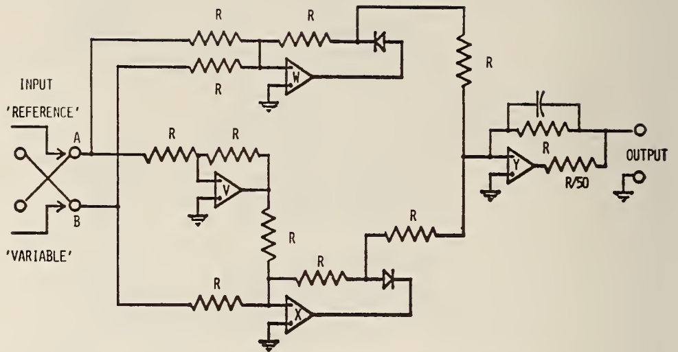
Figure 7.26 Phase Detector Circuit Schematic
