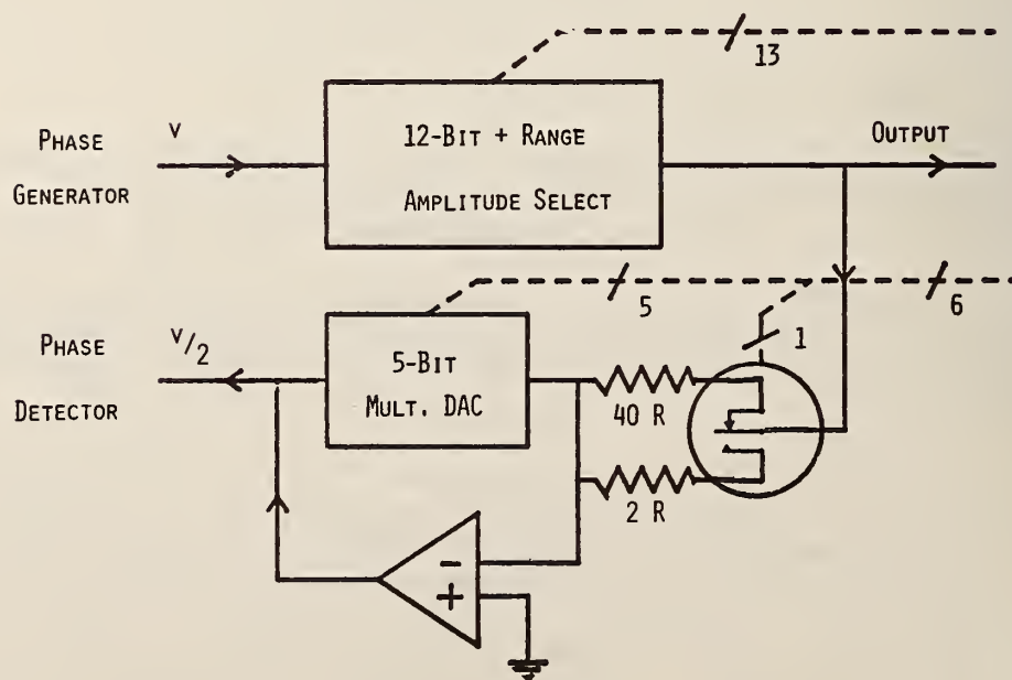
Figure 7.29 Phase Detector Scaling Stage
