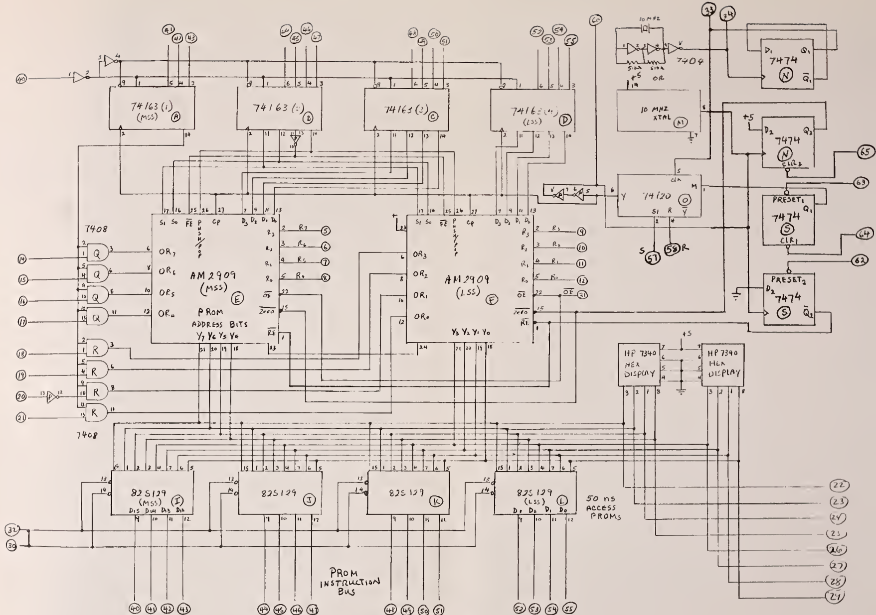
Fig. 7.15 Sequencer Circuit Diagram D9
