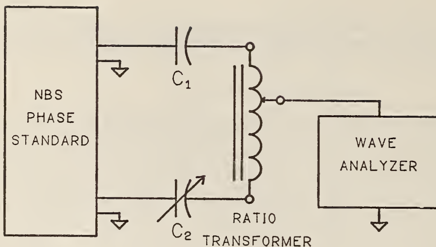
Figure 8.1 Test Circuit
