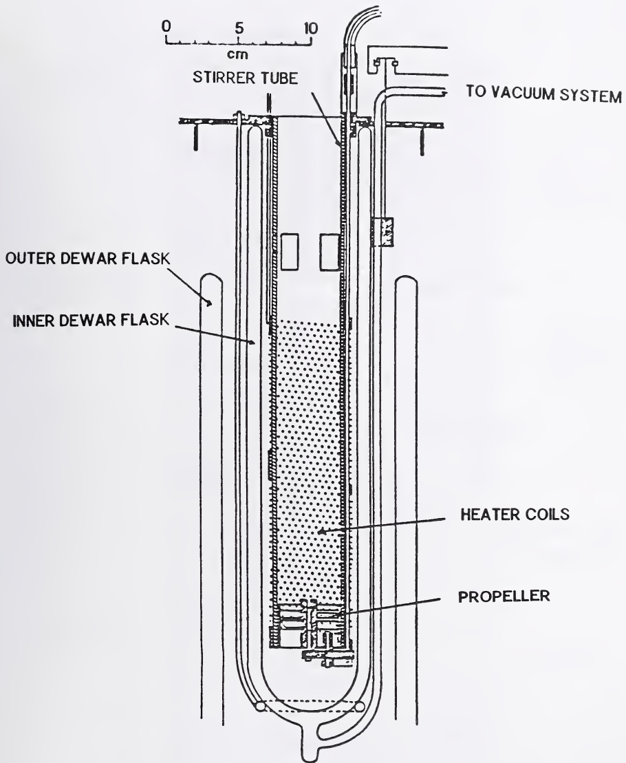
Figure 3.9. Cryostat.
