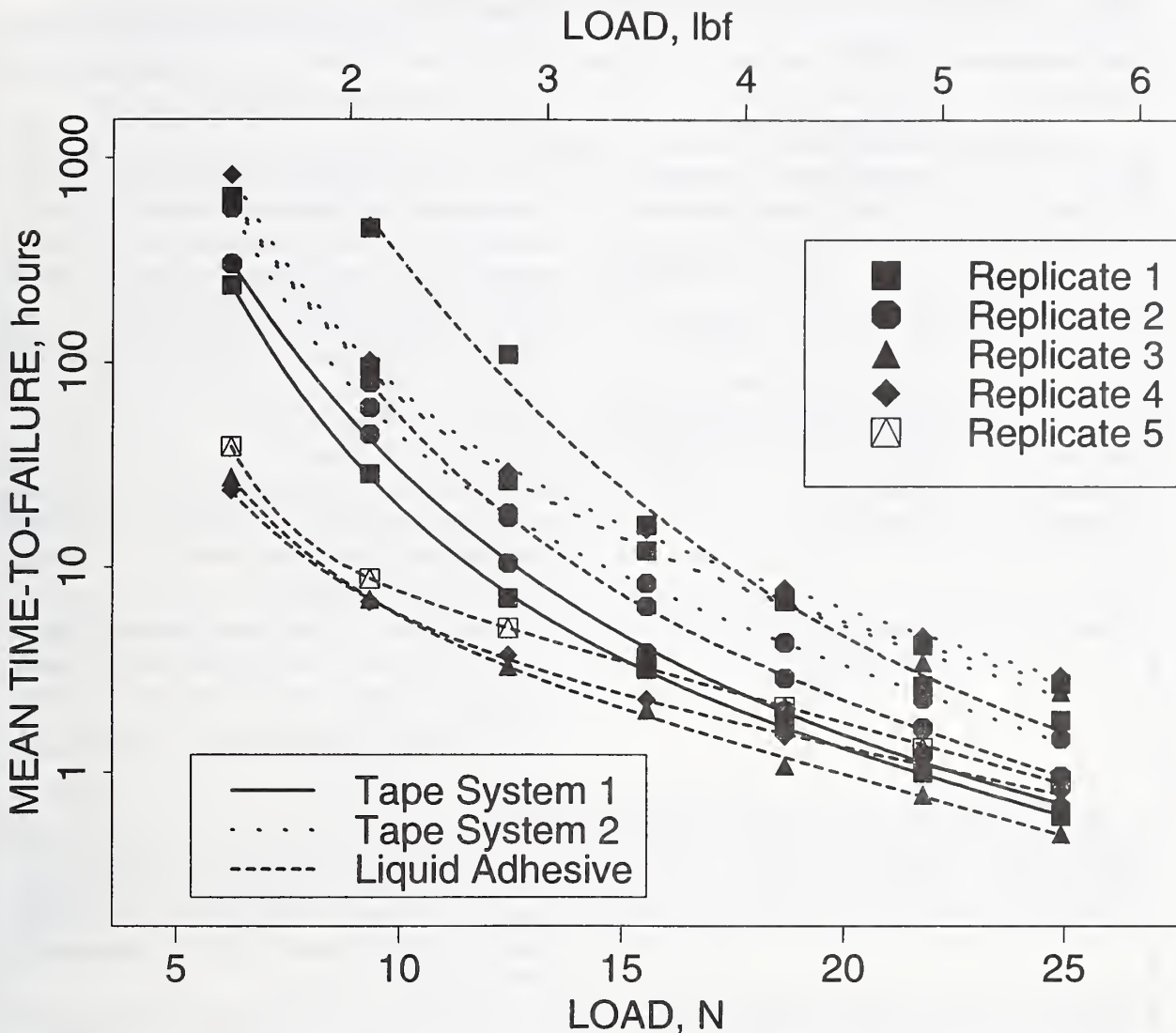
Figure 1. Mean Time-to-Failure Versus Load for the Tape-Bonded and Liquid-Adhesive-Bonded Specimens Investigated in Phase I [3].
