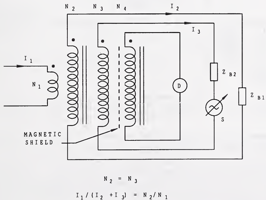
Figure 7. Compensated Current Comparator
