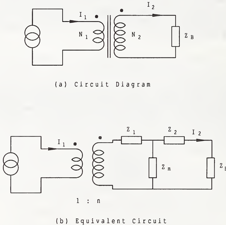
Figure 2. Current Transformer Connected to Source and Burden
