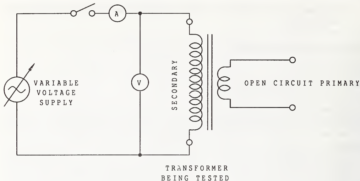
Figure 12. Demagnetization Circuit
