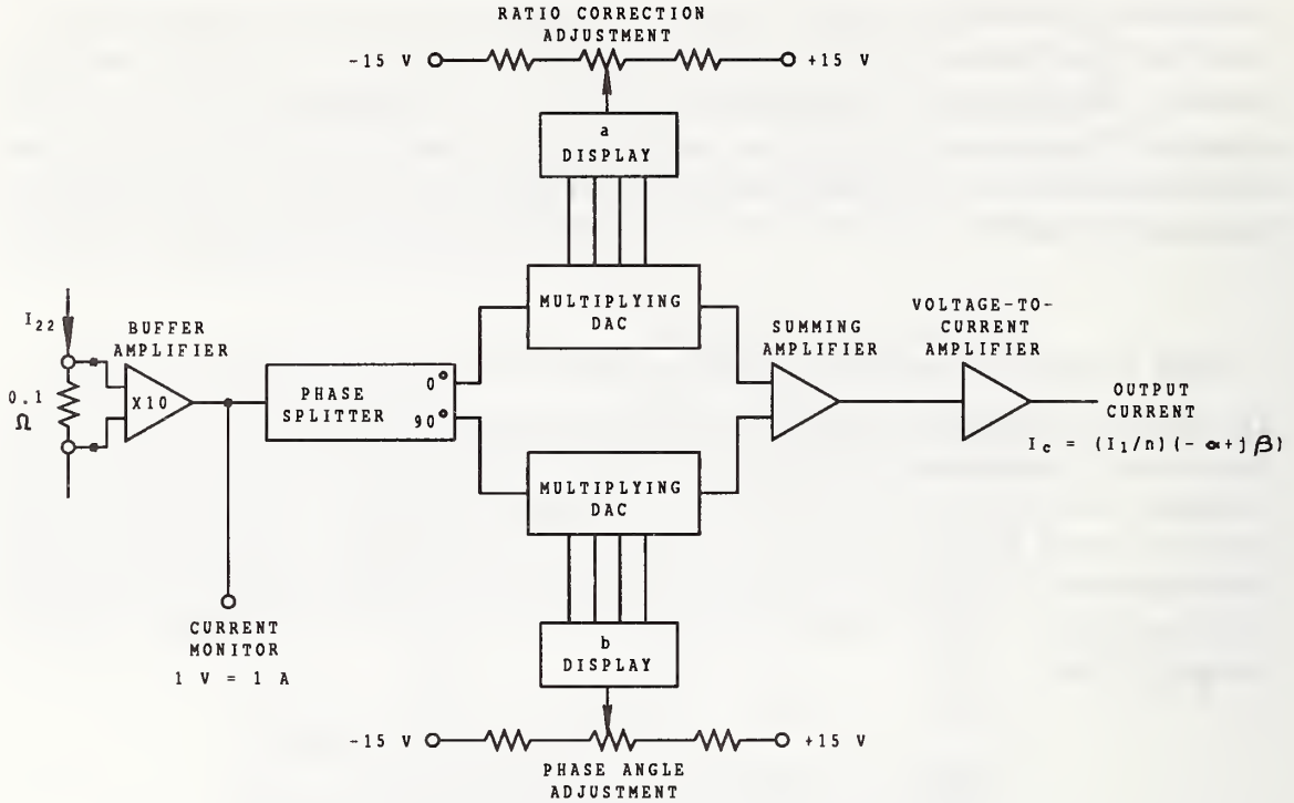
Figure 11. Test Set Used to Sense Secondary Current in the Current Comparator and to Generate a Correction Current
