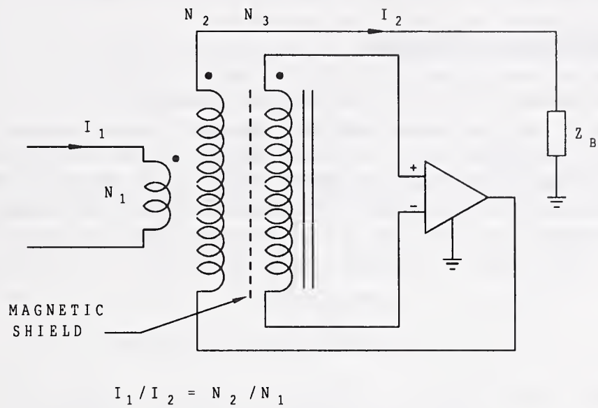
Figure 6. Amplifier-Aided Transformer
