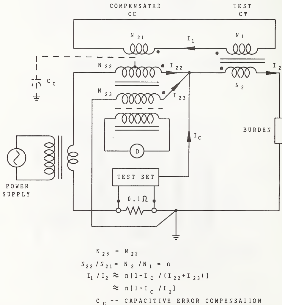
Figure 8. Current Transformer Calibration With a Compensated Current Comparator, Secondary Feed
