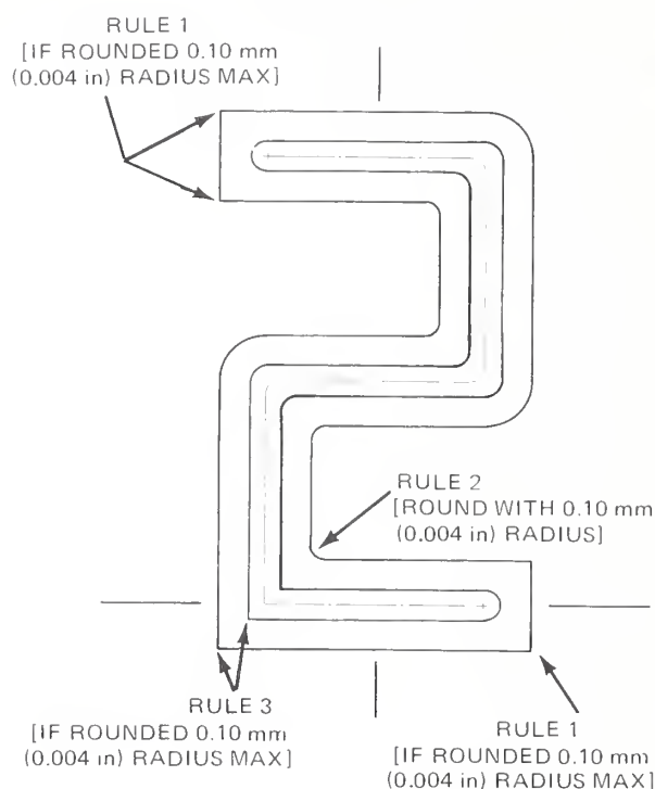
Figure 2 COL Gage
