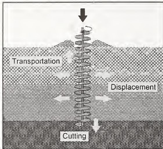
Figure 1 – CFA processes during the boring phase.
