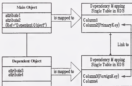
Fig. 3 Mapping XML Element objects with delegation (or dependency) relationship to RDB tables
