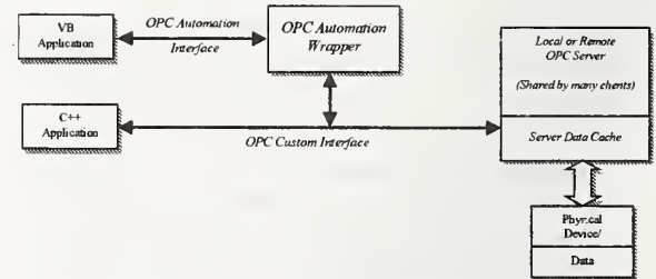
Figure 4. OPC Architecture
