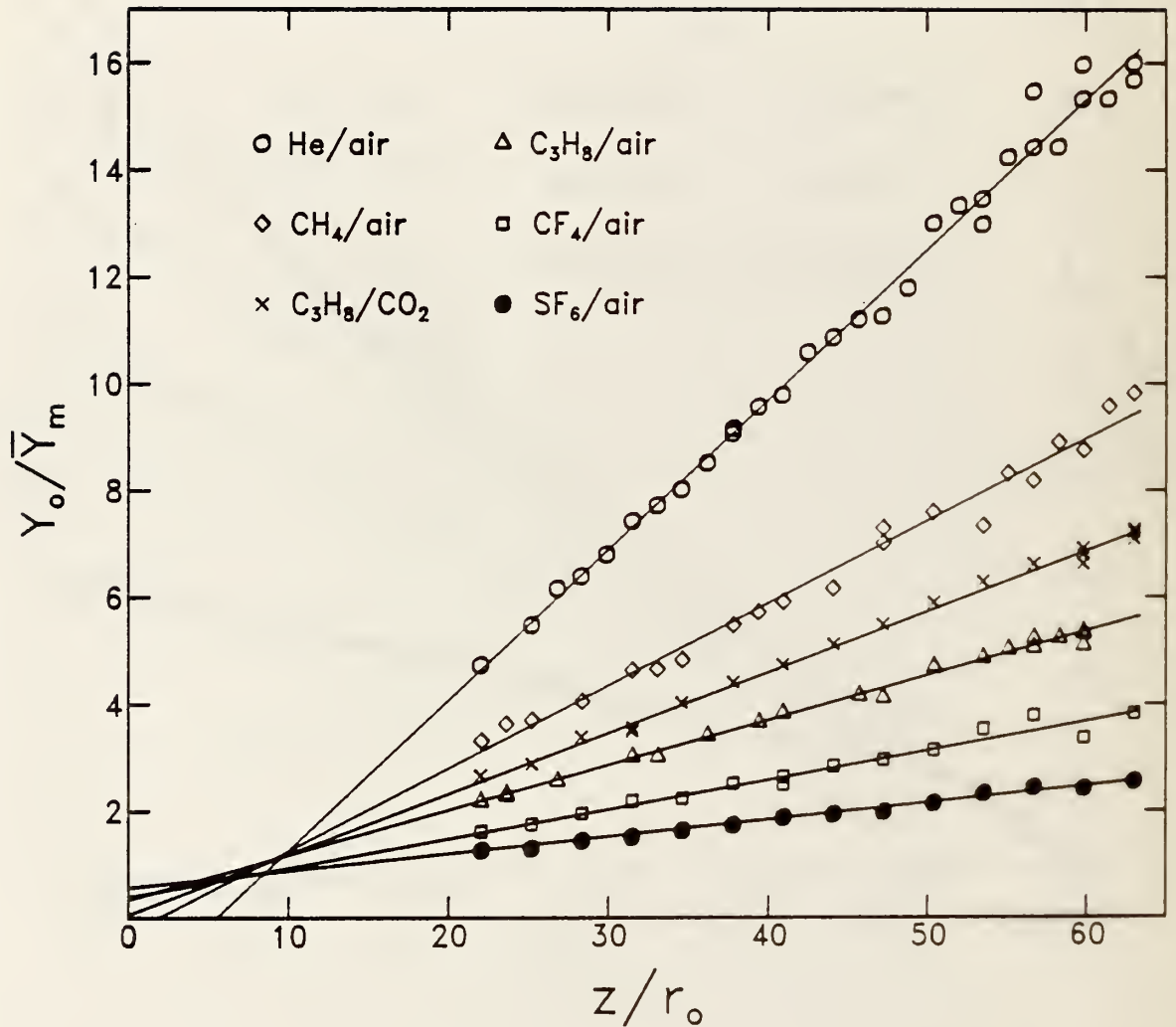
Figure 23. Values of the normalized centerline inverse mass fraction ( Y_o / \bar{Y}_m ) are plotted as functions of z/r_o for the six jet/coflow pairs listed. Straight lines are linear least squares curve fits of the data.
