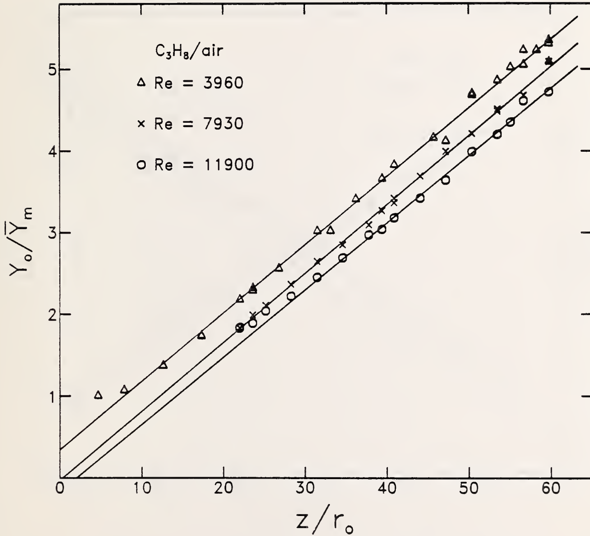
Figure 32. Y_o / \bar{Y}_m values are plotted against z / r_o for propane jets having the three different Reynolds numbers listed. The coflow gas is air. Straight lines represent linear least squares curve fits of the data.
