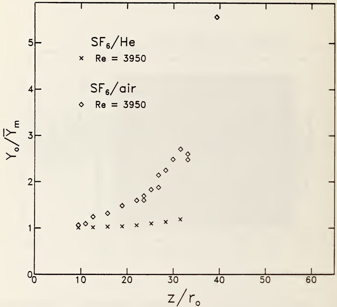
Figure 21. Values of Y_o/\bar{Y}_m as functions of z/r_o are shown for the SF_6 jet ( Re = 3950 ) flowing into coflows of air and helium.
