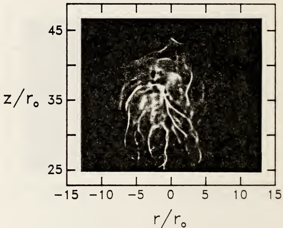
Figure 19. The fountain formed by the SF 6 jet (Re = 3950) entering into helium can be clearly seen in this shadowgraph recorded for downstream distances extending from z/r_0 = 25 to 47.
