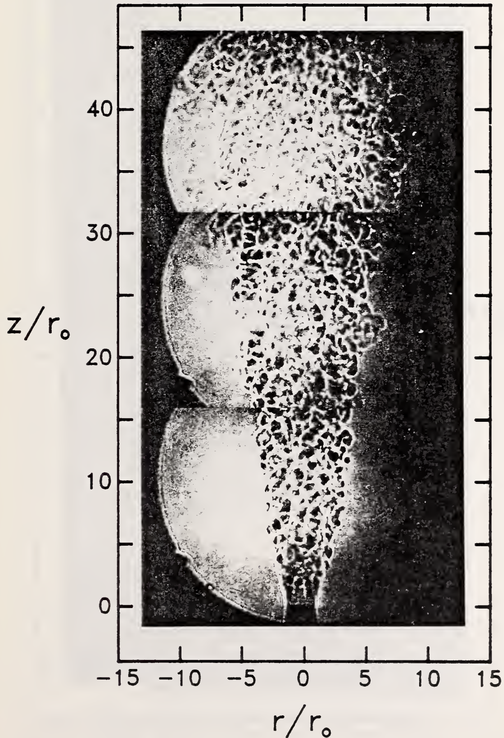
Figure 5. Superimposed shadowgraphs of the same helium jet visualized in fig. 5 are shown, but in this case, there is no coflow and the surroundings are the ambient air.
