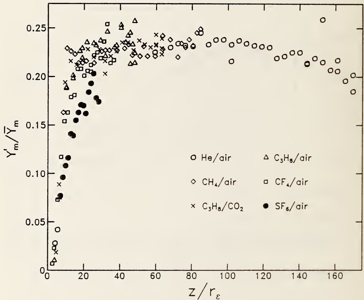
Figure 29. Mass fraction unmixedness values for the six jet/coflow gas combinations are plotted as functions of the downstream distance nondimensionalized by dividing by the effective radius. An excellent correlation of the data results.
