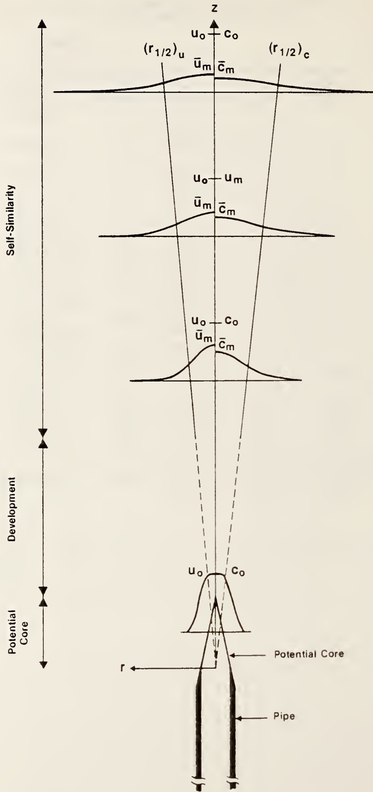
Figure 1. A schematic representation of the three flow regimes of an axisymmetric, constant-density, turbulent jet is shown. Representative radial profiles of velocity and jet fluid concentration are shown at one location in the potential core portion of the flow and at three positions in the self-similar regime.
