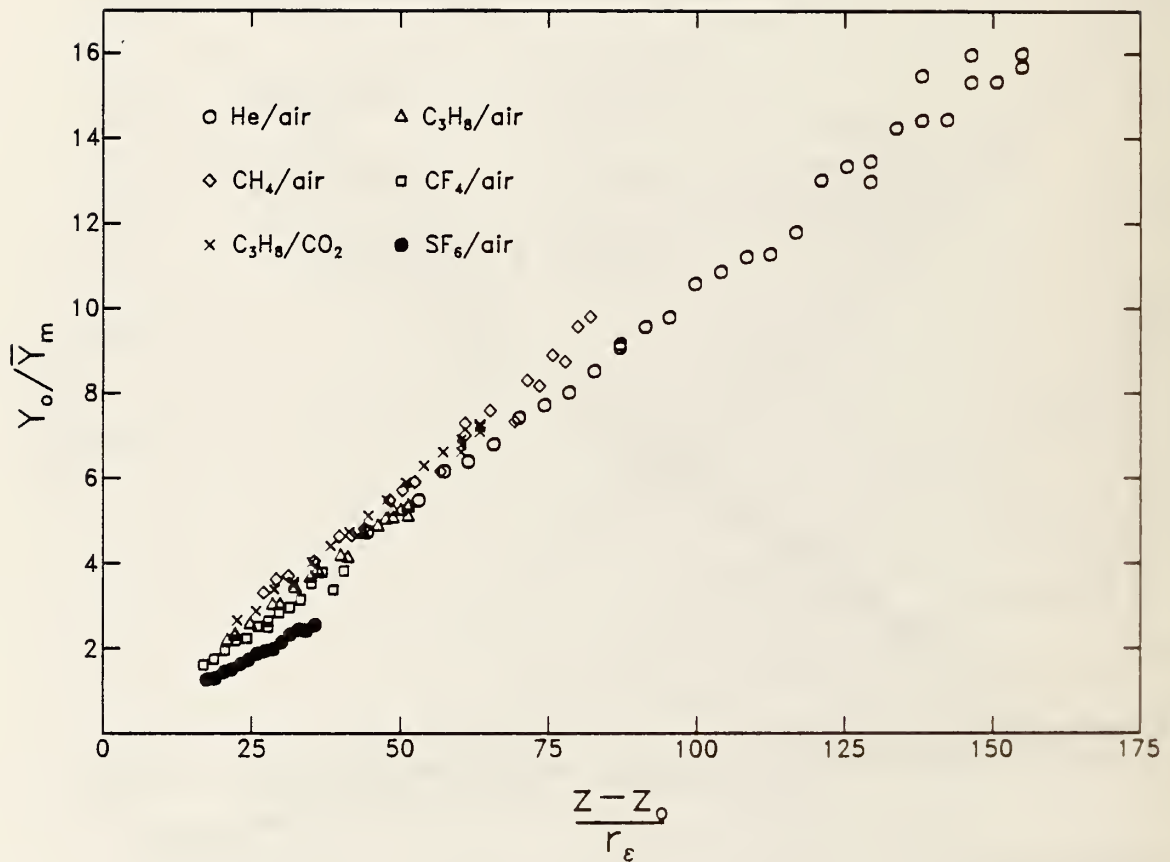
Figure 25. Experimental values of Y_o / \bar{Y}_m for the six jet/coflow combinations listed are plotted as functions of downstream distance normalized by the effective radius, r_\epsilon . Results have been offset by the appropriate values of virtual origin. Comparison with fig. 23 indicates that the use of the effective radius concept gives a partial correlation of the data.
