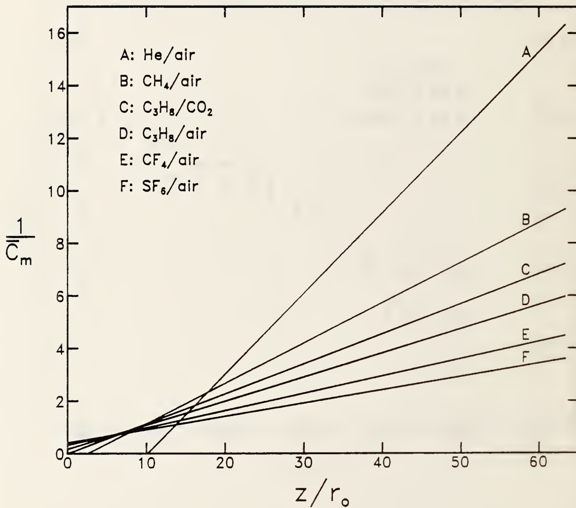
Figure 39. Values of 1/\bar{C}_m calculated using eq. (34) are plotted as functions of z/r_0 for the six gas pairs listed. These results are based on a method suggested by Thring and Newby [18].
