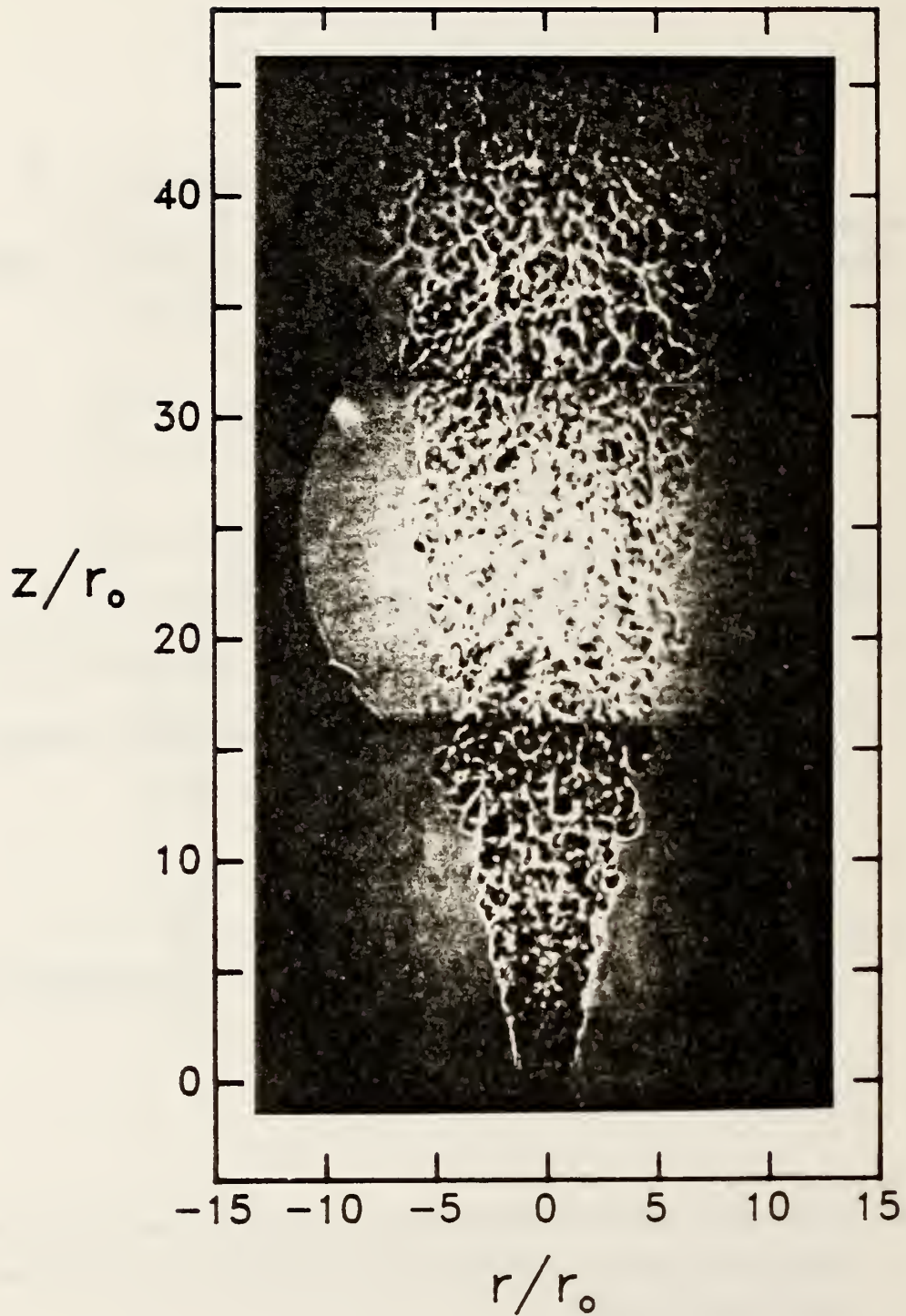
Figure 5. Three shadowgraphs of a turbulent helium jet flowing into a slow coflow of air are superimposed. The Reynolds number for the jet is 3950.
