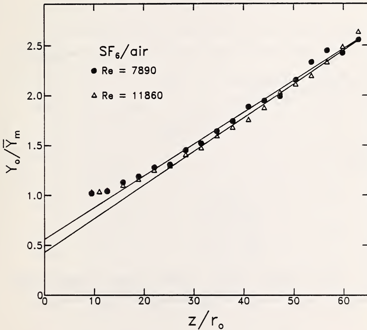
Figure 34. Values of Y_o/\bar{Y}_m for SF 6 jets at Reynolds numbers of 7890 and 11,860 are shown as functions of z/r_o . Straight lines represent the results of linear least squares curve fits of the data.
