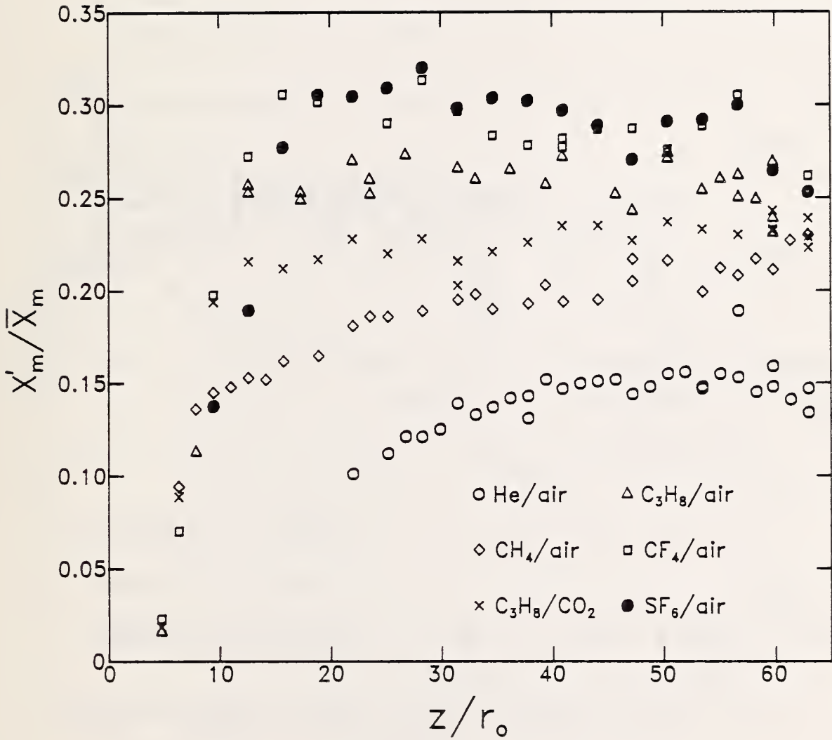
Figure 26. Experimental results of centerline unmixedness measurements in mole fraction terms ( X'_m / \bar{X}_m ) are plotted as functions of z/r_0 for the six jet/coflow pairs listed.
