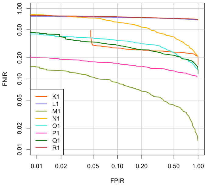
Figure 7: DET at rank 20 of all SDKs for four test cases
