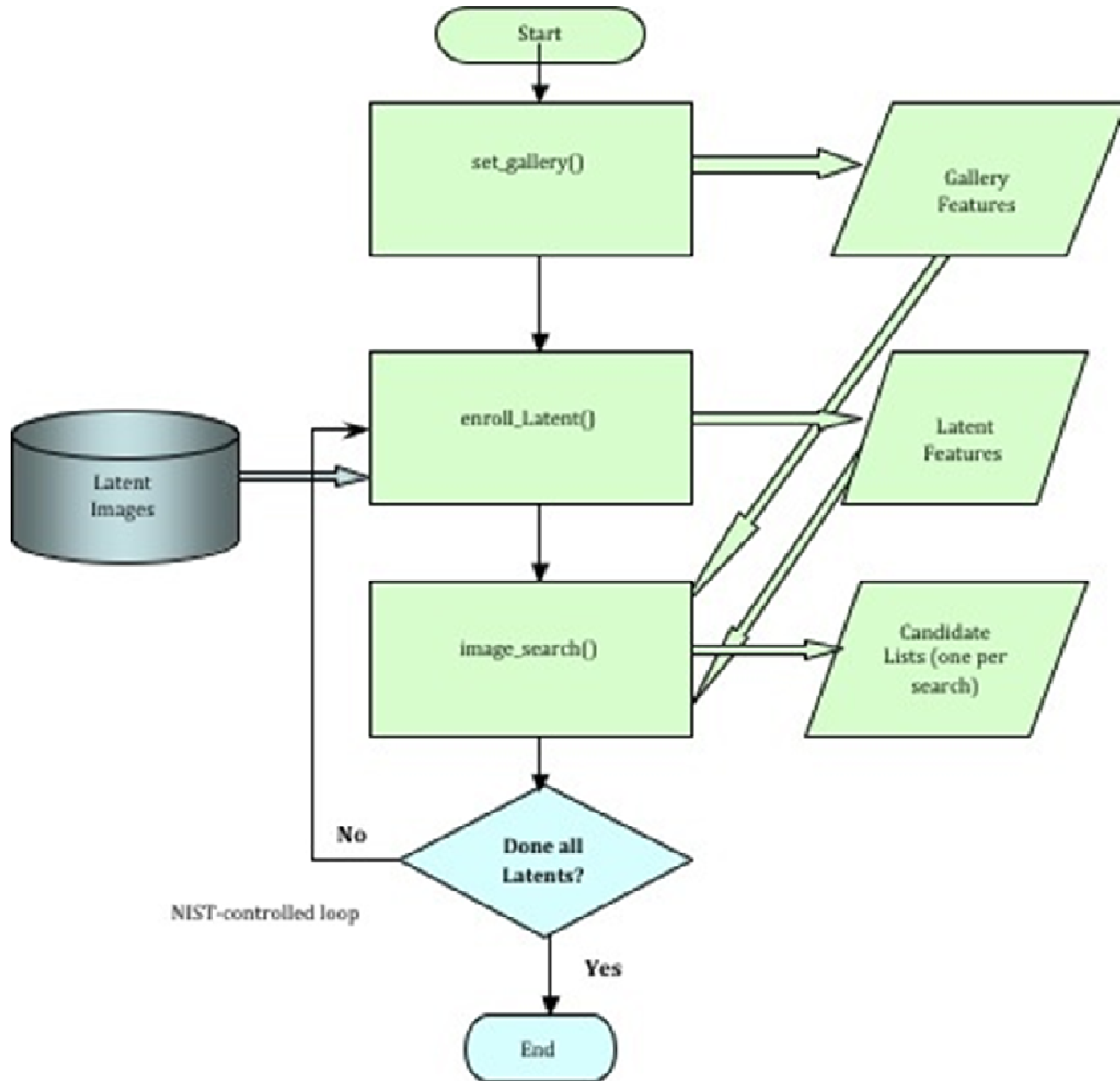
Figure B- 4: Stage 3 - Logic and data flow for Latent image search of Gallery using extracted features
