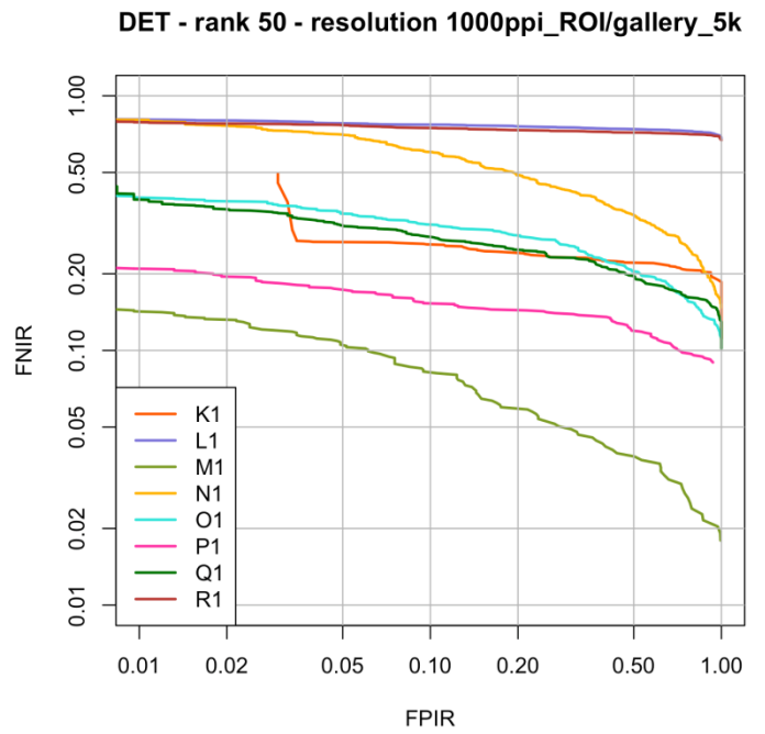
Figure 8: DET at rank 50 of all SDKs for four test cases
