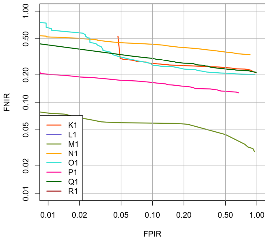
DET - using probability rank 1 - resolution 1000ppi/gallery_10k
