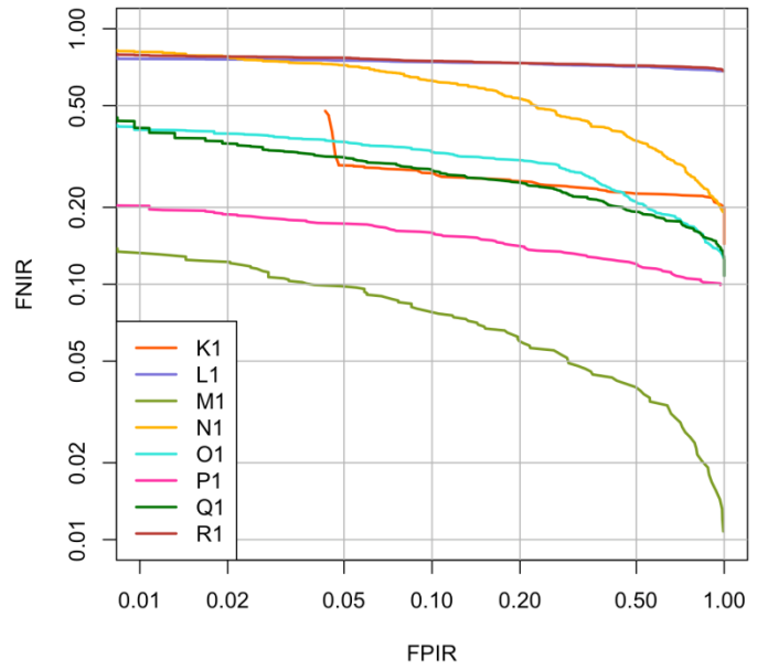
DET - rank 20 - resolution 1000ppi/gallery_5k
