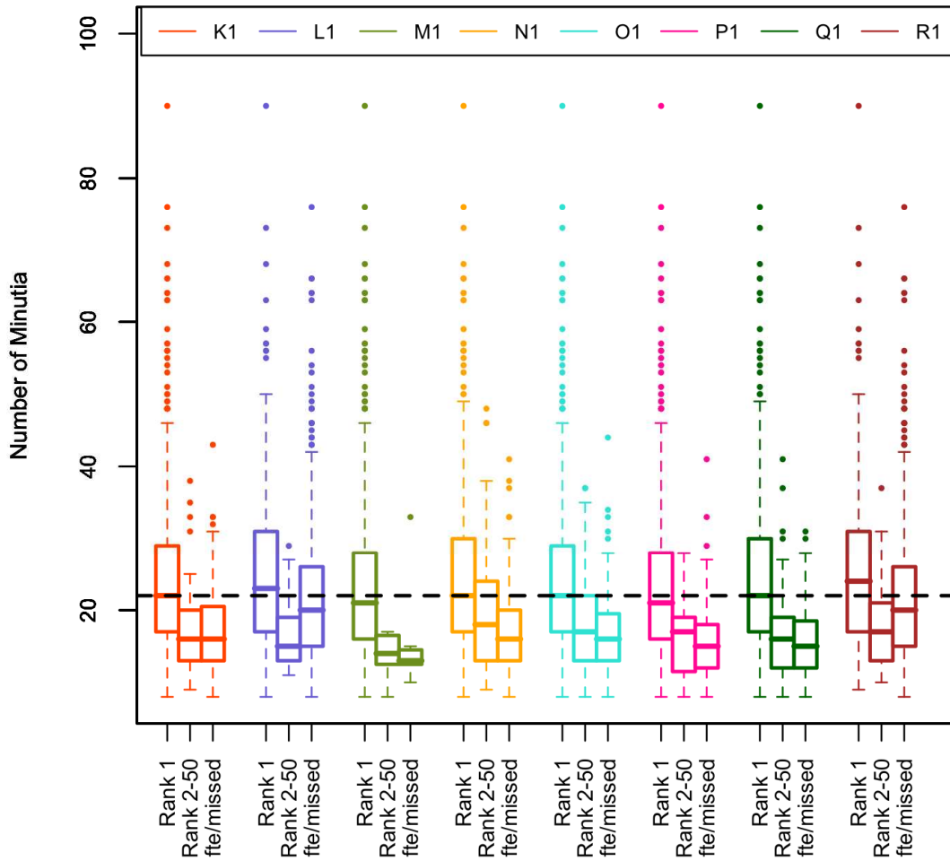
Figure 16: Box plot of minutia count vs. performance for latent resolution 1000 ppi and gallery size of 5k. (Minutia count was performed manually by fingerprint examiners.)
