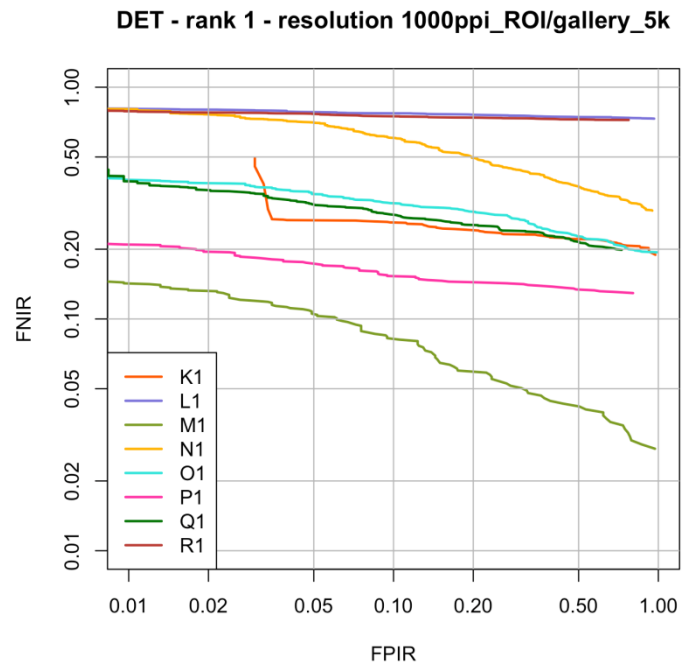
Figure 6: DET at rank 1 of all SDKs for four test cases
