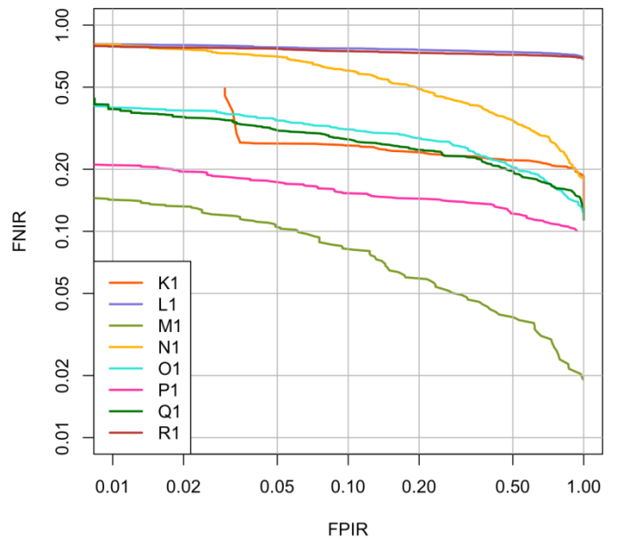
Figure 7: DET at rank 20 of all SDKs for four test cases
