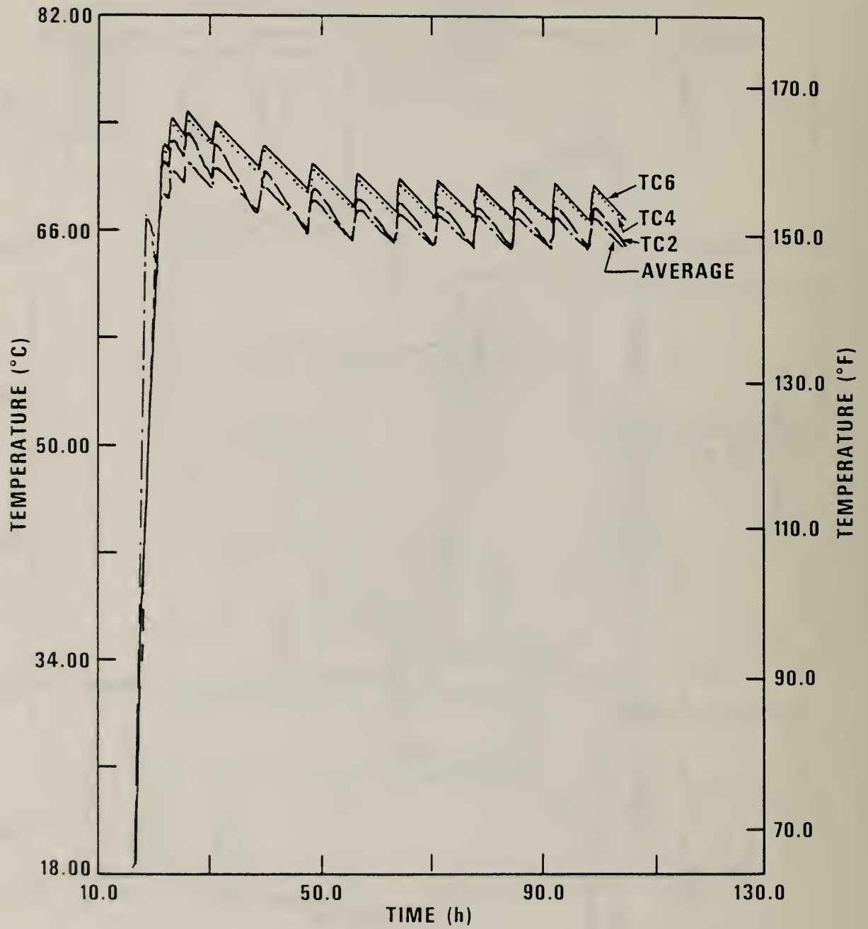
Figure 9. Typical Temperatures (TC2, TC4, TC6, and Water Average) vs Time for a Recovery and Standby Test.
