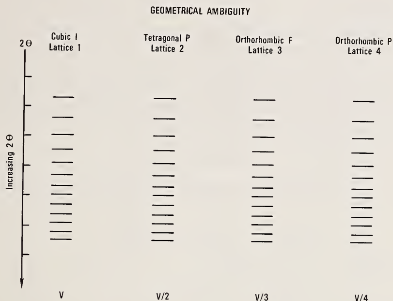
Figure 4. Total geometrical ambiguities. From any cubic I lattice, one can calculate a tetragonal P, an orthorhombic F and an orthorhombic P lattice all of which have exactly the same d-spacings (ref. [8]) as depicted schematically. The transformation matrices required to produce this four-fold ambiguity are:
