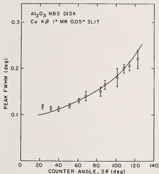
Figure 5a. Variation of FWHM of Al 2 O 3 diffraction peaks as a function of scattering angle 2\theta for the experimental conditions listed: x-rays, Cu K \beta .
