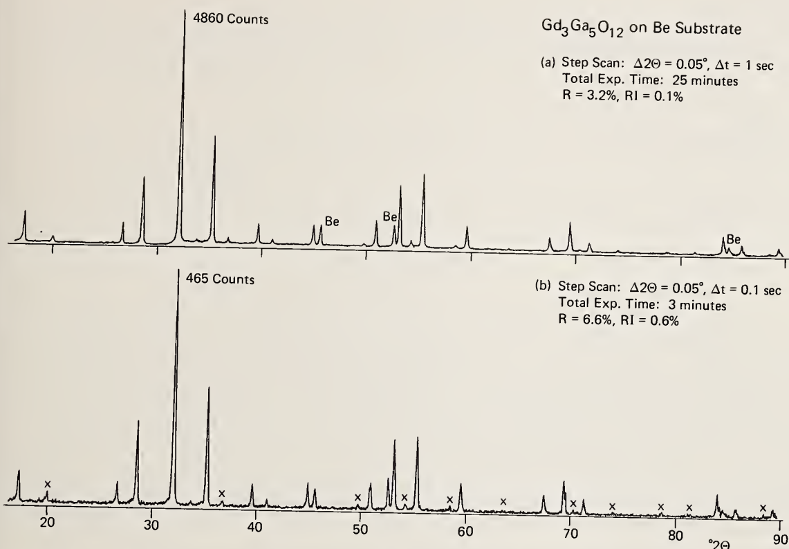
Figure 4. Transmission powder diffractometer patterns of garnet Gd 3 Ga 5 O 12 powder sample mounted on thin Be foil, CuK \alpha radiation. Eleven reflections marked x in (b) had peak intensities less than 3(B^{\frac{1}{2}}) and were dropped from the profile fitting calculations; average of 18 peaks 0.008^\circ(2\theta) and 0.8 peak intensities for 3 minute recording time.
