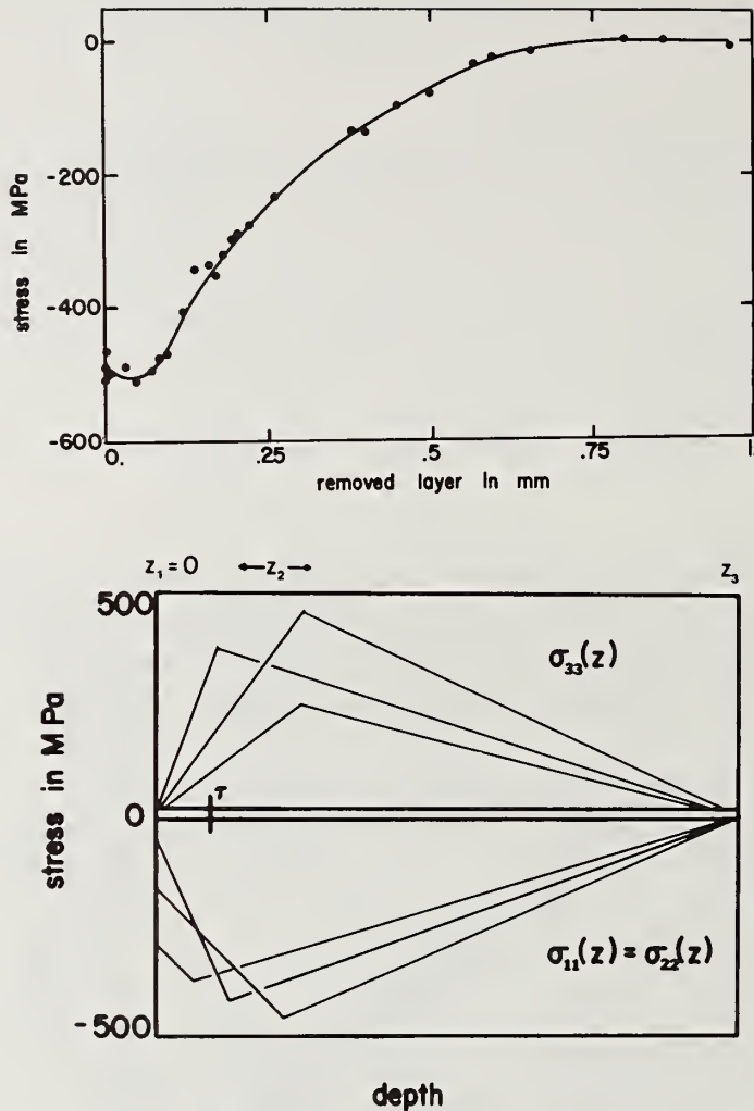
Figure 10. (a) The gradient measured by layer removal for one of the specimens in figure 9. (Etchant: 100 parts 30 pct H_2O , 10 parts 48 pct HF). Data uncorrected for layer removal and depth of penetration. 310 peak, CoK_{\alpha} radiation. (b) Assumed gradients for calculations described in text to fit data in (a).
