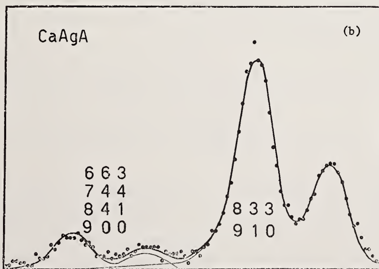
Figure 3. Selected peaks of a dehydrated CaAgA zeolite powder ( \text{Pm}3\text{m} , \alpha_0 = 12.34 \text{ \AA} ) fitted with the silicon \alpha_1 standard derived from the Silicon 220 peak: (a) 210 peak ( 2\theta \approx 16^\circ ), counting time per step: 18 s, (b) 663, 744, 841, 900 and 833, 910 diffracted peaks, counting time per step: 18 s, 2\theta \approx 68.5^\circ .
