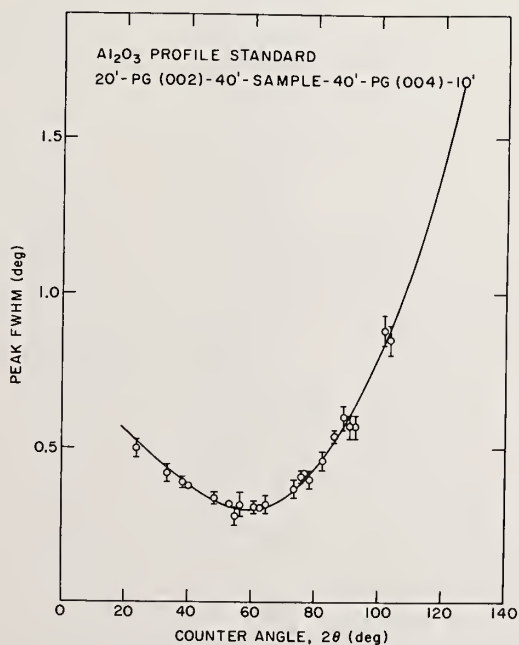
Figure 5b. Variation of FWHM of Al 2 O 3 diffraction peaks as a function of scattering angle 2\theta for the experimental conditions listed: neutrons, \lambda = 1.424 \text{ \AA} .
