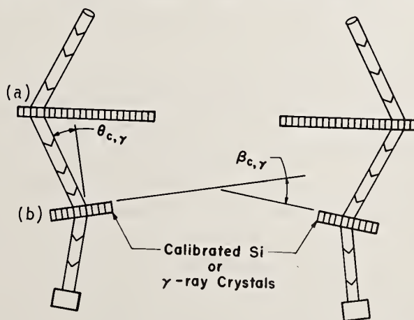
Figure 4. Quasi-non-dispersive arrangement for transfer of crystal calibration.
