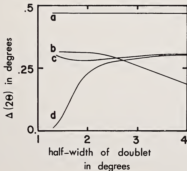
Figure 13. Calculated peak shift due to \text{K}_{\alpha_1} - \alpha_2 doublet for various definitions of the peak. (a) Special slits to symmetrize peak (Wolfstieg, U., Die Symmetrisierung unsymmetrischer Interferenzlinien mit Hilfe von, Spezial Henden, Härtereitechn. Mit. 31, 23-26 (1978)). (b) Center of gravity. (c) Middle of half-width. (d) Parabolic fit to top 15 pct. The same Gaussian functions were assumed for the \alpha_1 , \alpha_2 components. 211 reflection, \text{CrK}_\alpha radiation.
