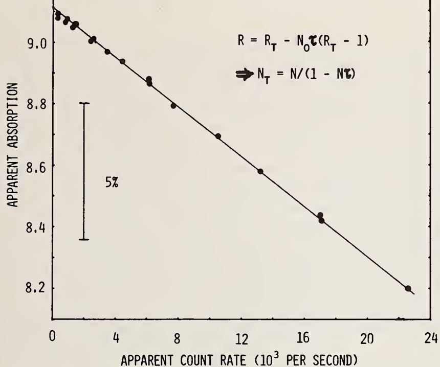
Figure 1. A typical plot of observed count rate vs number of absorbers placed in the beam.
