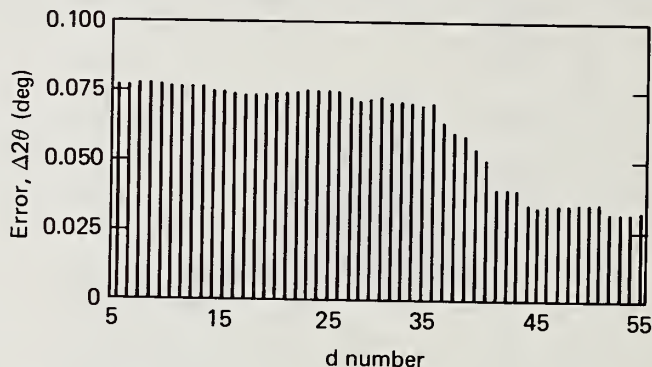
Figure 4. The effect of the 40-line PDF card format on the quality of data reported (PDF cubic patterns). Authors who measure more accurate data are more likely to continue their listing on to a second card.
