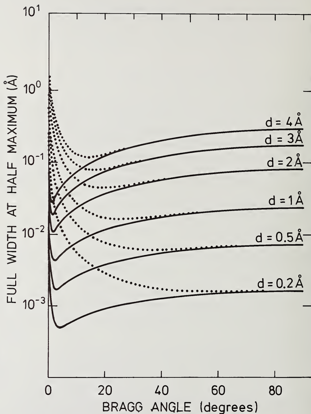
Figure 7. The dependence of \delta d_{\text{FWHM}} (the FWHM of a diffraction peak measured in the interplanar spacing scale) on the Bragg angle \theta_0 for \Delta\theta_0 = 10^{-4} rad (full lines) and \Delta\theta_0 = 5 \cdot 10^{-3} rad (dotted lines) for different interplanar spacings d using a germanium detector with a resolution of 150 eV and 485 eV at 5.9 keV and 122 keV, respectively [53].
