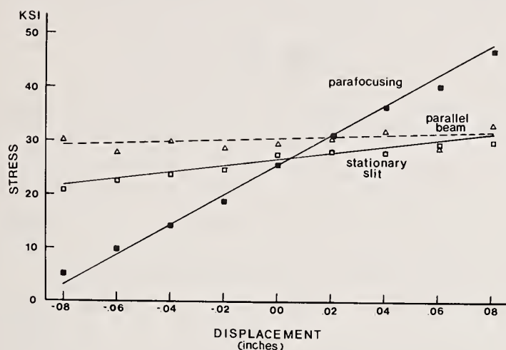
Figure 12. Measured effects of sample displacement, for various focussing techniques employed in stress measurements. Normalized 1045 steel, 211 reflection, \text{CrK}_\alpha radiation.
