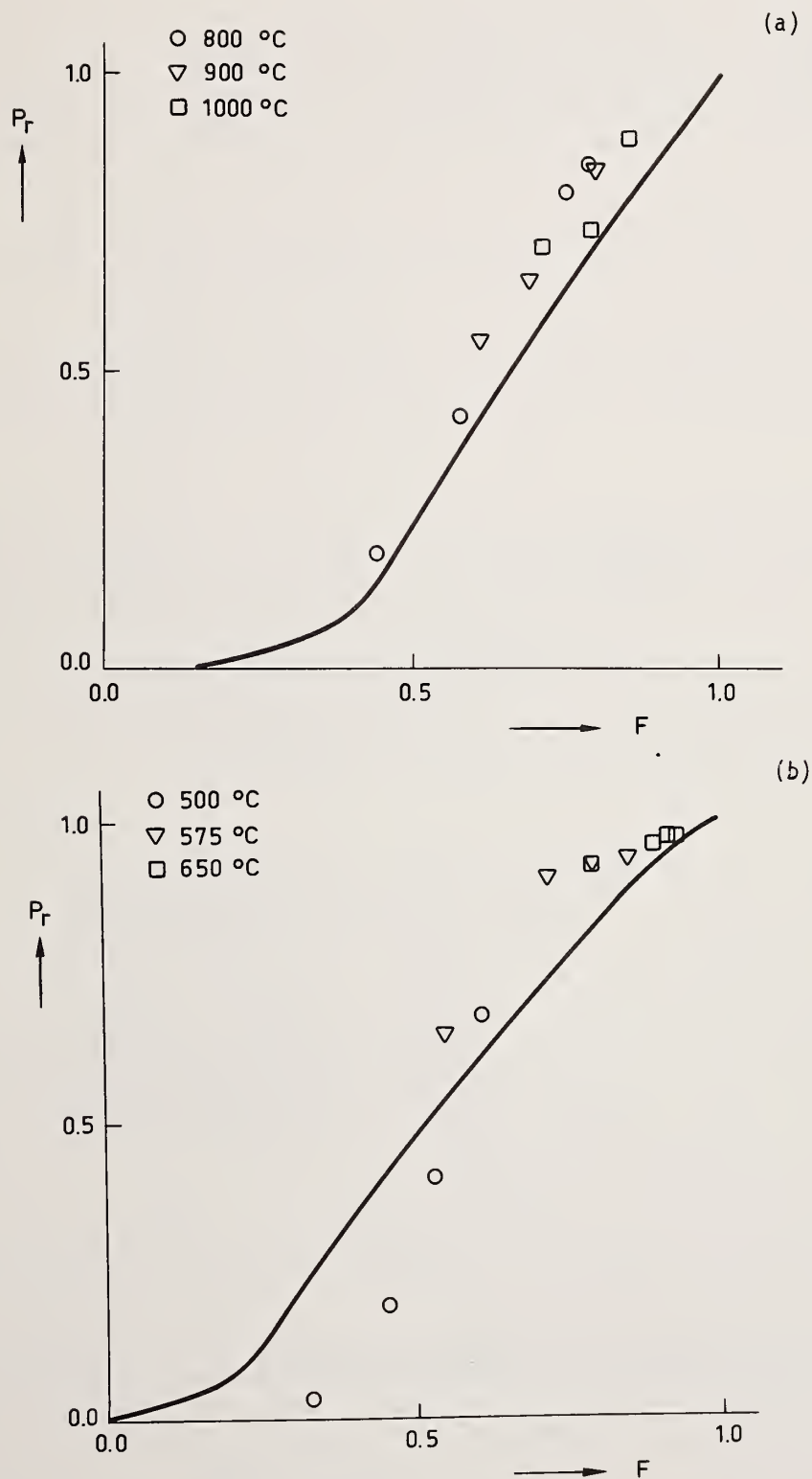
Figure 12. The relative peak position p_r as a function of the degree of interdiffusion F according to the concentric sphere model for Cu/Ni (a) and RbCl/KCl (b) powder blends. The experimental data points are also shown.
