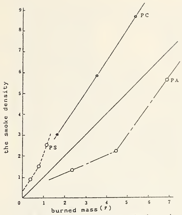
Fig. 2 Relationship between the burned mass and the smoke density.
