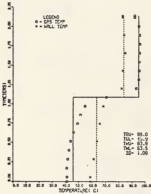
Figure 4. Typical room temperature profiles
