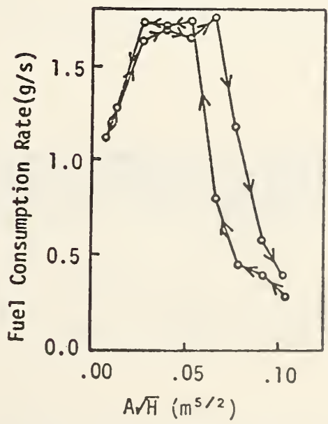
Figure 8 Hysteresis of Fuel Consumption Rate to Opening Factor(0.20m Tray)
