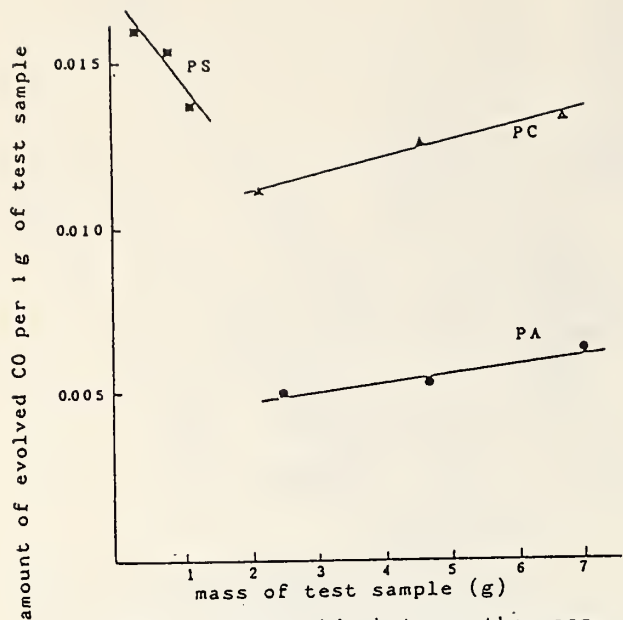
Fig. 5 Relationship between the mass of test sample and the amount of evolved CO per 1g of test sample.
