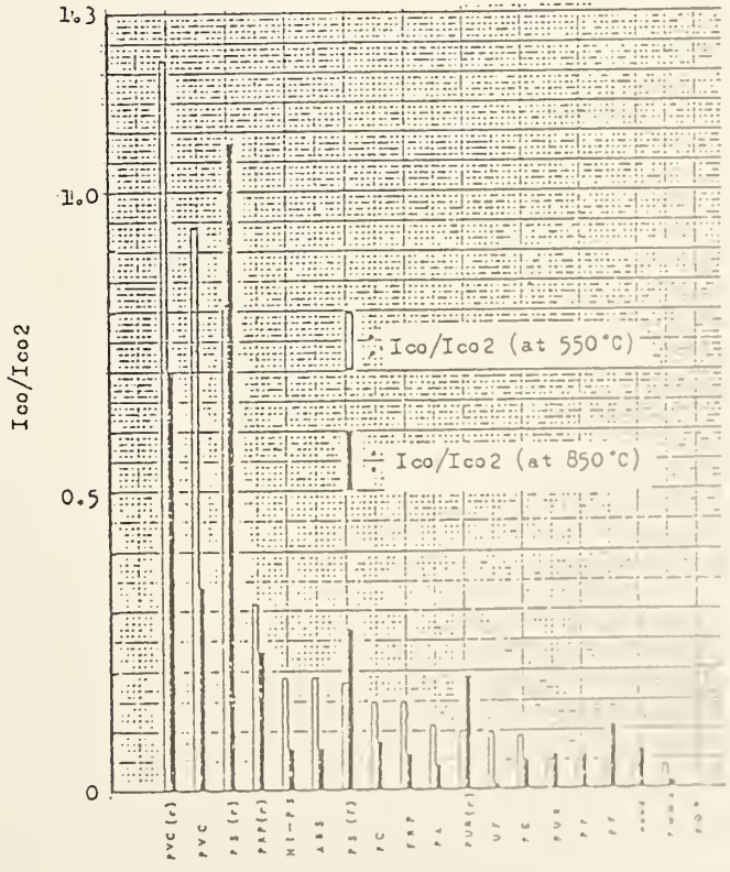
Fig. 11 Ico/Ico2 (at 550°C and 850°C).
