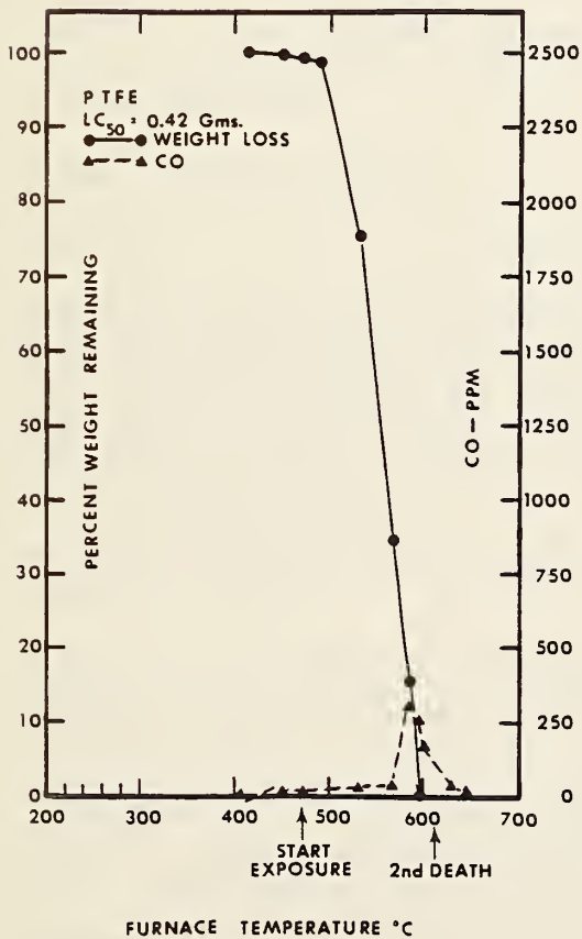
Figures 5 and 6: Decomposition pattern of polytetrafluoroethylene (PTFE) and polystyrene foam with evolution of carbon monoxide. Arrow at second death indicates the temperature at which the second of four exposed animals died (50% lethality).
