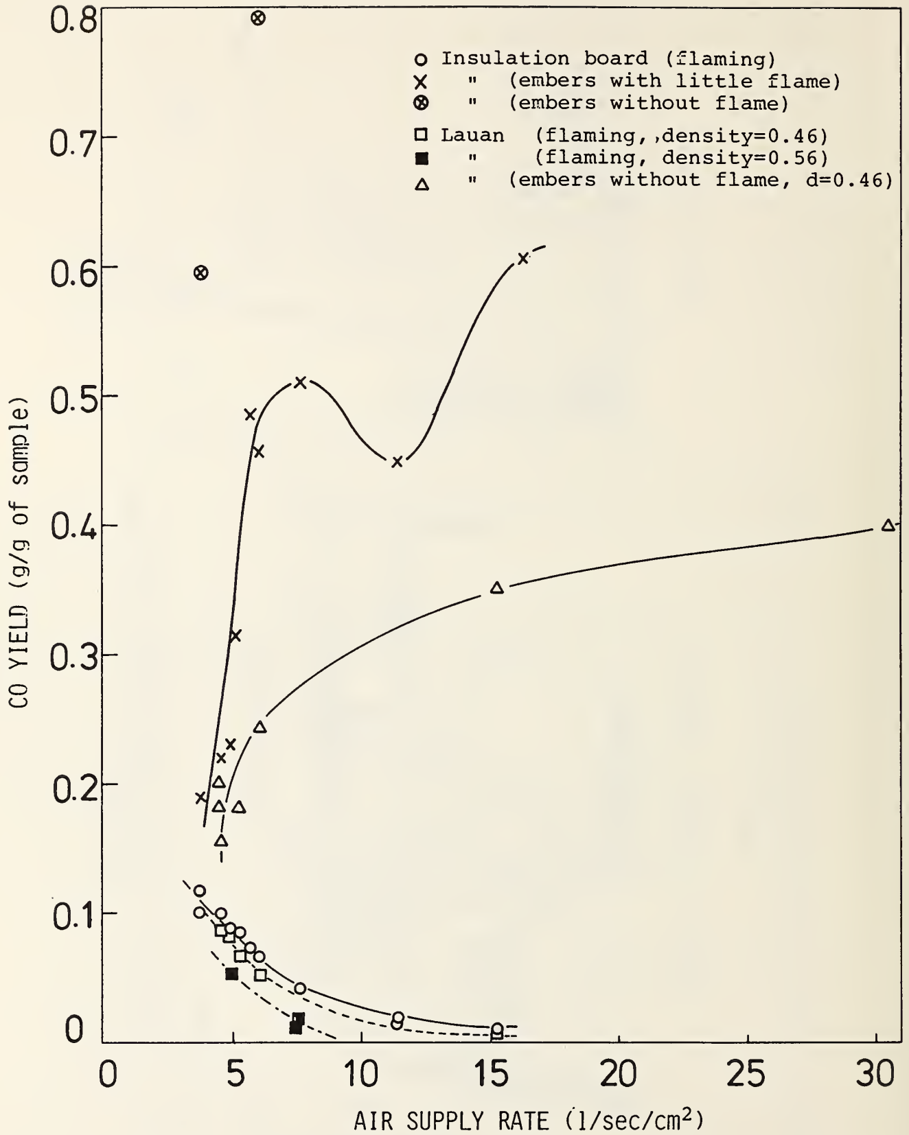
Figure 9. Relationship between CO yield and air supply rate
