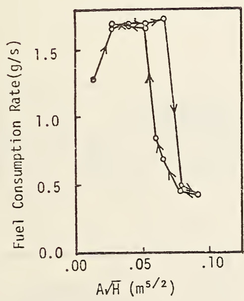
Figure 8 Hysteresis of Fuel Consumption Rate to Opening Factor(0.20m Tray)
