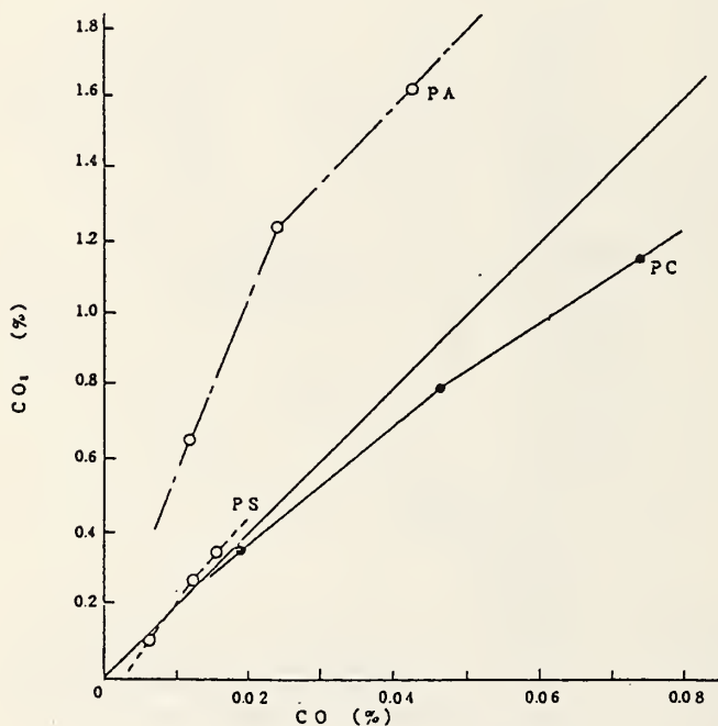
Fig. 7 Relationship between CO and CO_2 .
