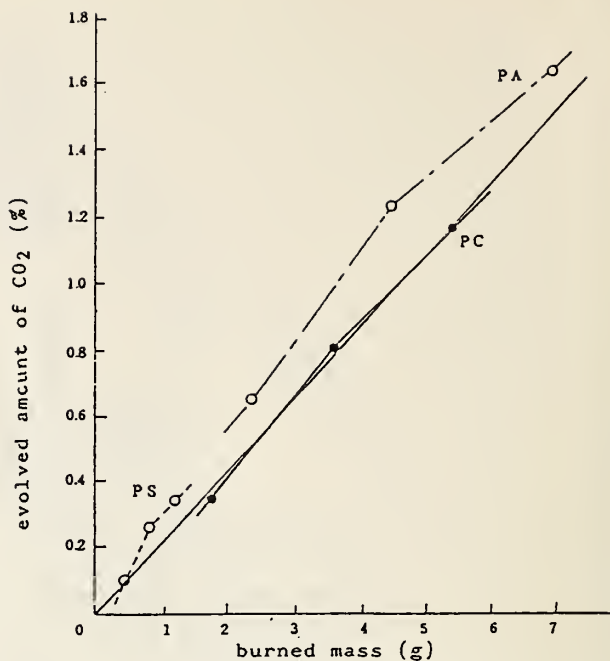
Fig. 6 Relationship between the burned mass and evolved amount of CO_2 .
