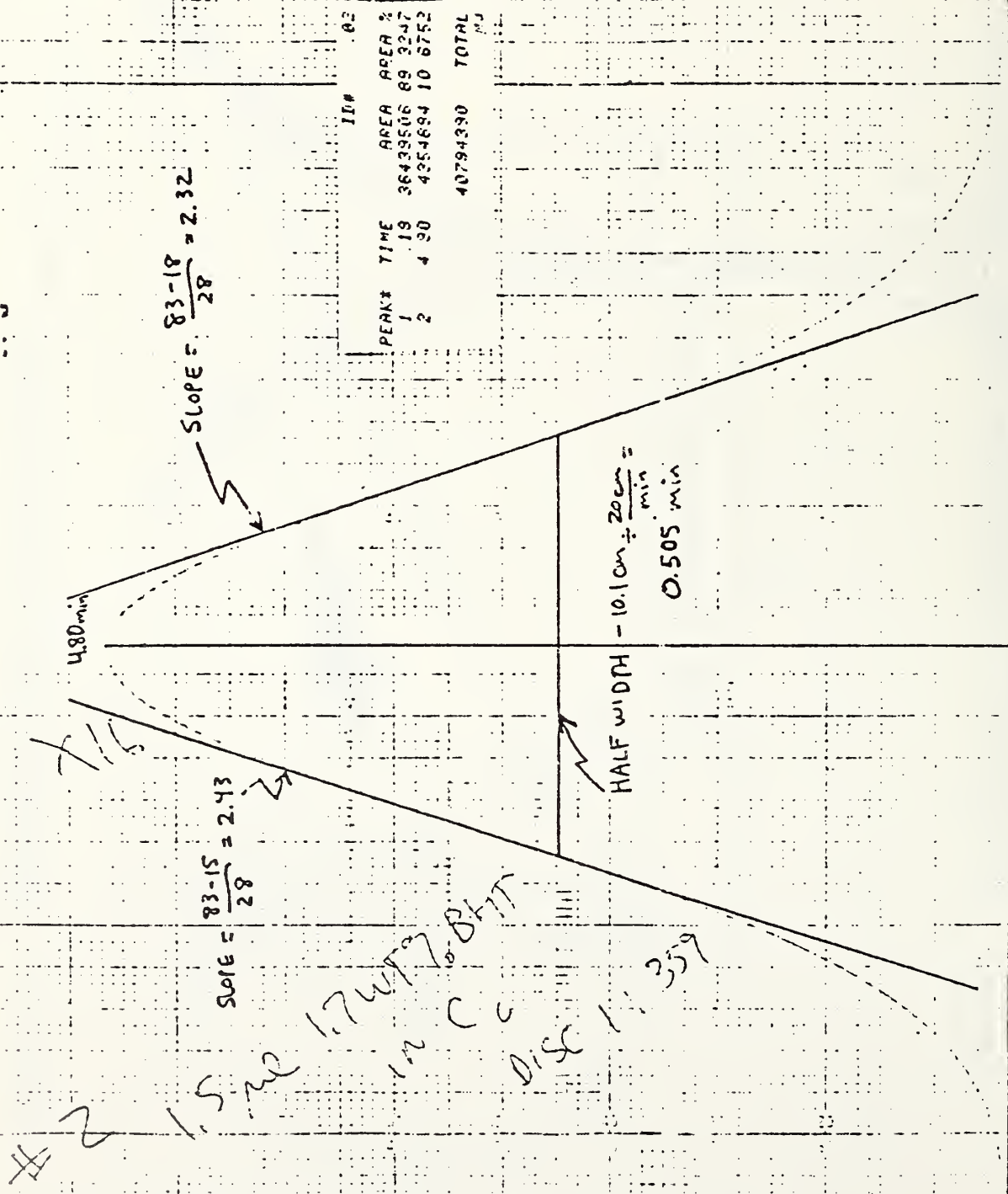
Figure VI-4: Typical strip chart recorder output of a probe peak showing the methods for determining the width at half maximum and tangent slopes.
