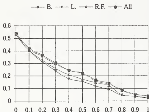
Figure 1: Recall/Precision curves
